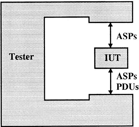
Figure 6 - Conceptual testing architecture
