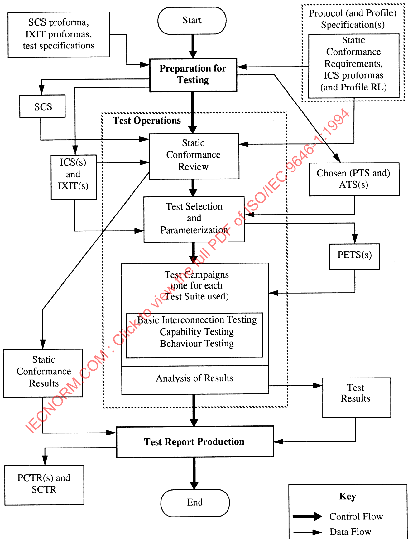
Figure 1 - Conformance assessment process overview
