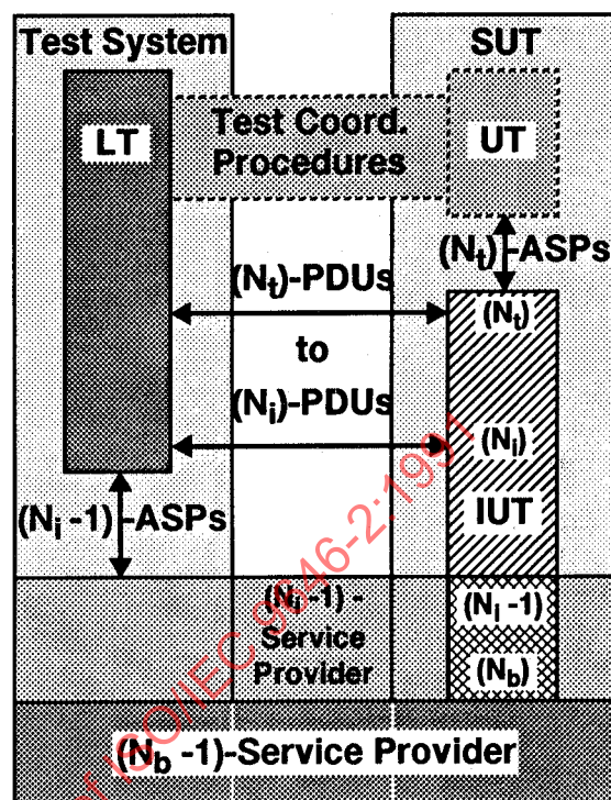
Figure 10 - Example of the DSE test method: testing the ( N_i )-protocol in an ( N_b ) to ( N_i )-protocol IUT
