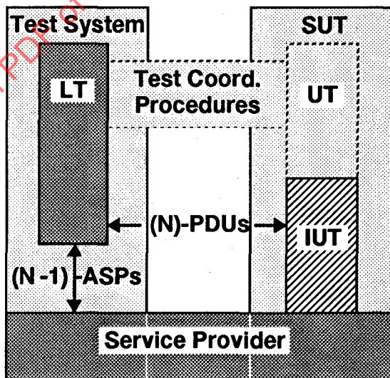
Figure 8 - The RS test method
