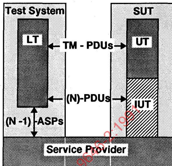
Figure 7 - The CS test method
