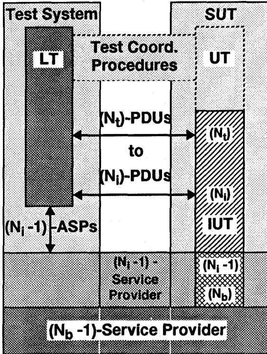
Figure 12 - Example of the RSE test method: testing the (N_i) -protocol in an (N_b) to (N_i) -protocol IUT
