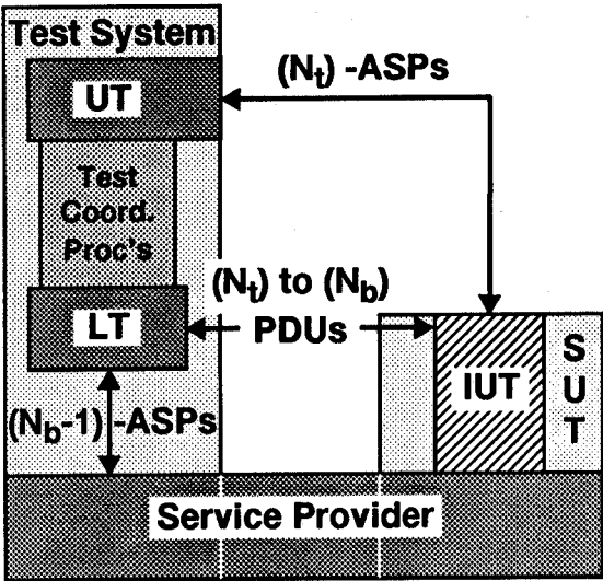
Figure 1 - The Local test method
