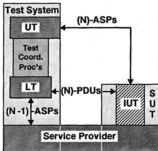
Figure 5 - The LS test method
