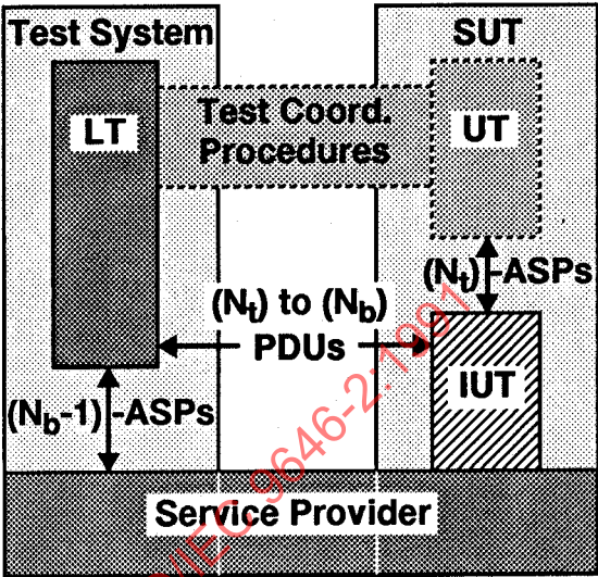
Figure 2 - The Distributed test method
