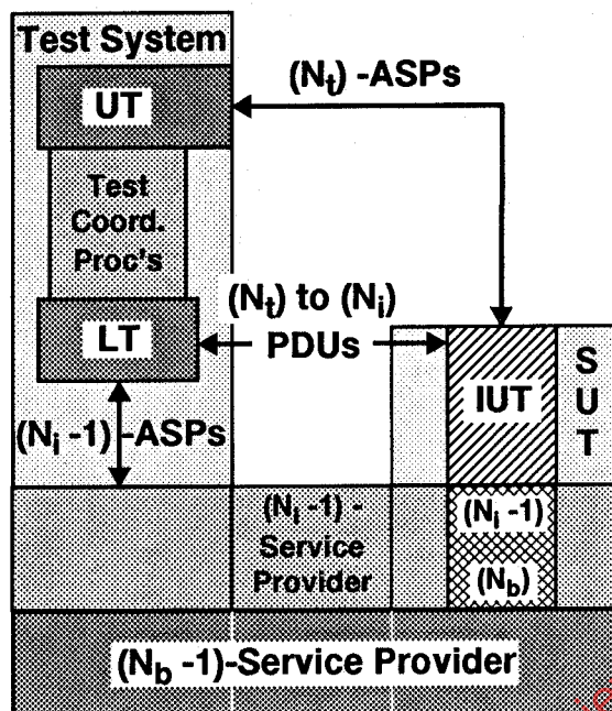
Figure 9 - Example of the LSE test method: testing the ( N_i )-protocol in an ( N_b ) to ( N_i )-protocol IUT
