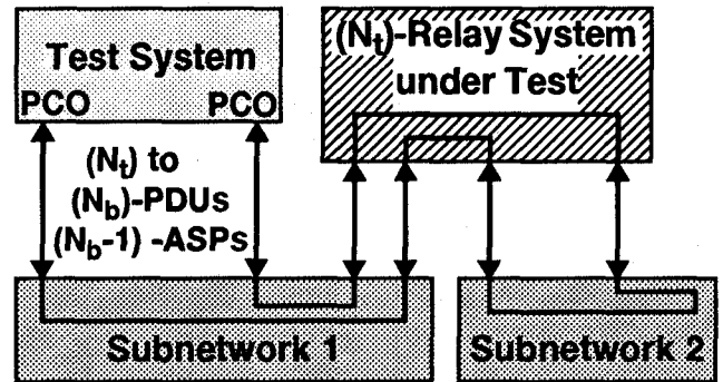
Figure 13 - Loop-back test method (YL)
