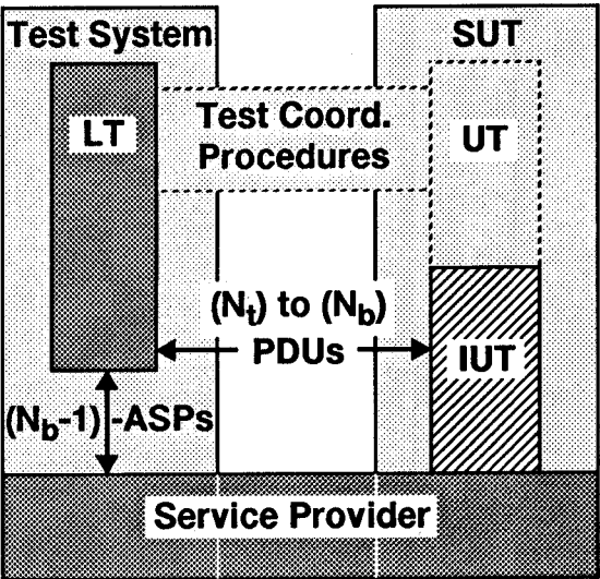
Figure 4 - The Remote test method
