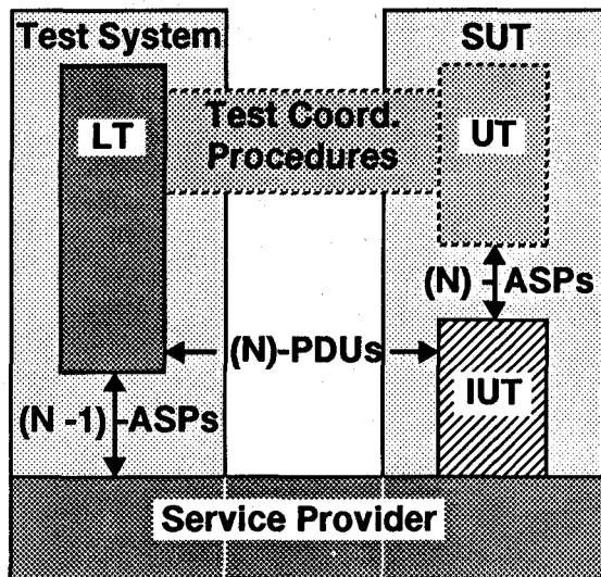
Figure 6 - The DS test method
