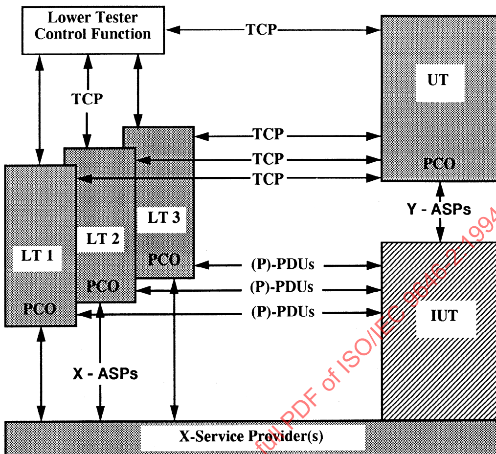
Figure 7 - Multi-Party Testing with a single UT
