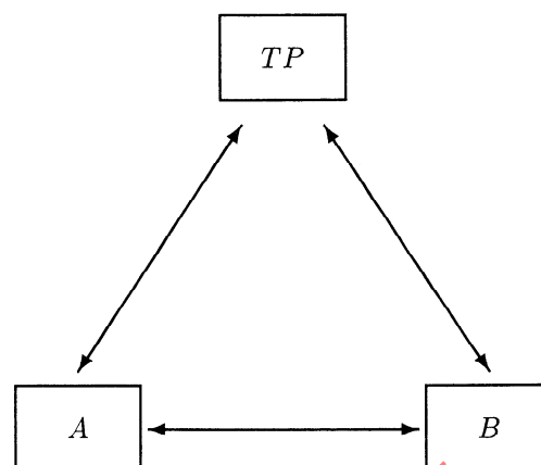
Figure 1 – Authentication model
