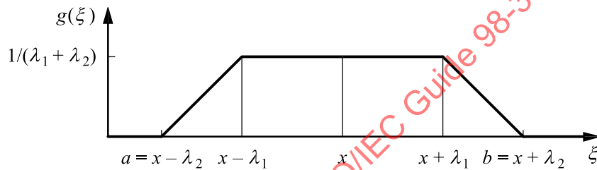
Figure 5 — The trapezoidal PDF for X = X_1 + X_2 , where the PDFs for X_1 and X_2 are rectangular (6.4.4.2)
