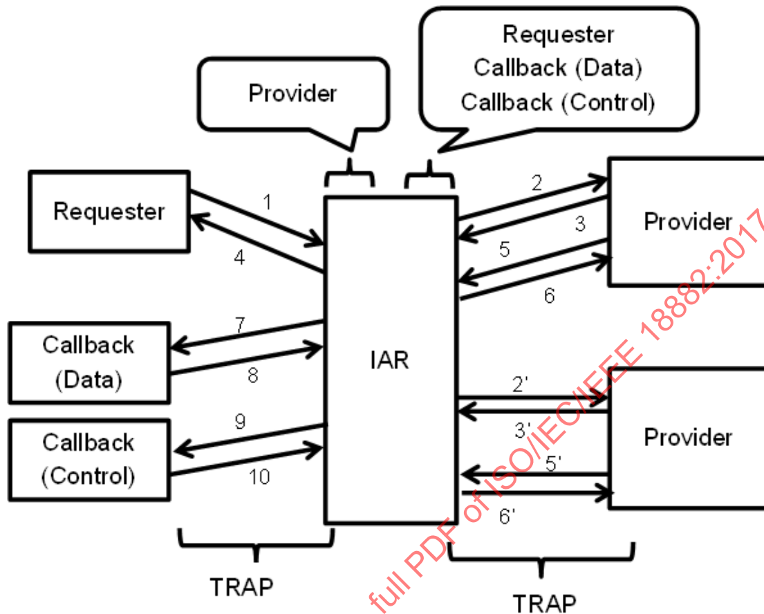
Figure 8—The IAR as a TRAP provider
