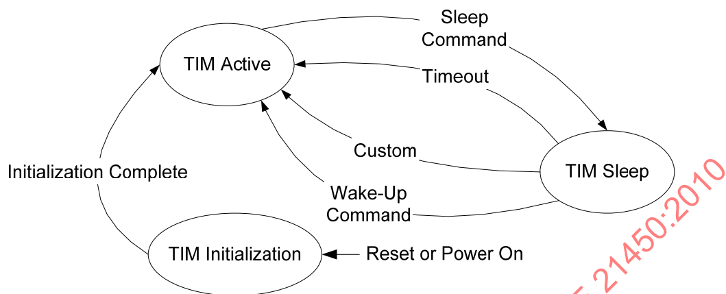
Figure 4—TIM operating states
