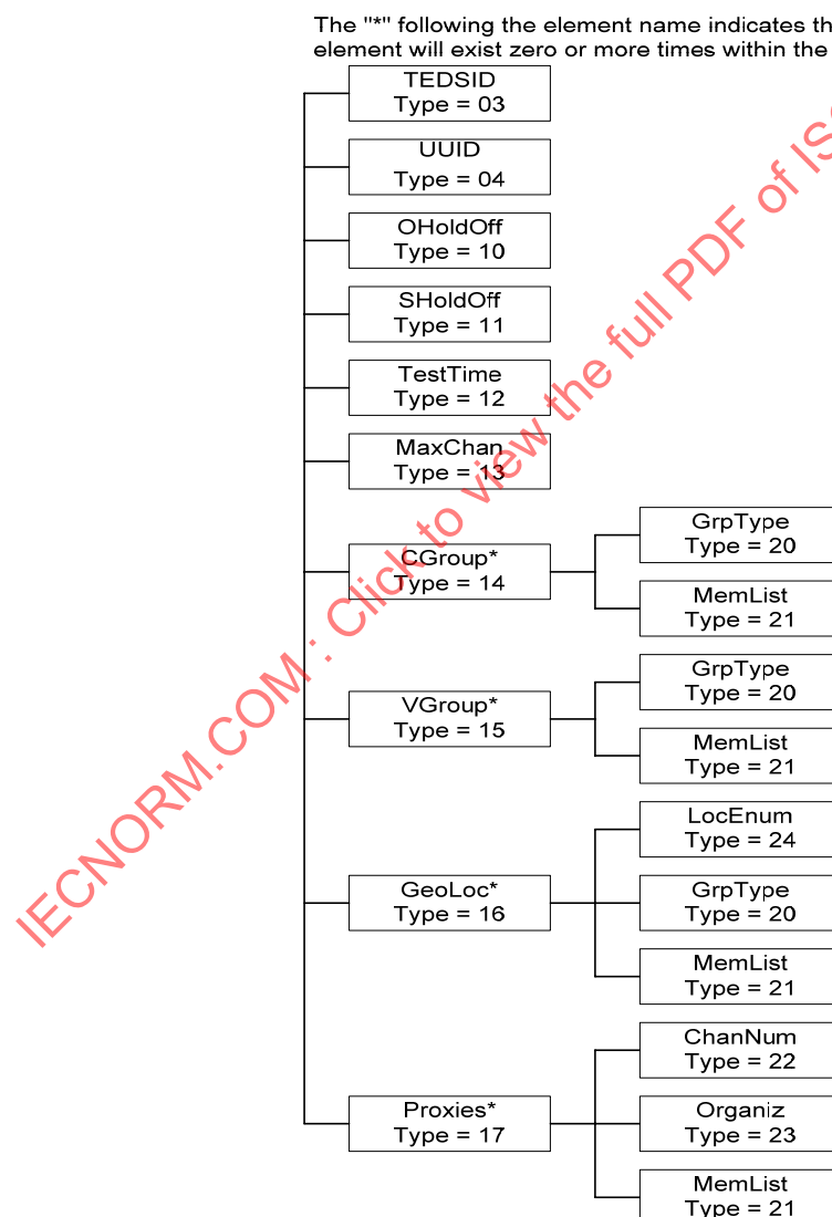
Figure 13—Structure of the Meta-TEDS data block
