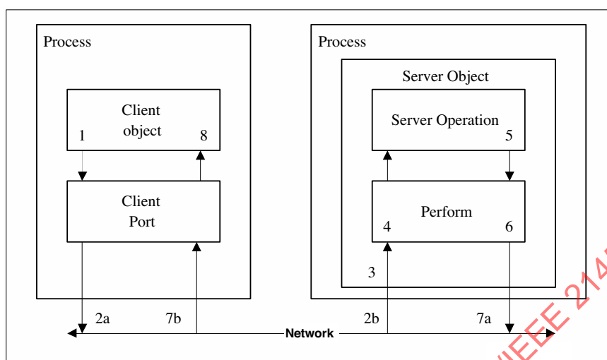
Figure 33— Client-server communication
