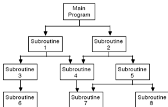
Figure 5 — Call graph
