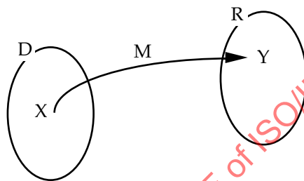
Figure 43—Mapping
