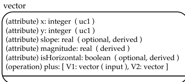
Figure 65—Operations
