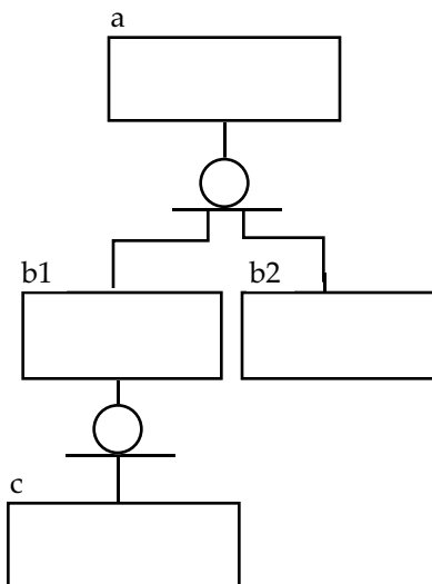
Figure 27—Changing specialization
