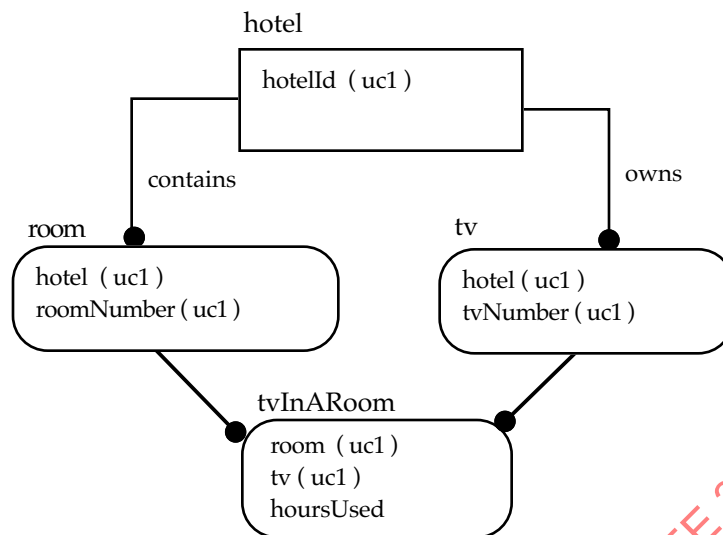
Figure 71—Uniqueness constraints
