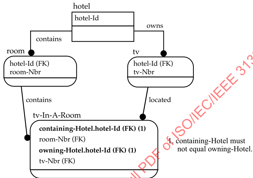
Figure 98—Distinct ancestor
