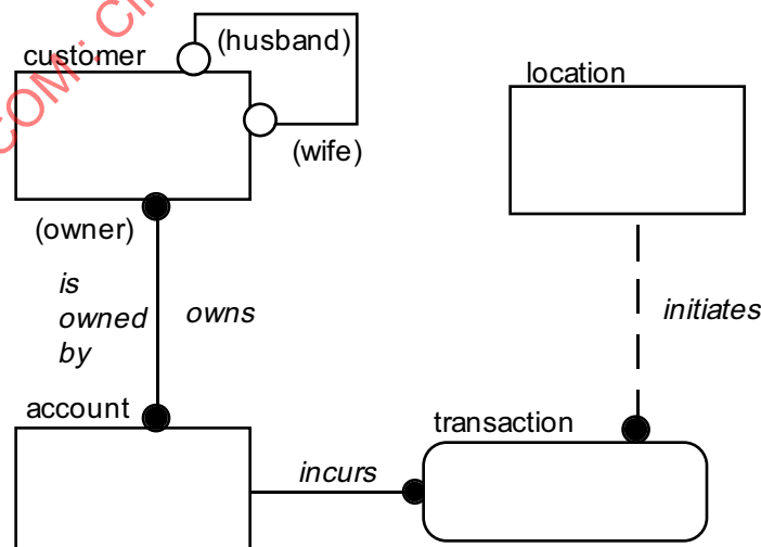
Figure 34—Relationships
