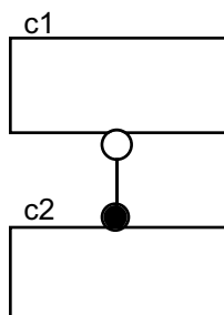
Figure 37—Deletion case 3
