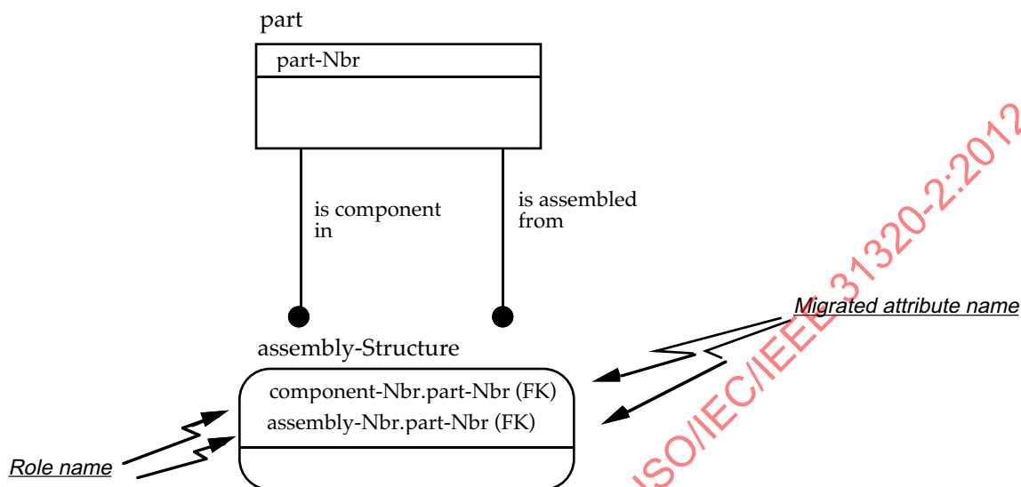
Figure 96—Key-style role name syntax
