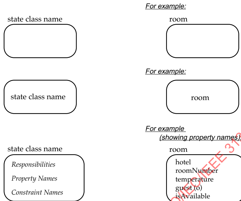
Figure 9—Alternatives for dependent state class labeling
