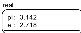
Figure 21—Value class class-level property instance diagram
