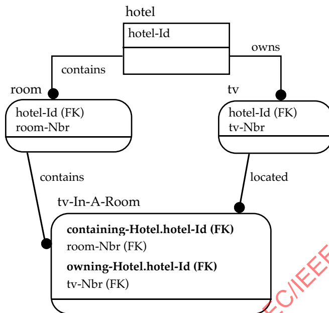
Figure 99—Common ancestor with no restriction
