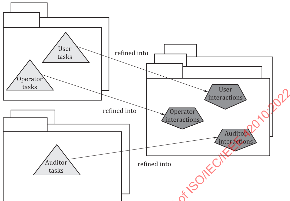
Figure A.3 — Example of a correspondence satisfying the Task-Interactions method
