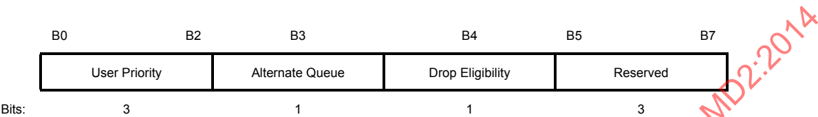
Figure 8-401e—Intra-Access Priority field format
