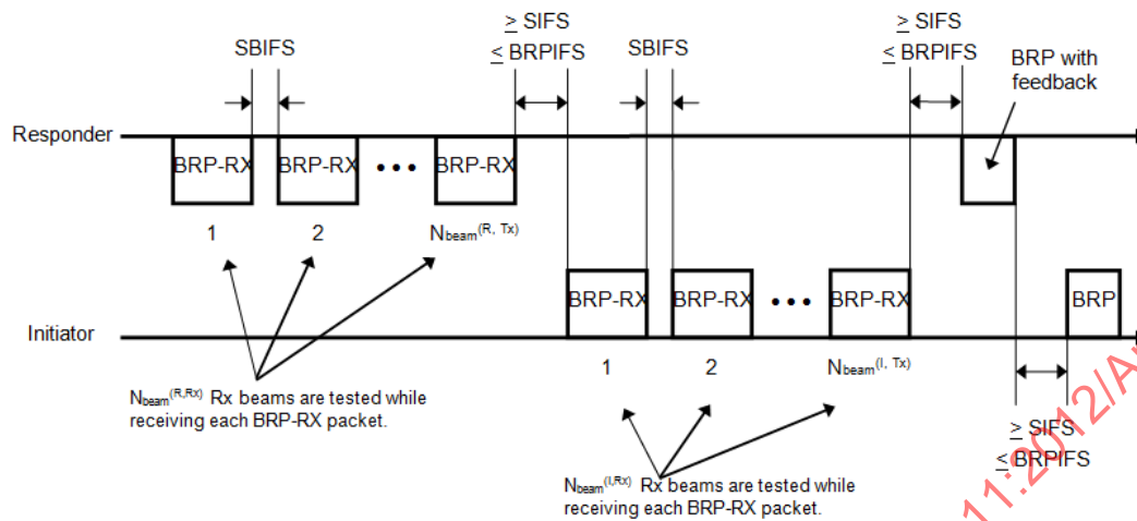
Figure 9-64—Beam combining
