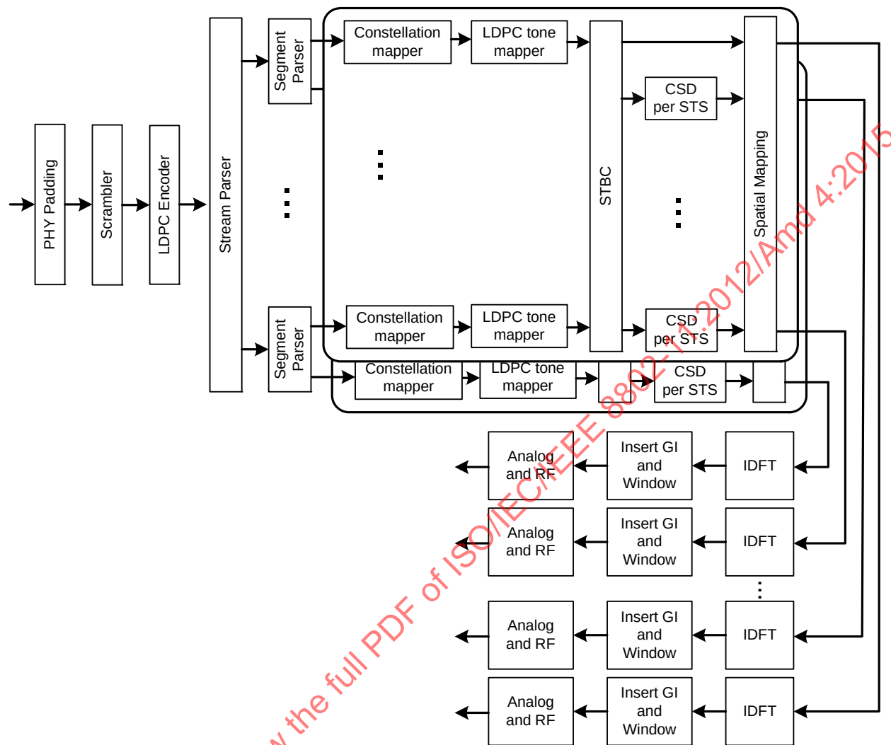
Figure 22-16—Transmitter block diagram for the Data field of an 80+80 MHz VHT SU PPDU with LDPC encoding
