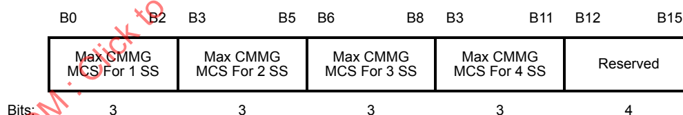
Figure 9-589dk—Rx CMMG MCS Map and Tx CMMG MCS Map subfields and Basic CMMG MCS and NSS Set field
