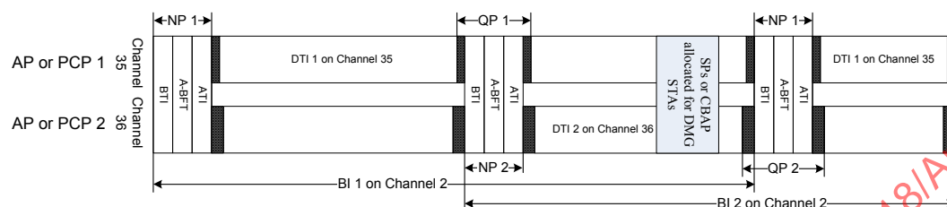
Figure 10-115—SPs or CBAPs allocated for DMG STAs on channel 2 without starting a beacon interval on channels 35 and 36
