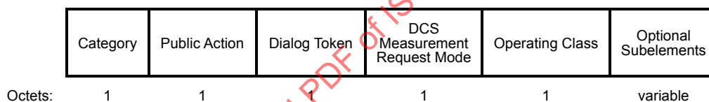
Figure 9-687f—DCS Measurement Request frame Action field format
