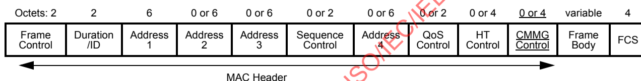
Figure 9-1—MAC frame format
