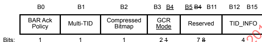
Figure 9-27—BAR Control field
