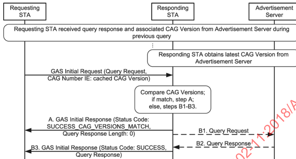
Figure 11-40d—GAS frame exchange sequence using CAG Version
