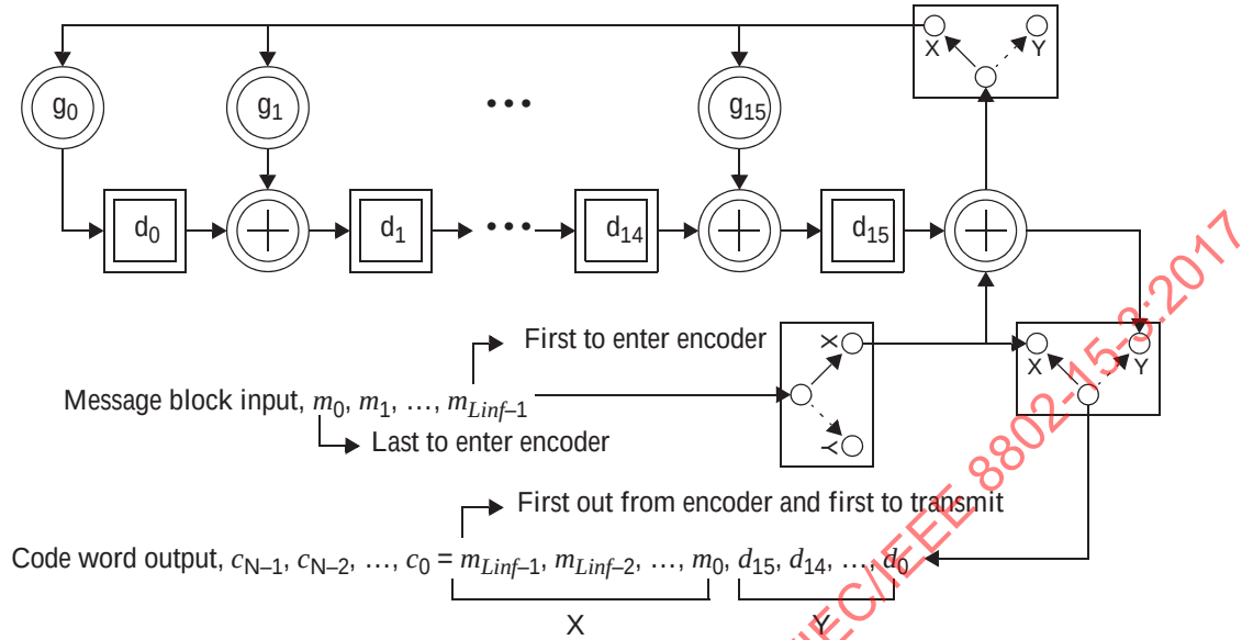
Figure 11-12—Reed Solomon encoder GF(2 8 )
