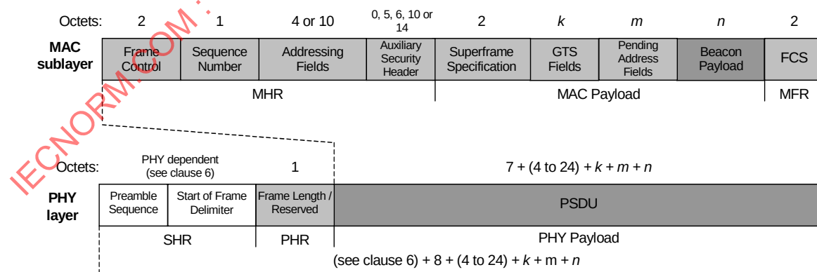
Figure 10—Schematic view of the beacon frame and the PHY packet
