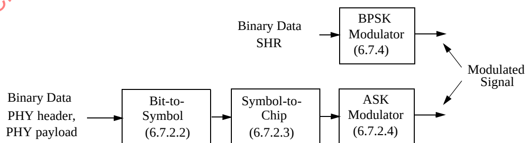
Figure 22—Modulation and spreading functions
