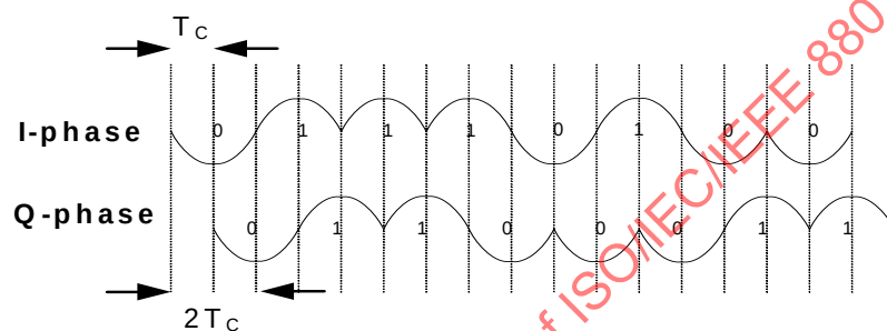
Figure 27—Sample baseband chip sequences with pulse shaping
