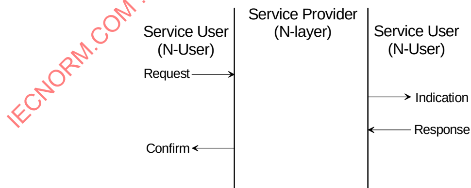
Figure 14—Service primitives
