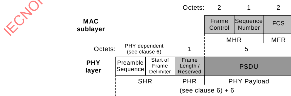
Figure 12—Schematic view of the acknowledgment frame and the PHY packet
