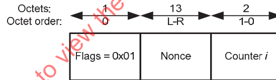
Figure 112 —Counter blocks Ctr_0, \dots, Ctr_m format
