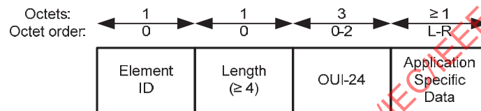
Figure 59—Application Specific IE format
