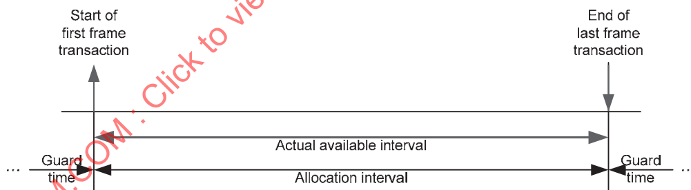
Figure 94—Centralized provisioning of guard times for frame transmissions
