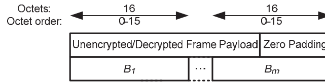
Figure 111 —Payload blocks B_1, \dots, B_m format
