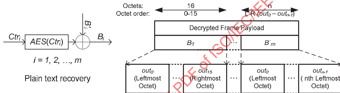
Figure 115 —Decrypted Frame Payload format for encrypted frames
