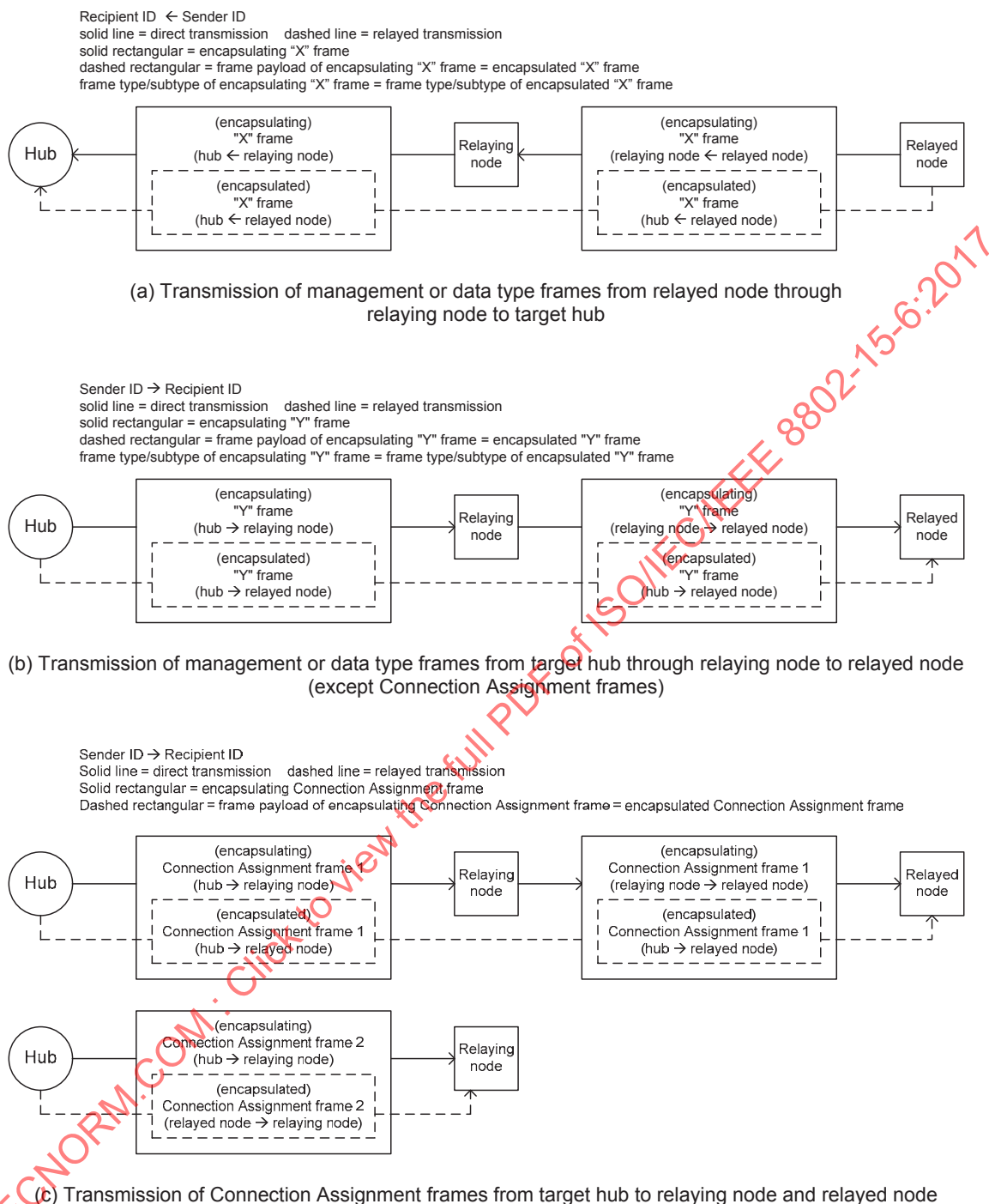
Figure 88—Management or data type frame exchanges on a two-hop extension
