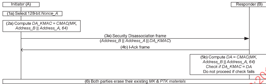
Figure 106 —Security disassociation procedure
