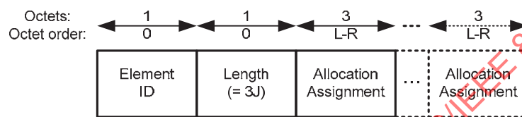
Figure 51 —Uplink Assignment, Downlink Assignment, Bilink Assignment, or Type-I Unscheduled Bilink Assignment IE format
