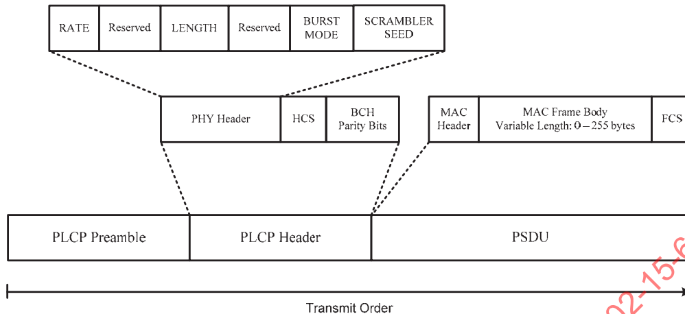
Figure 116—Standard PPDU structure
