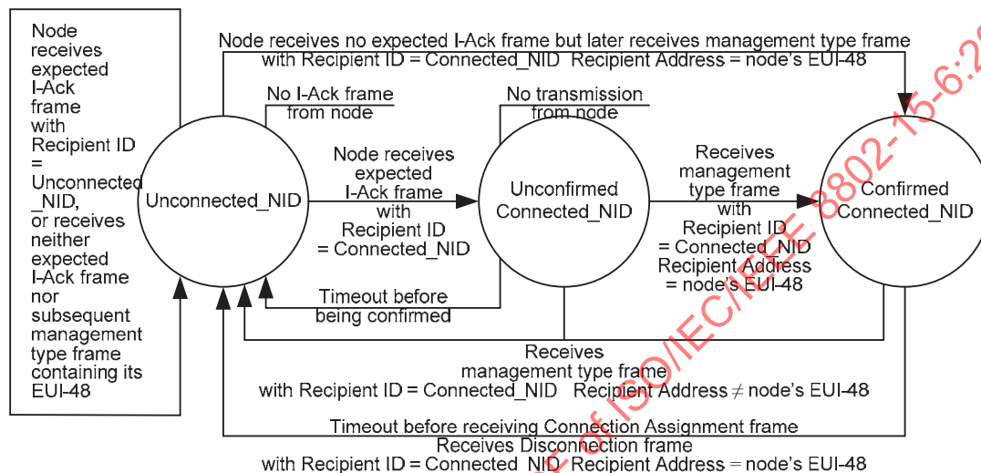
Figure 60—Node NID transition
