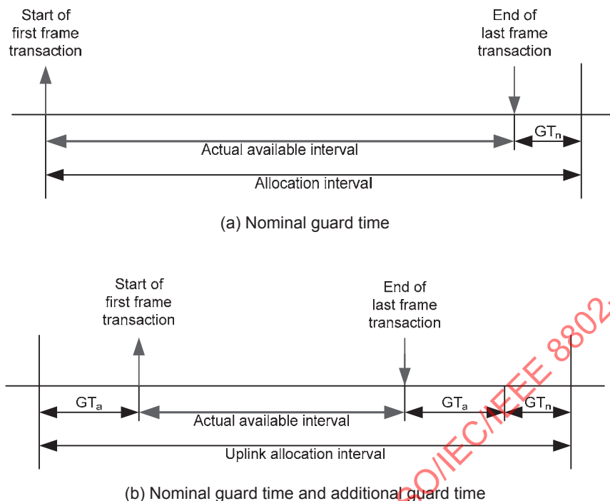
Figure 92—Distributed provisioning of guard times for frame transmissions
