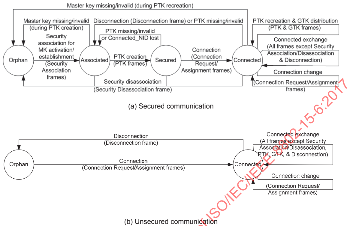
Figure 4—MAC and security state diagrams
