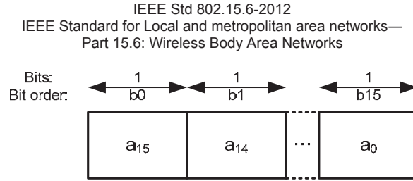
Figure 13—FCS format
