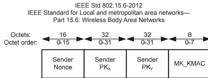
Figure 21—Security Association Data format for security association protocols 1 to 4
