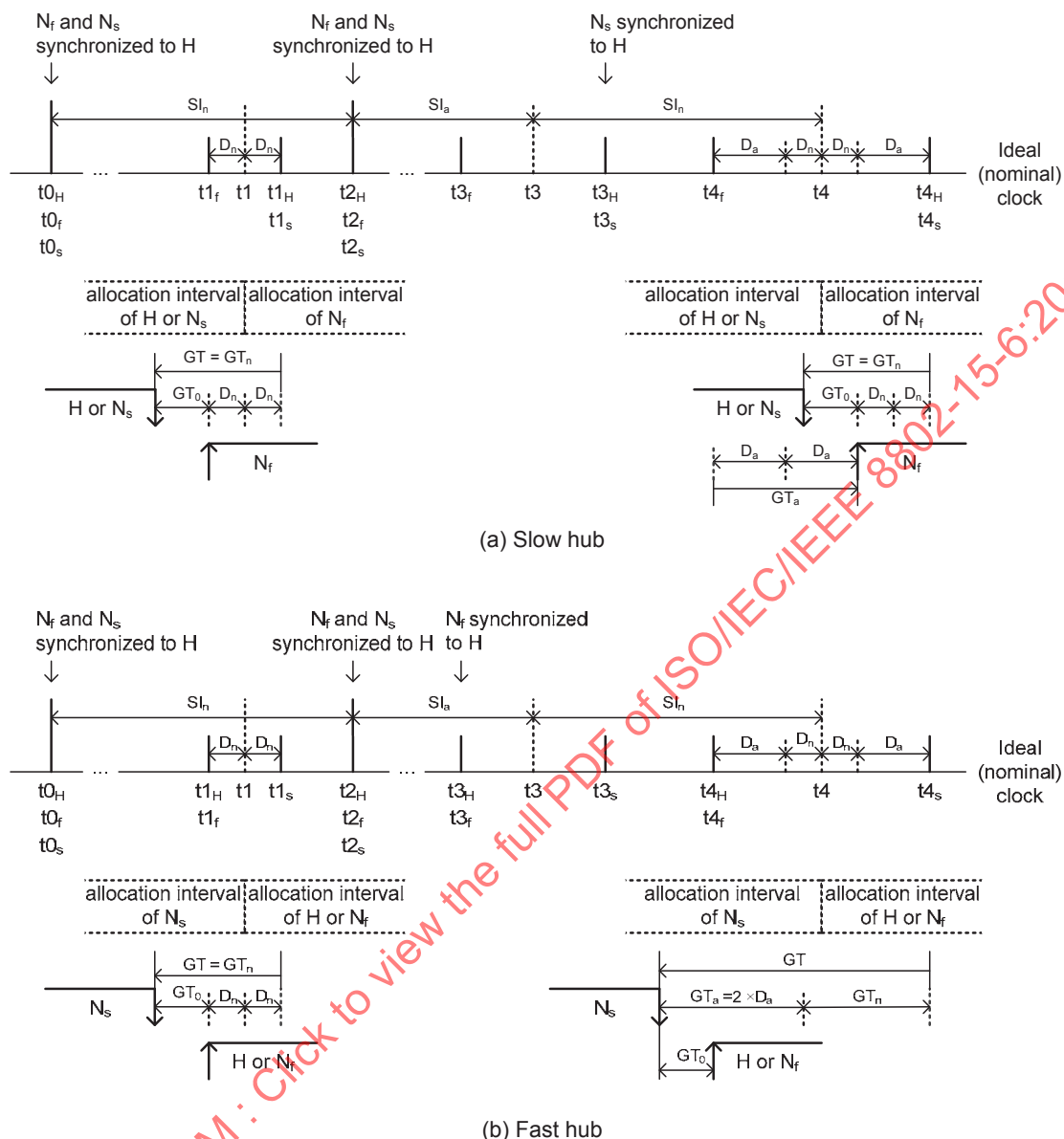
Figure 91—Analysis of clock drifts and guard times for distributed provisioning
