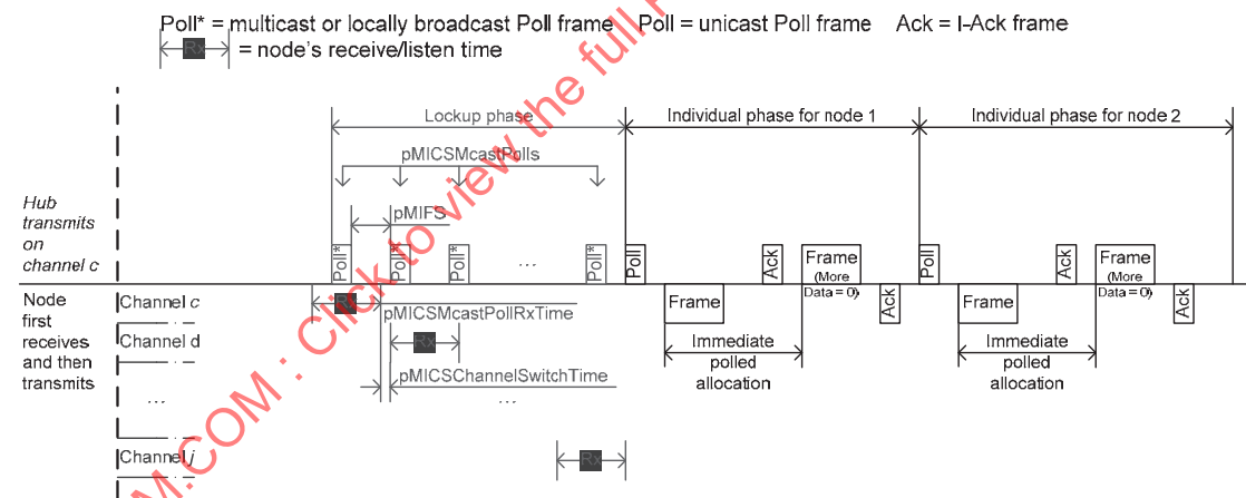
Figure 84—Multicast poll aided connected discovery and frame exchange in MICS band
