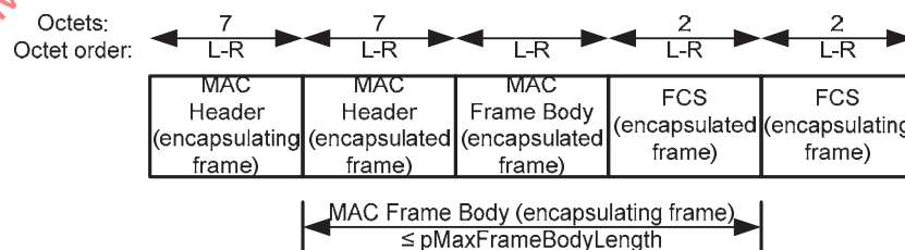
Figure 87—General frame encapsulation format
