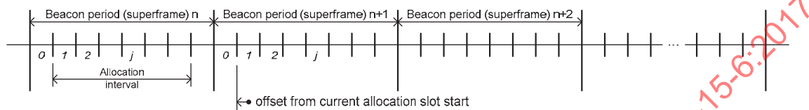
Figure 3—Time reference base
