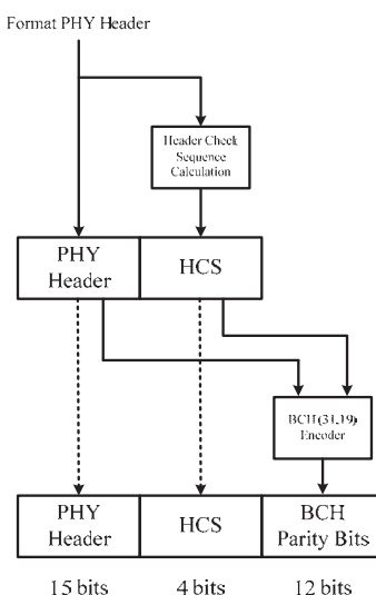
Figure 118 —BCH encoding scheme for PLCP header construction
