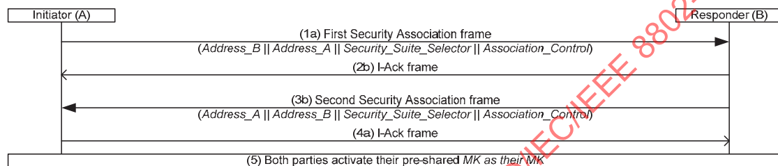
Figure 102 —MK pre-shared association procedure
