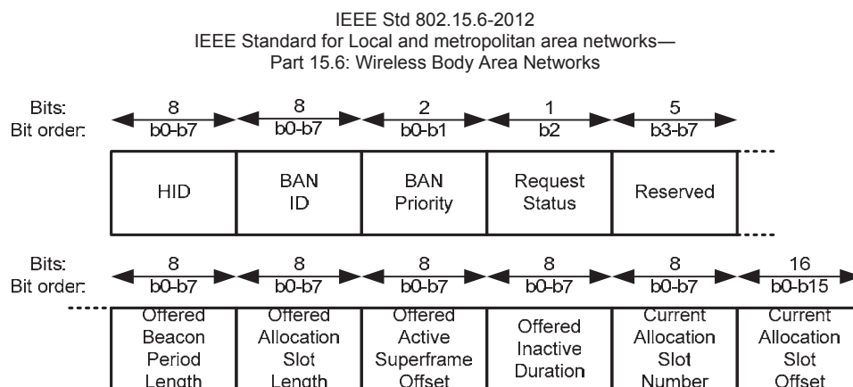
Figure 36—Command Data format for Command—Active Superframe Interleaving Response frames
