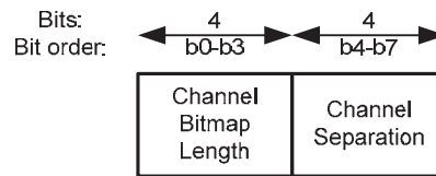
Figure 57 —Channel Control format
