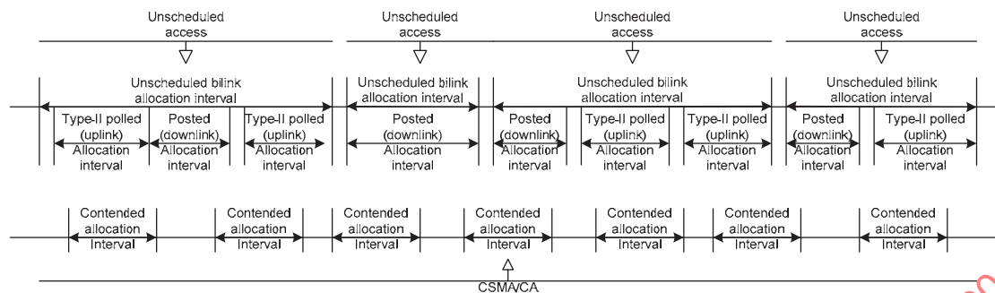
Figure 67—Allocation intervals and access methods permitted for non-beacon mode without superframes
