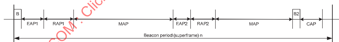
Figure 64—Layout of access phases in a beacon period (superframe) for beacon mode
