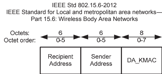
Figure 22—Frame Payload format for Security Disassociation frames
