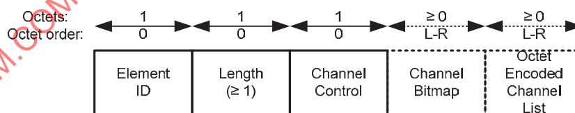
Figure 56—Channel Hopping and Ordering IE format
