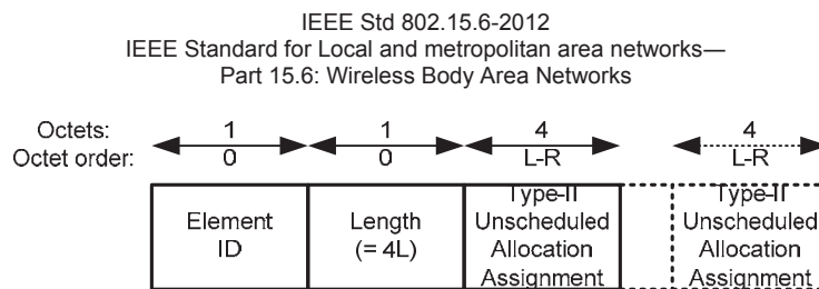
Figure 53—Type-II Unscheduled Bilink Assignment IE format
