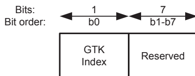
Figure 26—GTK Control format
