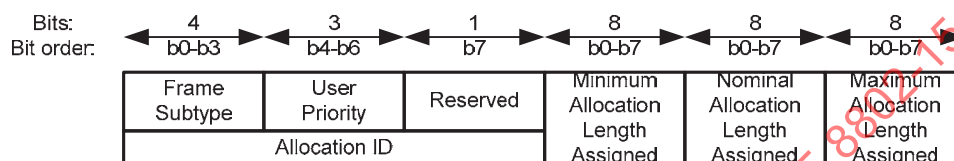
Figure 54—Type-II Unscheduled Allocation Assignment format
