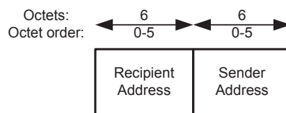
Figure 40—Frame Payload format for Wakeup frames
