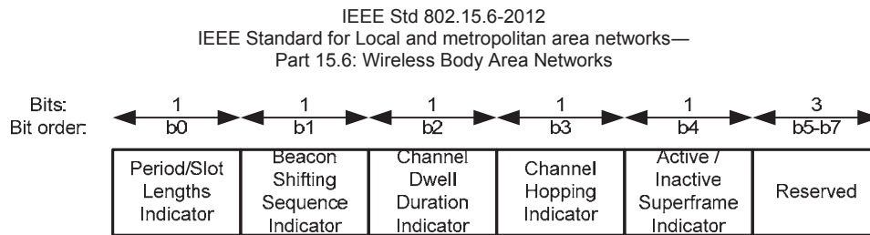
Figure 46—Superframe Parameters Bitmap format
