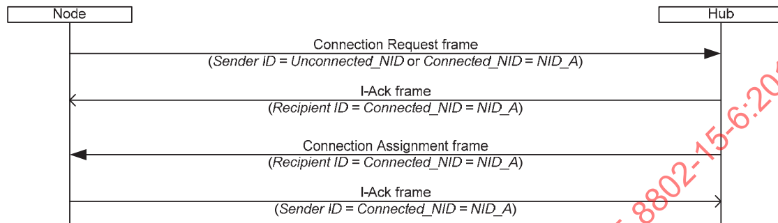
Figure 68—Connection procedure
