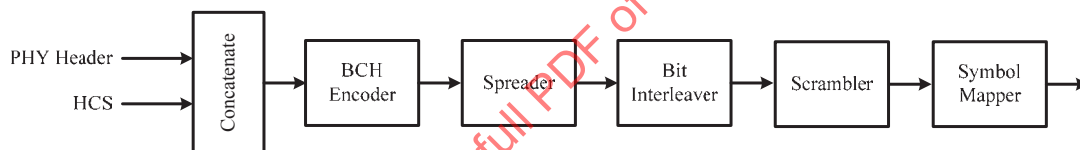
Figure 117 —Block diagram of PLCP header construction for transmission
