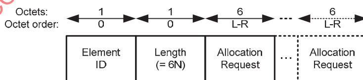
Figure 47 —Uplink Request, Downlink Request, Bilink Request, or Type-I Unscheduled Bilink Request IE format
