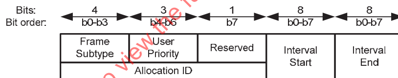
Figure 52 —Allocation Assignment format
