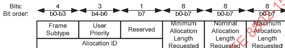
Figure 50—Type-II Unscheduled Allocation Request format
