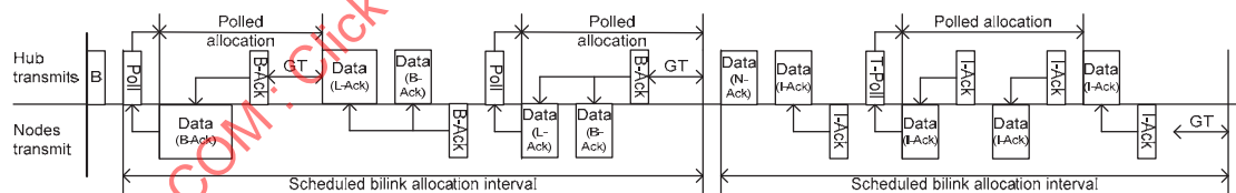
Figure 81 —Example frame transactions in scheduled bilink allocation intervals
