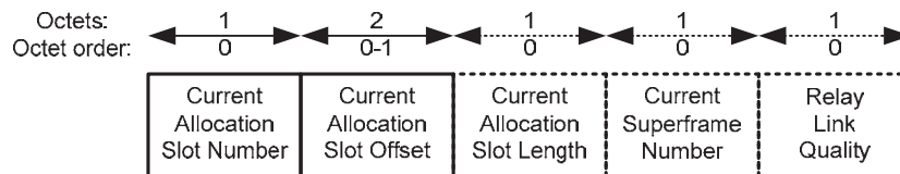
Figure 39—Frame Payload format for T-Poll frames
