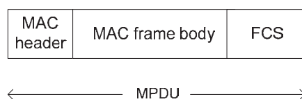
Figure 130 —MPDU structure
