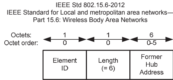
Figure 58—Former Hub Address IE format
