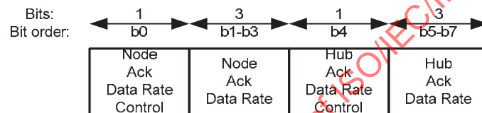
Figure 29—Requested Ack Data Rates and Assigned Ack Data Rates format
