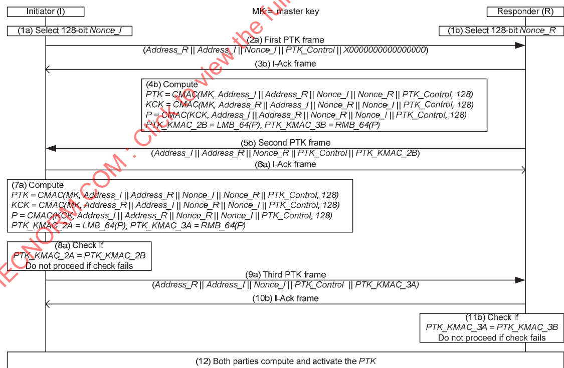
Figure 107 —PTK creation procedure
