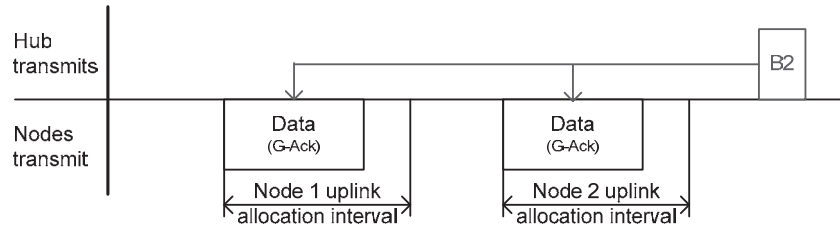
Figure 61—Group acknowledgment (G-ACK)
