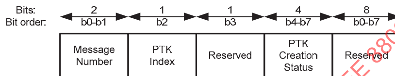
Figure 24—PTK Control format
