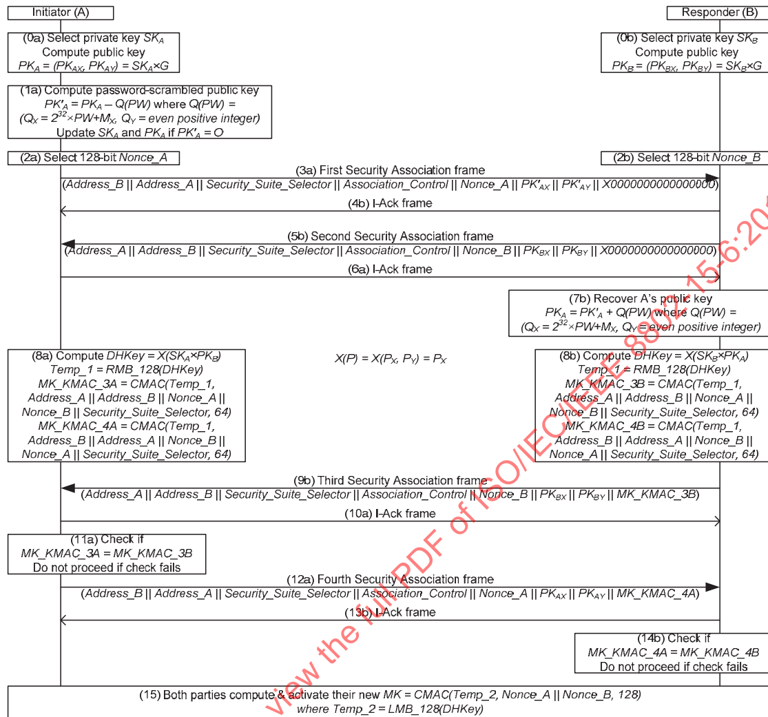
Figure 104 — Password authenticated association procedure
