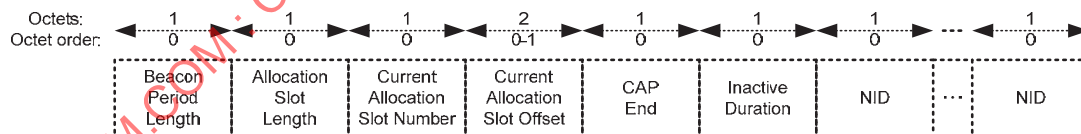
Figure 41—Frame Payload format for B2 frames
