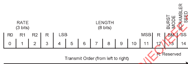
Figure 119 —PHY header bit assignment
