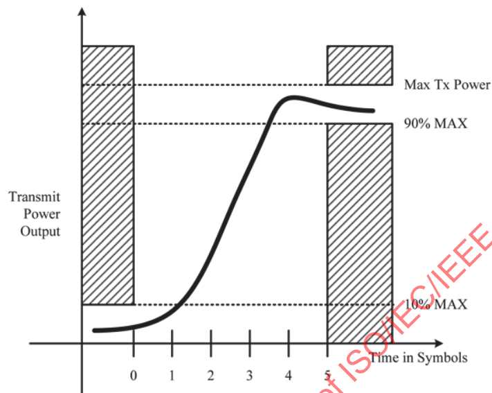
Figure 126 —Transmit power-on ramp
