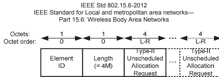
Figure 49—Type-II Unscheduled Bilink Request IE format
