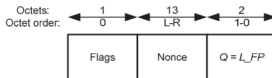
Figure 110 —Initial block B_0 format
