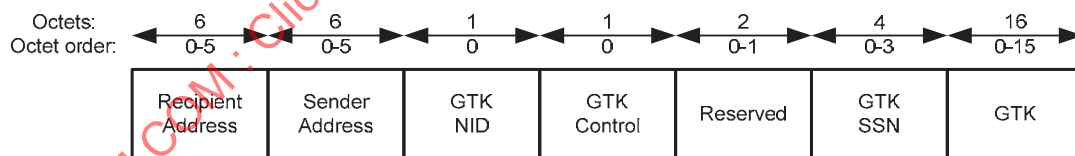
Figure 25—Frame Payload format for GTK frames
