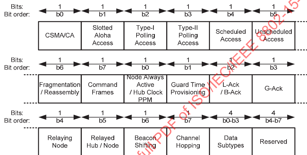
Figure 42—MAC Capability format
