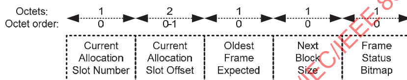
Figure 38—Frame Payload format for B-Ack frames
