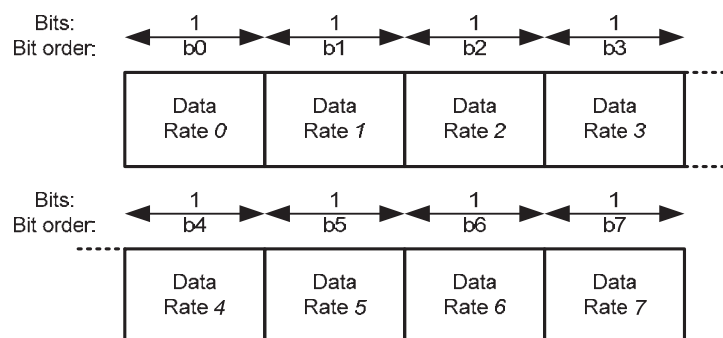
Figure 43—PHY Capability format
