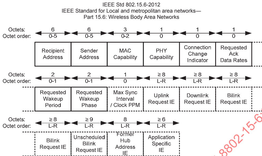
Figure 27 —Frame Payload format for Connection Request frames
