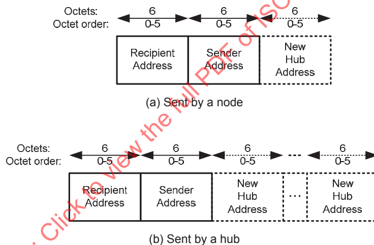
Figure 33—Frame Payload format for Disconnection frames
