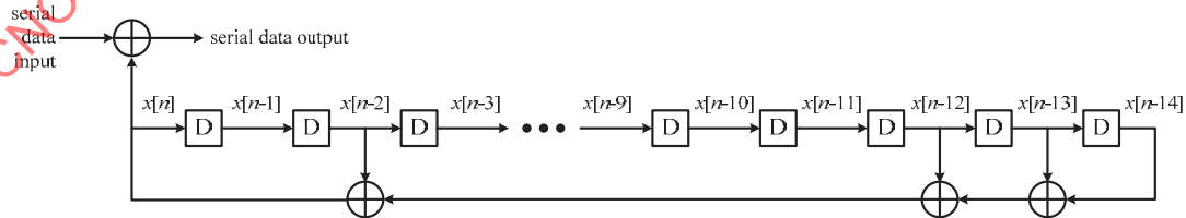
Figure 124 —Block diagram of a side-stream scrambler
