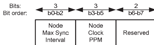
Figure 30—Max Sync Interval/Clock PPM format
