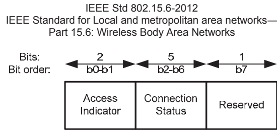
Figure 32—Mode/Status format
