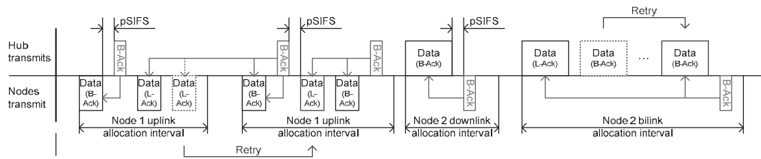
Figure 63—Late acknowledgement (L-ACK) and block acknowledgement (B-Ack) illustration
