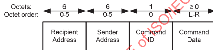
Figure 34—Frame Payload format for Command frames
