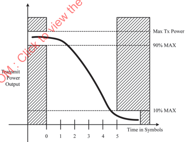
Figure 127 —Transmit power-down ramp
