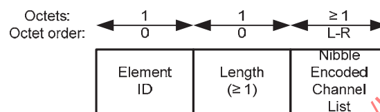
Figure 55—Nibble Encoded Channel Order IE format
