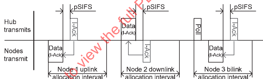
Figure 62—Immediate acknowledgment (I-Ack) illustration
