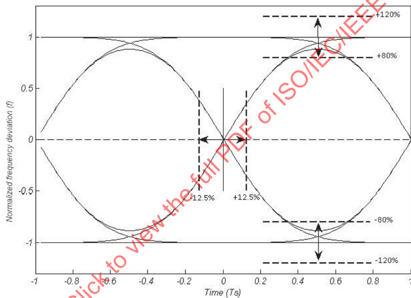
Figure 128—GMSK modulation accuracy
