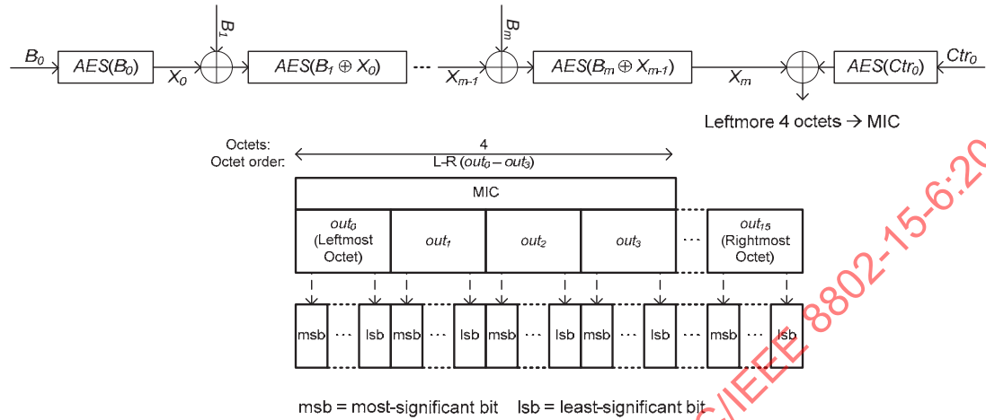
Figure 113 —MIC calculation and transmit order
