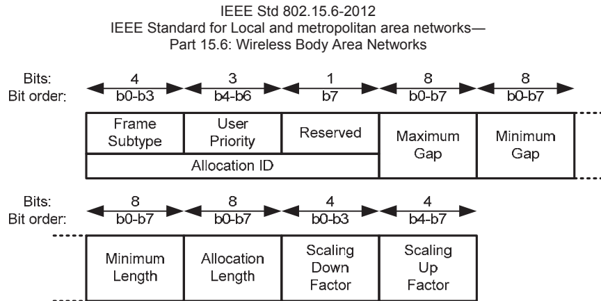
Figure 48—Allocation Request format
