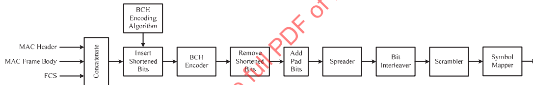
Figure 121 —Block diagram of PSDU construction for transmission
