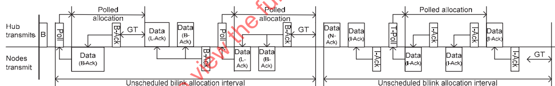
Figure 78—Example frame transactions in unscheduled bilink allocation intervals
