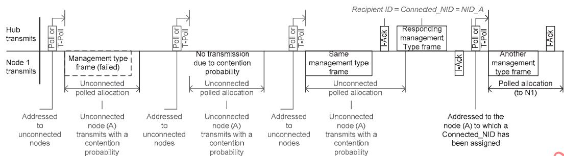
Figure 69—Unconnected and unicast polled allocations for unconnected nodes
