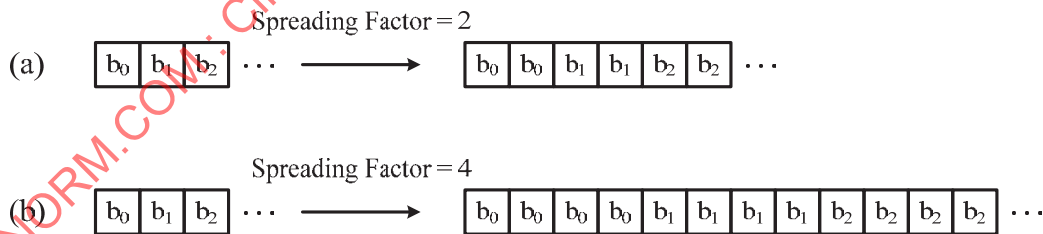
Figure 123 —Spreading scheme
