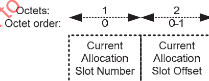
Figure 37—Frame Payload format for I-Ack frames
