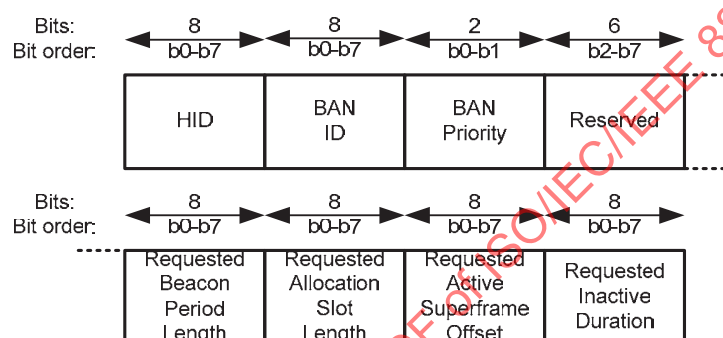
Figure 35—Command Data format for Command—Active Superframe Interleaving Request frames
