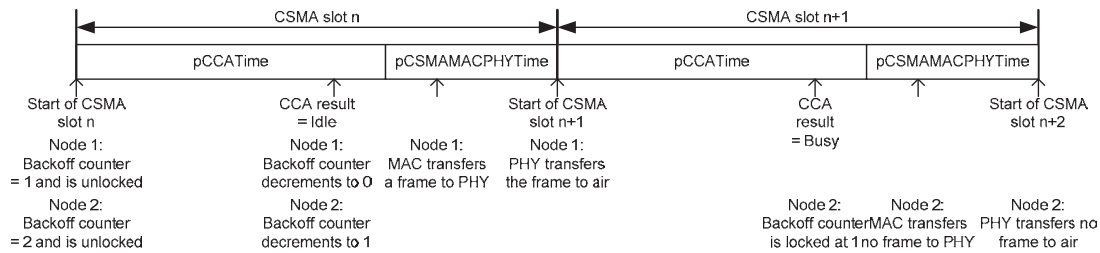
Figure 71 —CSMA slot structure
