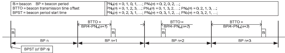
Figure 97—Beacon shifting illustration with PN_4(n)
