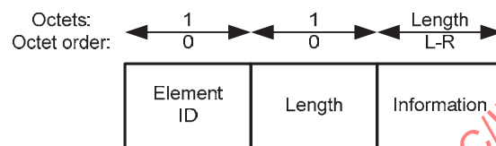
Figure 44—IE format—general
