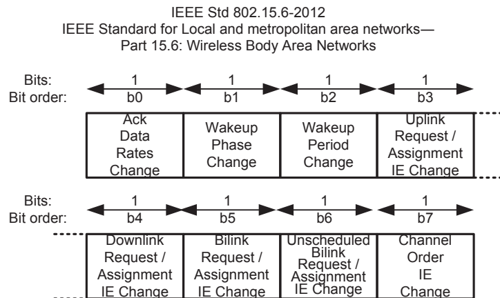
Figure 28—Connection Change Indicator format
