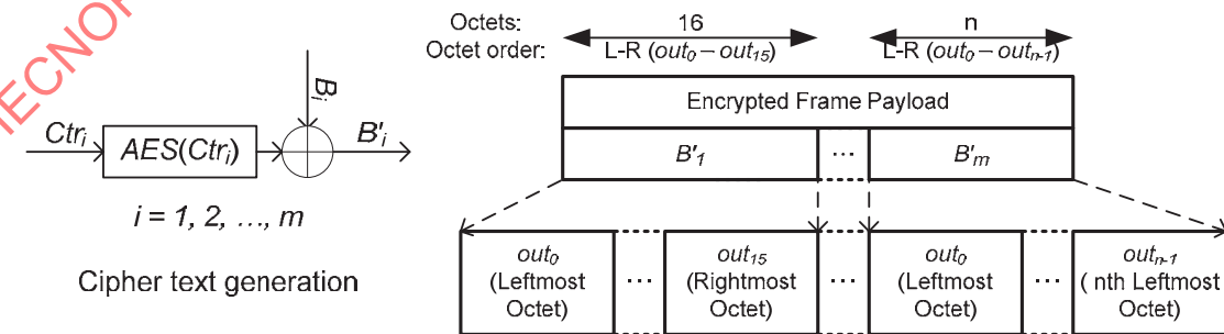
Figure 114 —Encrypted Frame Payload format for encrypted frames
