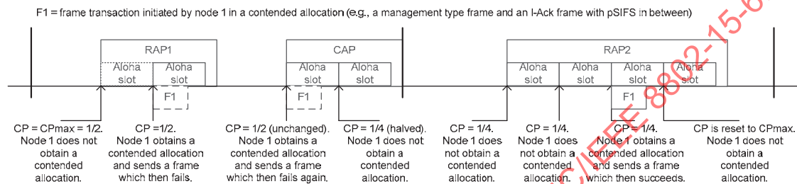
Figure 74—Slotted Aloha access illustration
