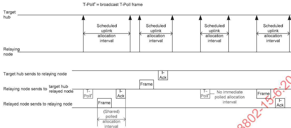
Figure 89—Scheduled uplink allocation for relaying node to send broadcast T-Polls and to relay frames
