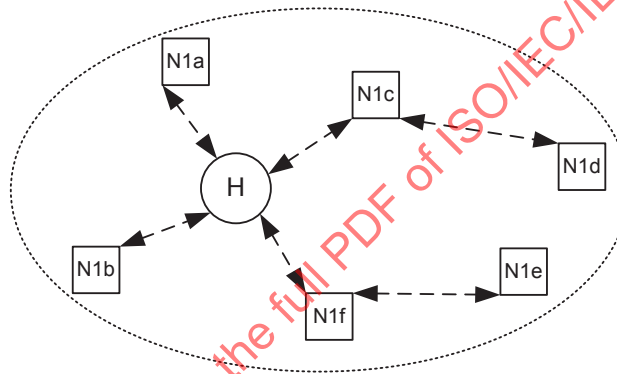
Figure 86—Two-hop extended star network topology
