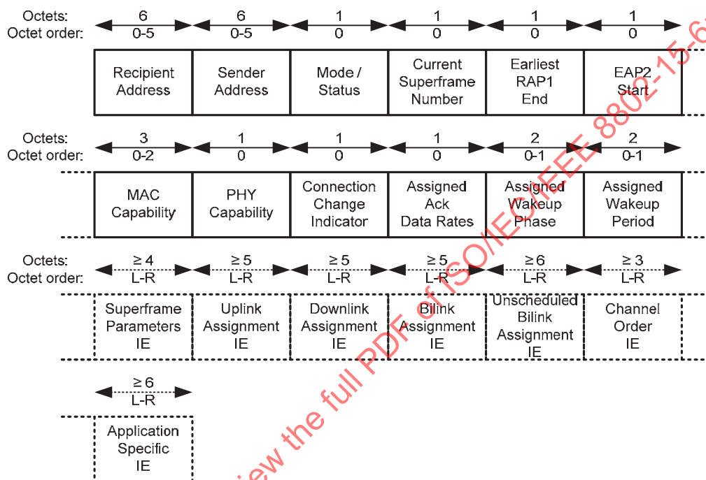
Figure 31—Frame Payload format for Connection Assignment frames
