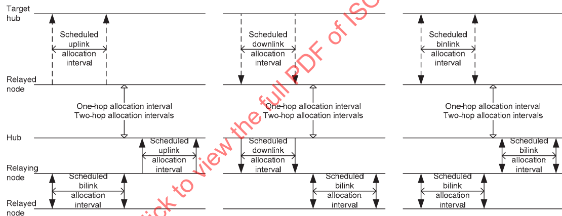
Figure 90—Equivalent one-hop and two-hop scheduled allocations
