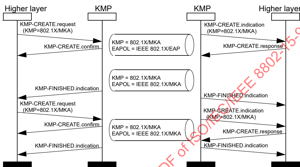
Figure A.1—IEEE 802.1X/EAP and IEEE 802.1X/MKA as a PAN KMP
