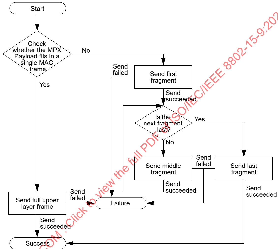
Figure 13—Outbound flow diagram
