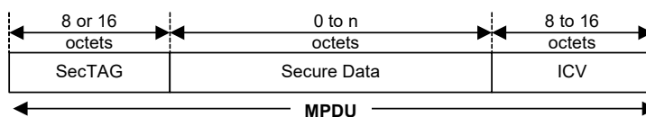
Figure 9-1—MPDU components
