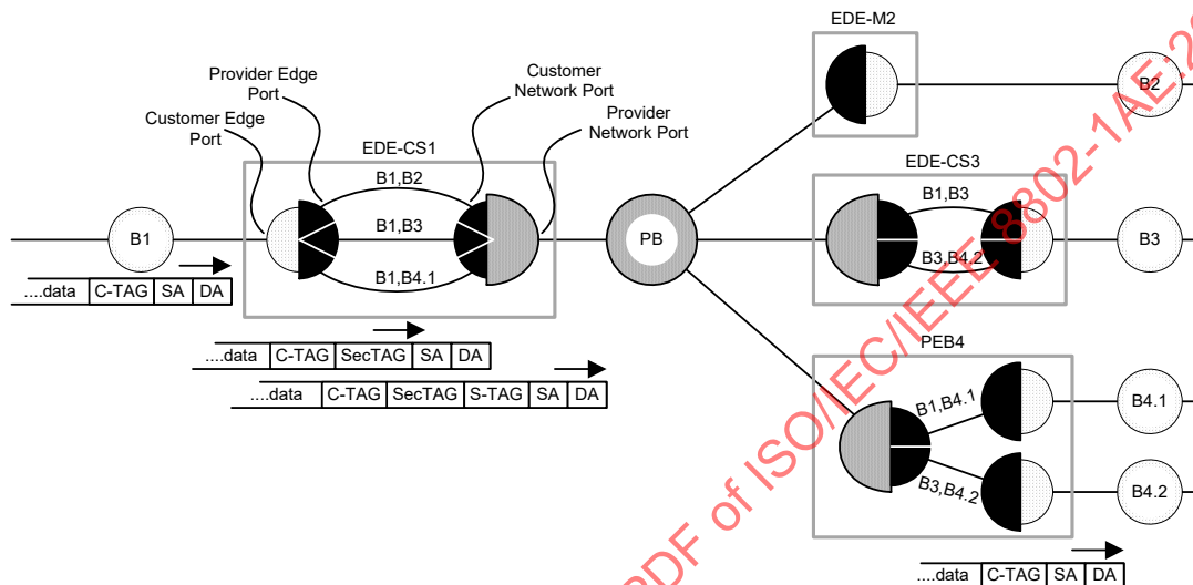
Figure 15-6—Example network with an EDE-CS
