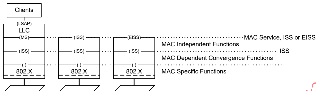
Figure 11-2—Provision of MAC Service with media-independent functions
