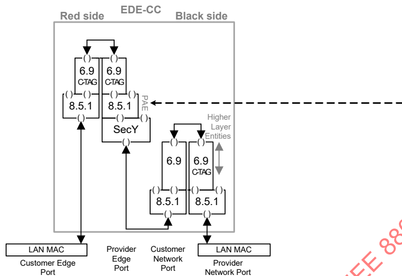
Figure 15-9—EDE-CC architecture
