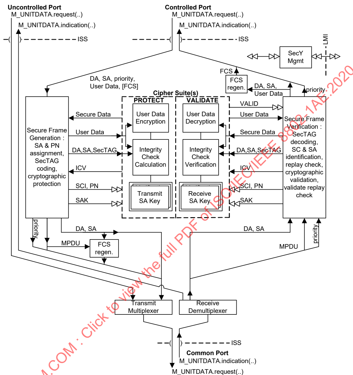
Figure 10-2—SecY architecture and operation
