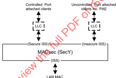
Figure 11-3—MACsec in an end station
