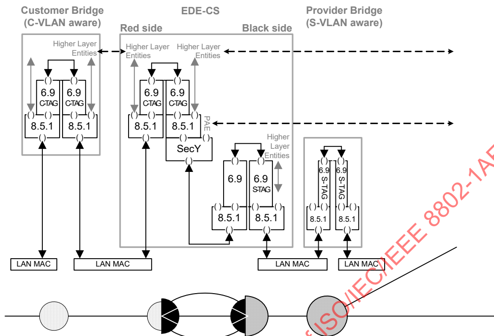
Figure 15-7—EDE-CS connected to a PBN S-tagged interface
