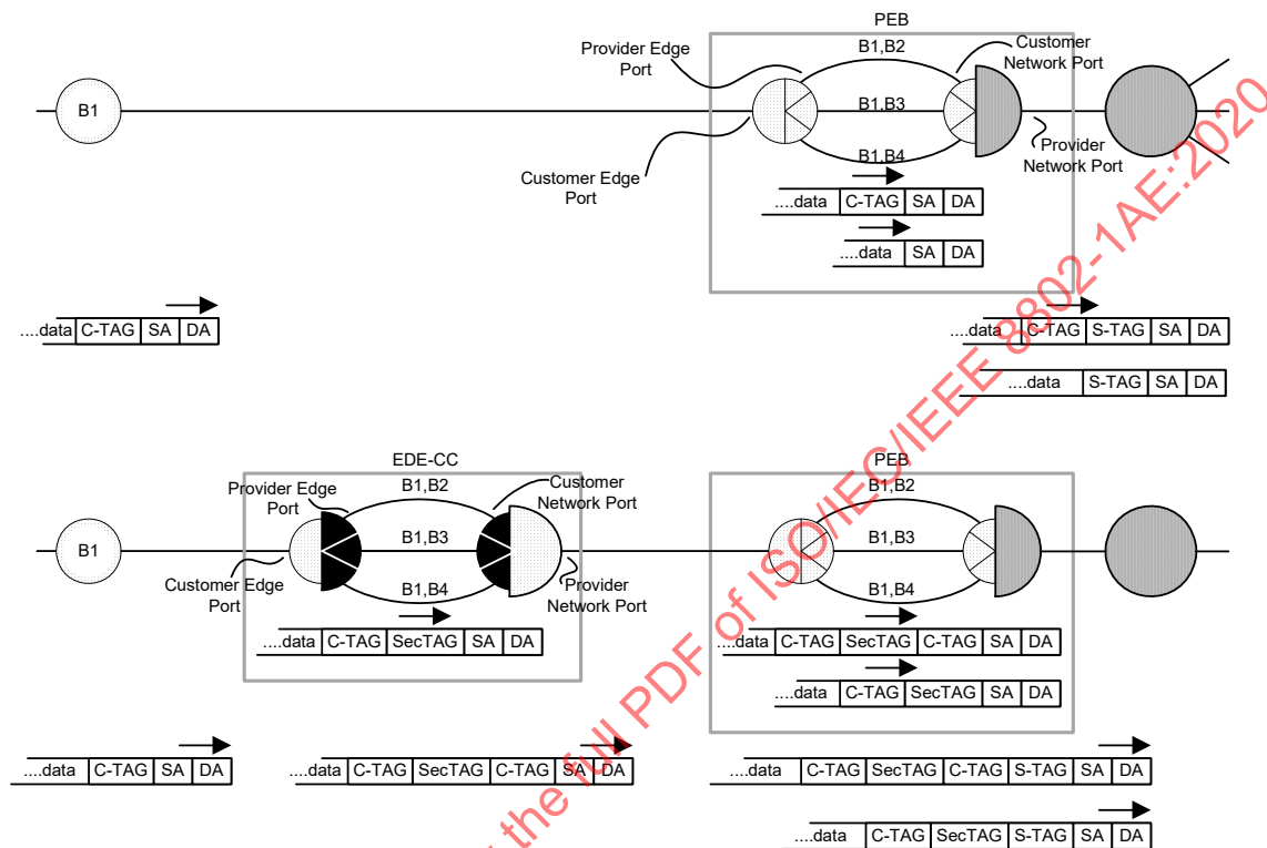
Figure 15-8—Using an EDE-CC with a C-tagged provider service interface
