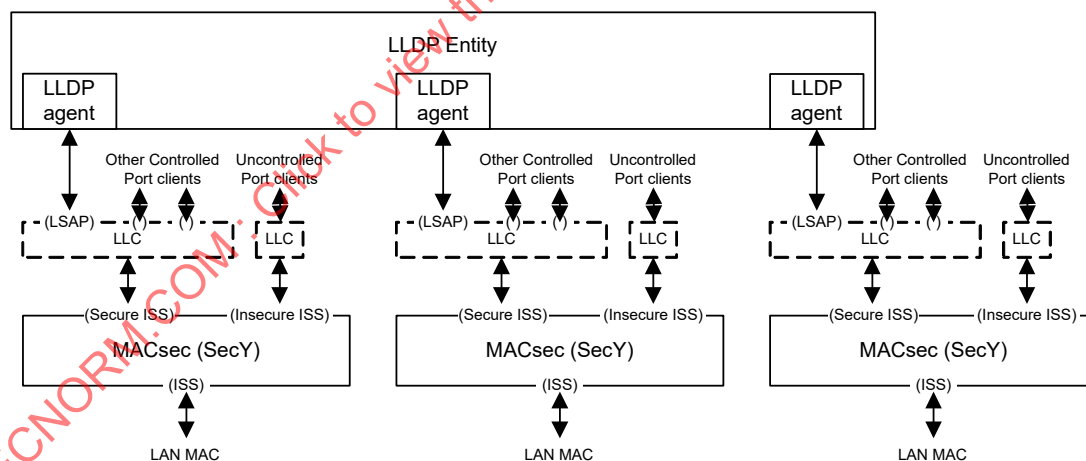
Figure 11-10—MACsec with LLDP
