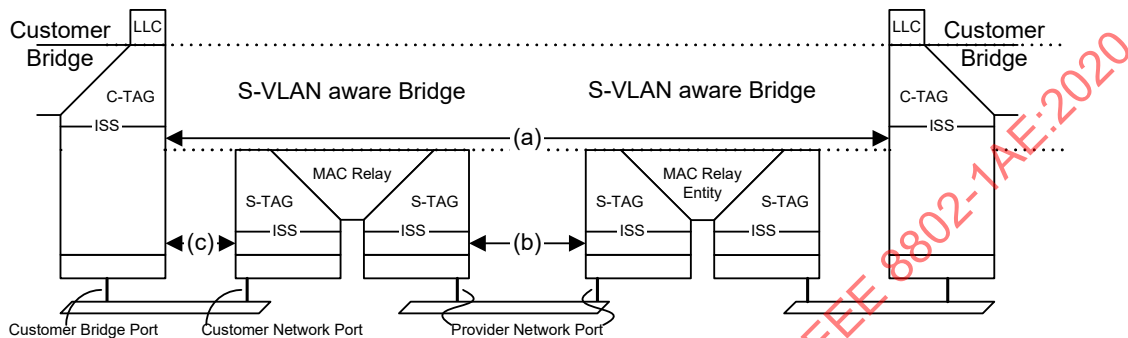
Figure 11-11—Internal organization of the MAC sublayer in a Provider Bridged Network
