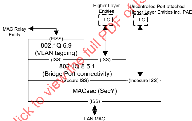
Figure 11-7— IEEE 802.1Q VLAN-aware Bridge Port with MACsec
