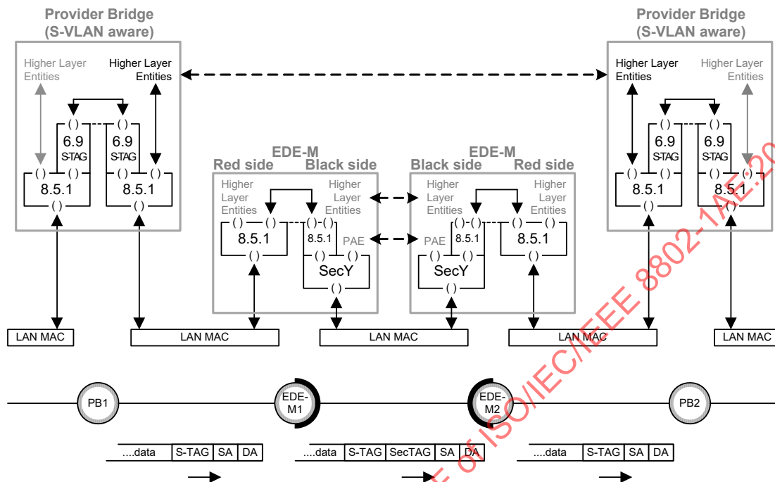
Figure 15-2—EDE-Ms securing a point-to-point LAN between Provider Bridges
