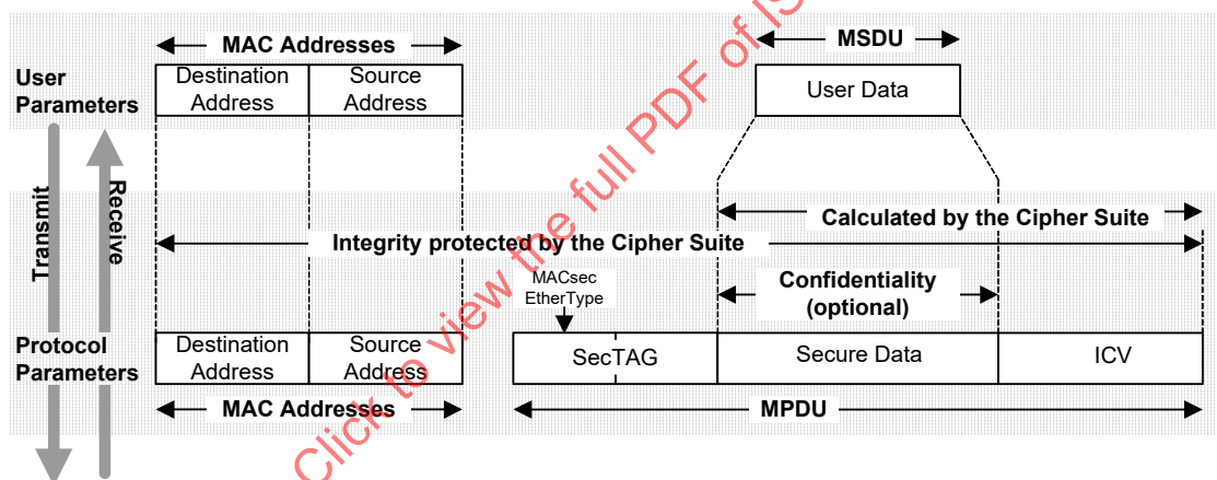
Figure 8-1—MACsec
