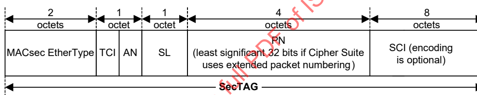
Figure 9-2—SecTAG format
