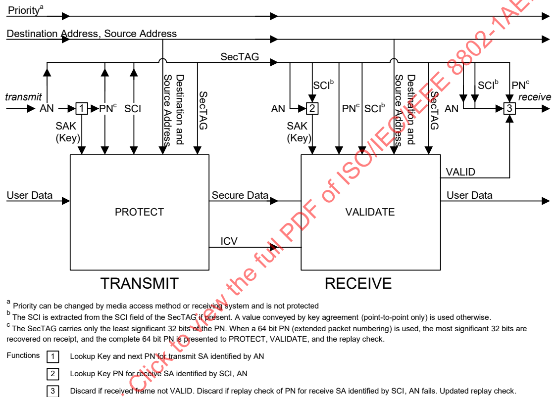
Figure 8-2—MACsec operation
