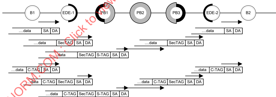
Figure 15-3—MACsec protected frame traversing a PBN
