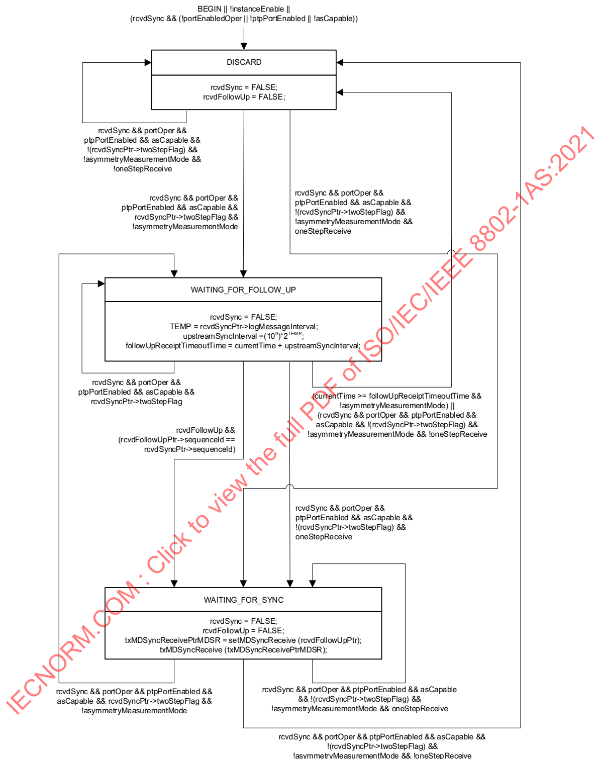
Figure 11-6—MDSyncReceiveSM state machine
