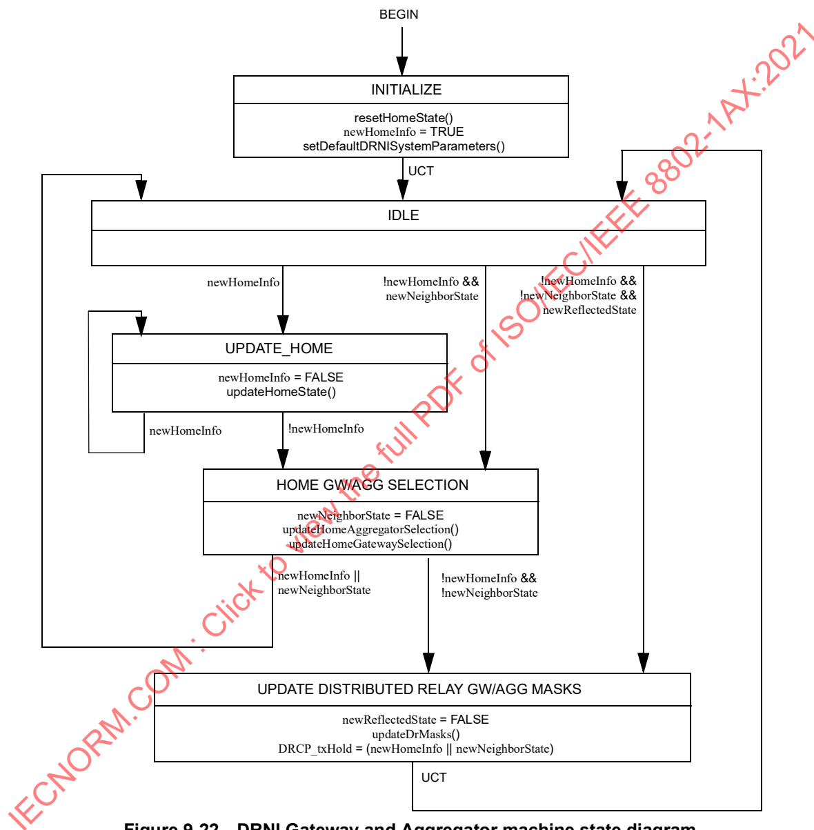
Figure 9-22—DRNI Gateway and Aggregator machine state diagram
