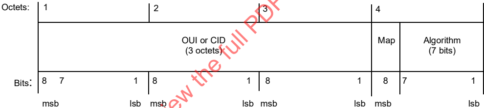
Figure 8-1—Distribution algorithm identifiers
