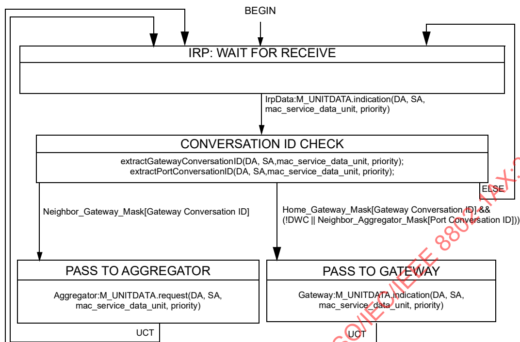
Figure 9-10—DR_IRP state machine
