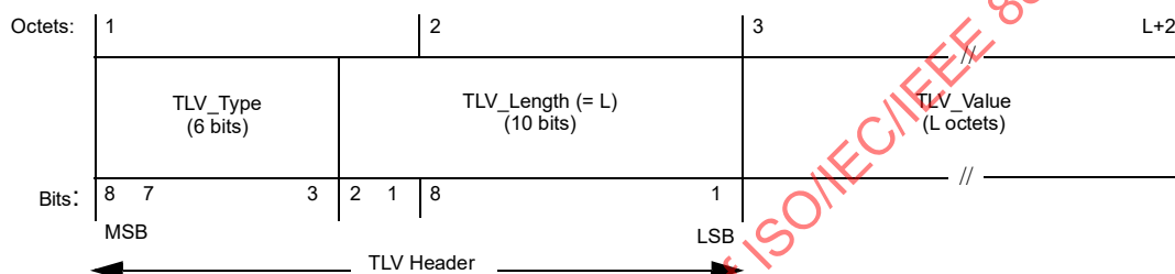
Figure 9-11—Basic TLV format
