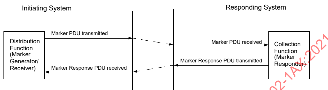
Figure 6-18—Marker protocol time sequence diagram
