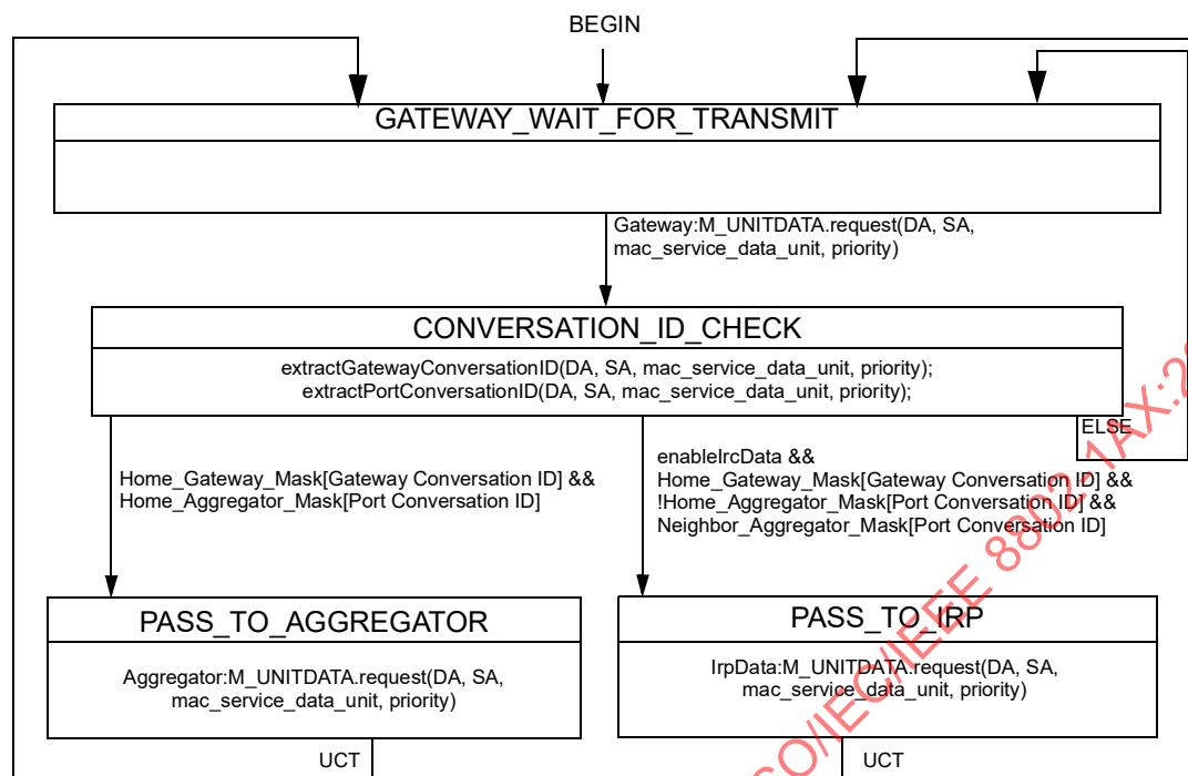
Figure 9-8—DR_Gateway state machine
