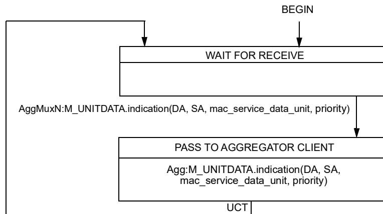
Figure 6-4—Frame Collector state diagram
