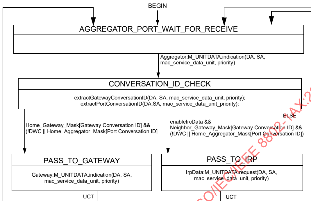
Figure 9-9—DR_Aggregator state machine
