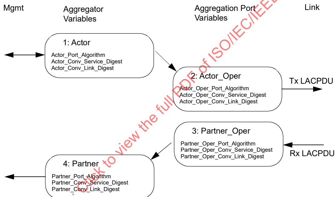
Figure 6-22—Distribution algorithm information flow
