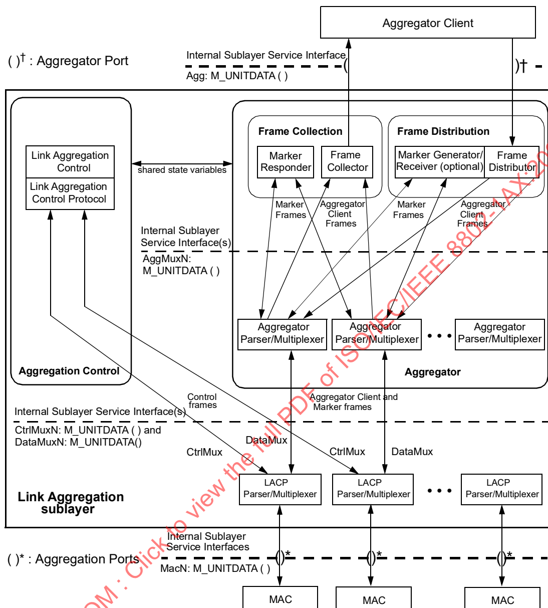
Figure 6-3—Link Aggregation sublayer block diagram
