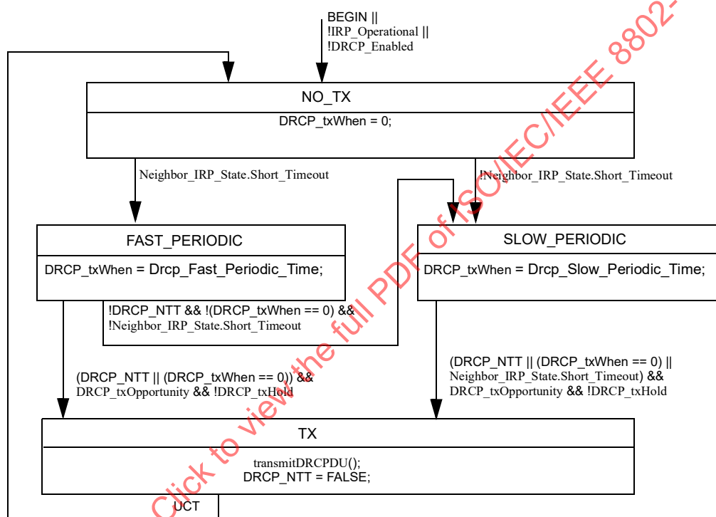
Figure 9-23—DRCP Transmit state diagram
