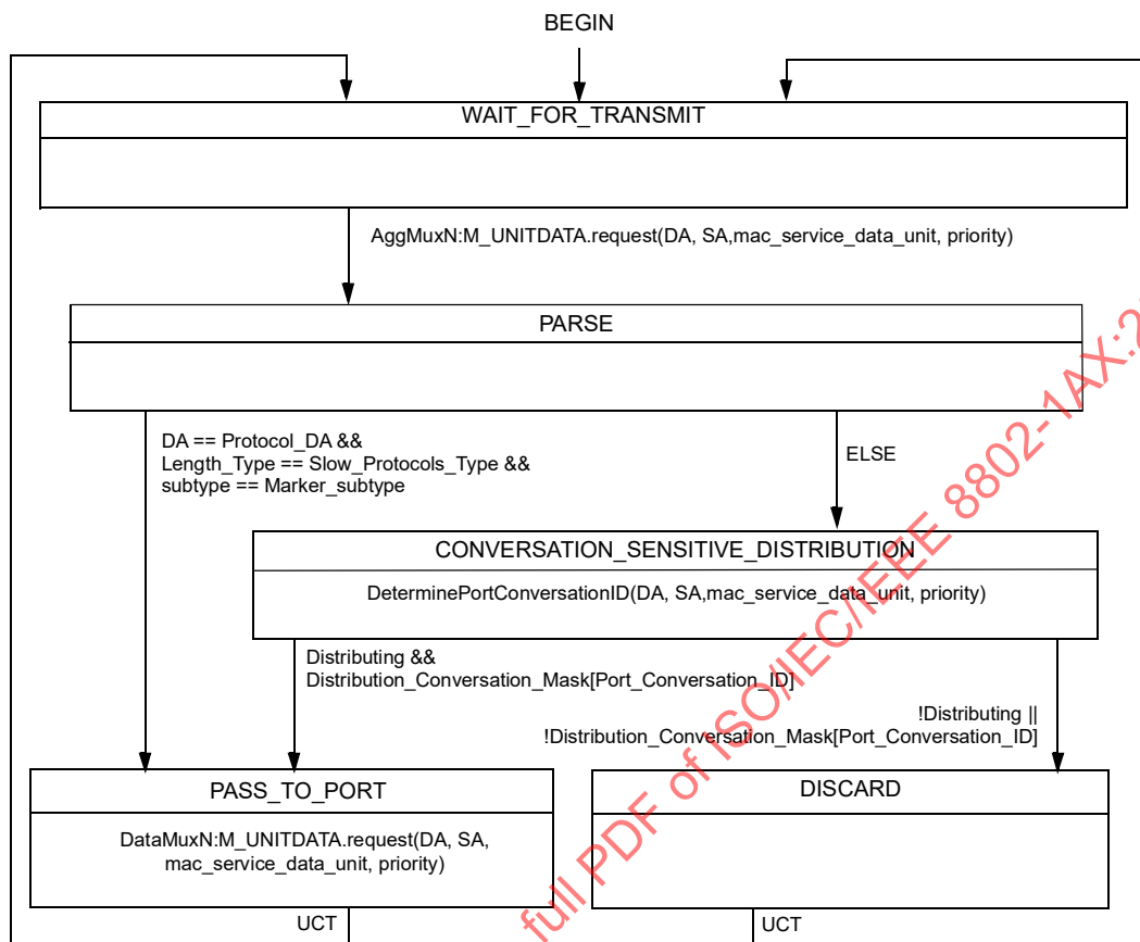
Figure 6-7—Aggregator Multiplexer state diagram
