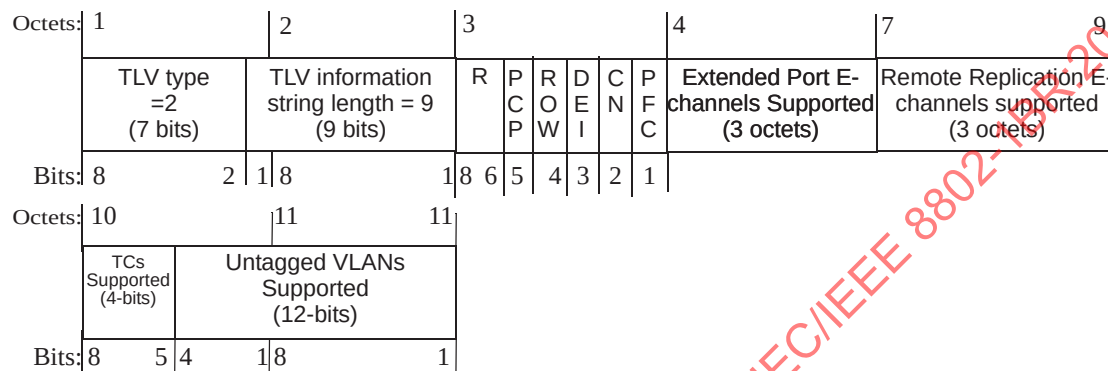
Figure 9-7—Resource Limit Capability TLV
