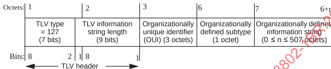
Figure 9-17—Basic format for Organizationally Specific TLVs
