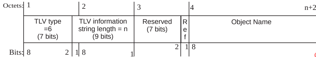
Figure 9-14—Object Name TLV
