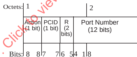
Figure 9-9—Port Entry
