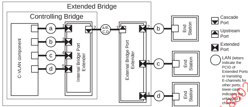
Figure 8-2—Extended Bridge Interconnection
