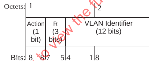
Figure 9-11—VID Entry
