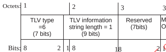
Figure 9-12—Port Status TLV
