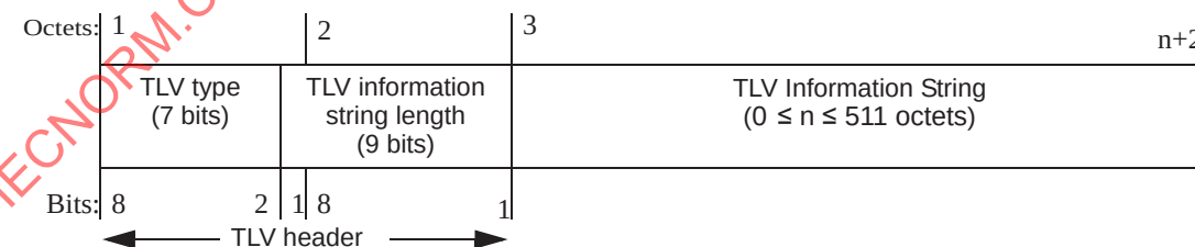
Figure 9-5—Basic TLV format
