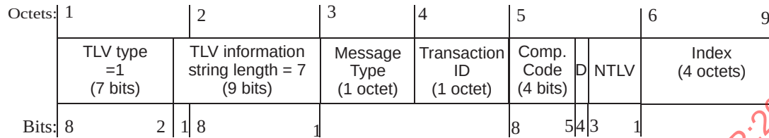
Figure 9-6—Command TLV
