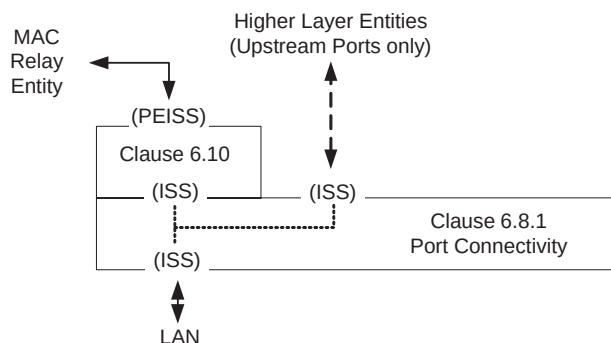
Figure 6-7—Port connectivity
