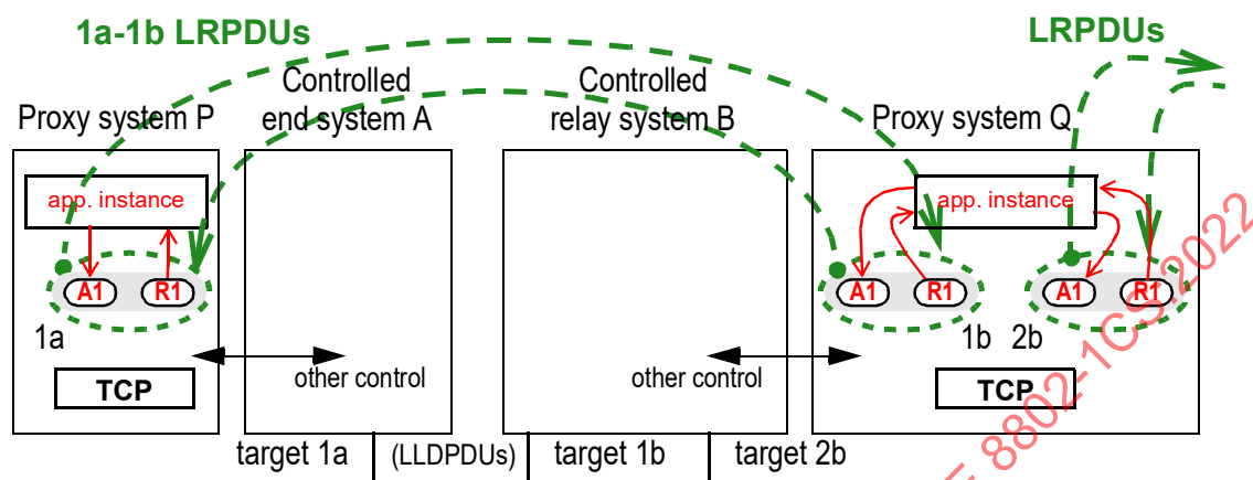
Figure 6-5—Controlled end and relay systems
