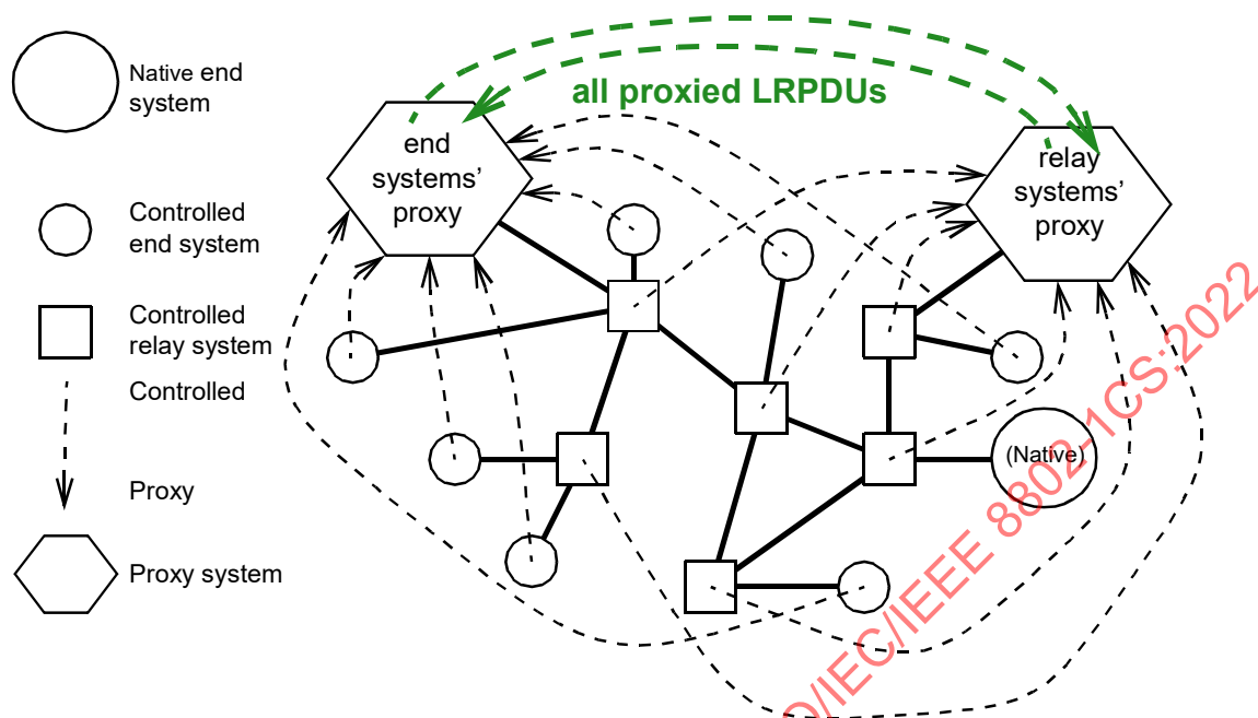
Figure 6-6—Communicating Proxy systems
