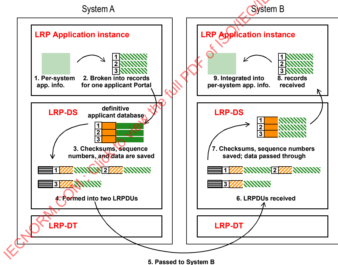
Figure 6-7—LRP-DS data path
