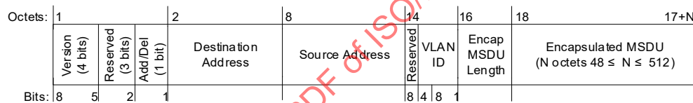
Figure 49-6—CIM PDU
