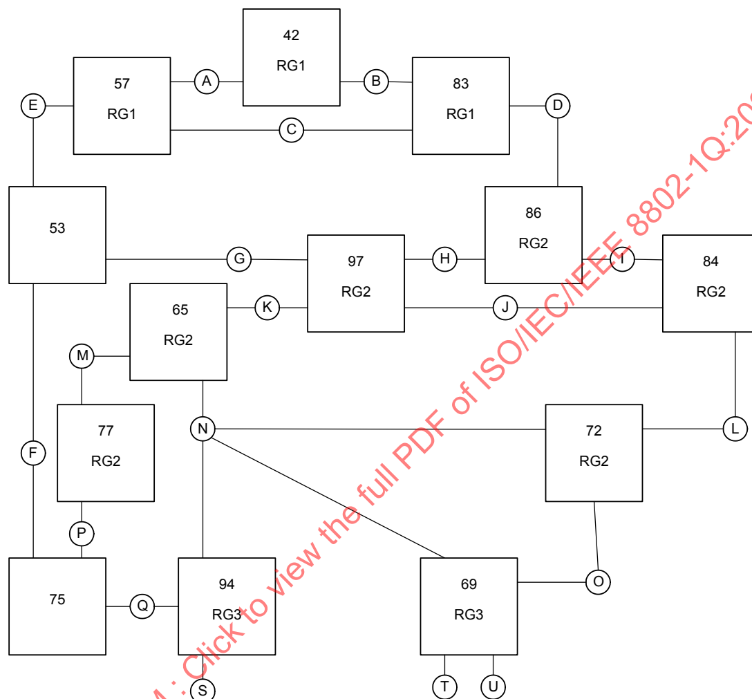
Figure 13-6—An MST Bridge network
