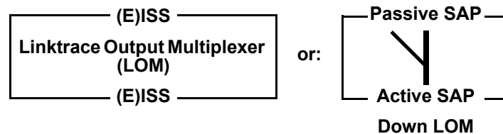
Figure 19-4—LOM shim
