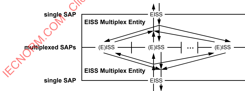
Figure 6-6—Two back-to-back EISS Multiplex Entities
