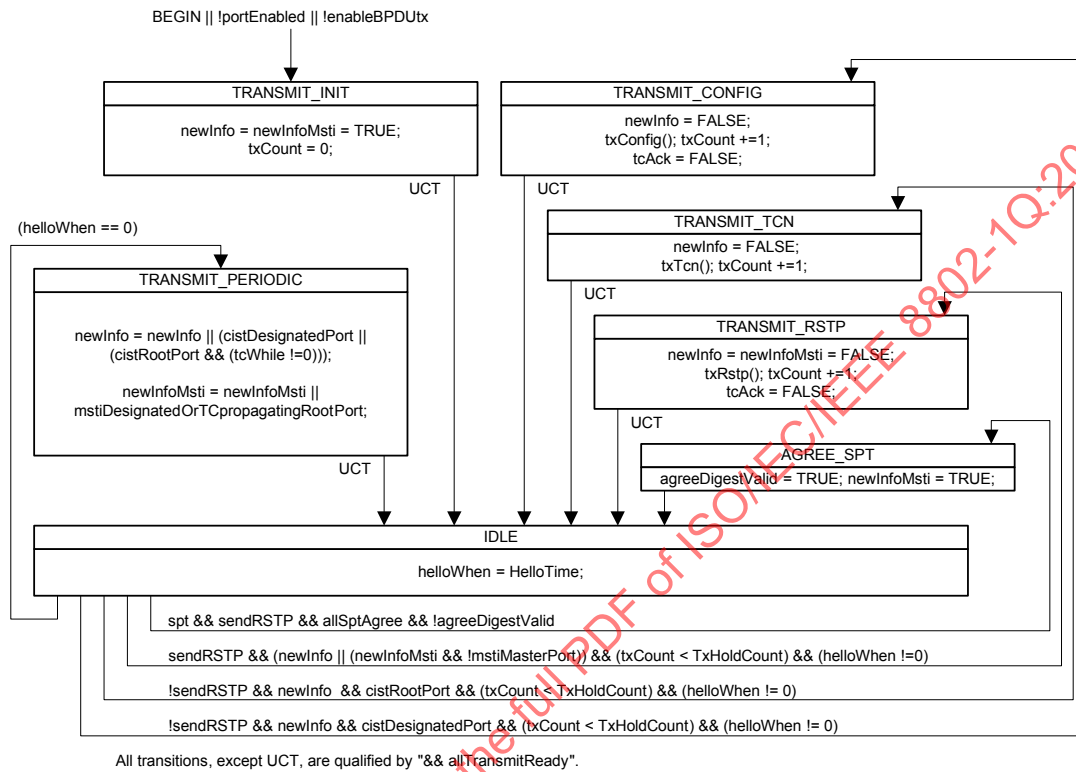
Figure 13-19—Port Transmit state machine
