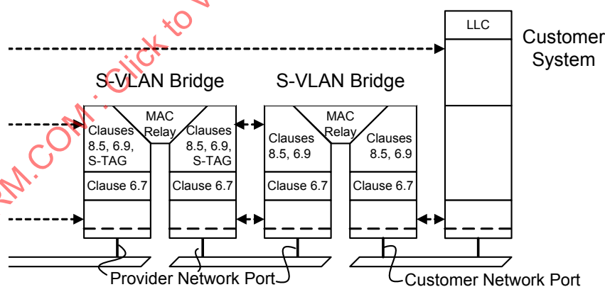
Figure 15-2—Port-based service interface to a PBN
