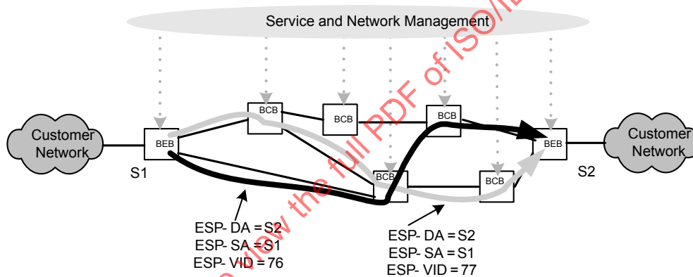
Figure 25-14—PBB-TE Region
