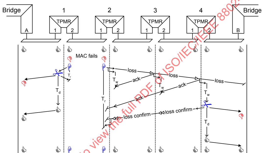
Figure 23-5—Losing connectivity
