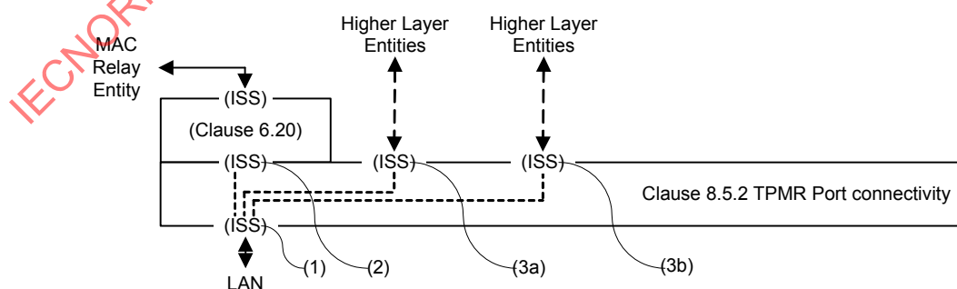
Figure 8-11—TPMR Port Transmit and Receive
