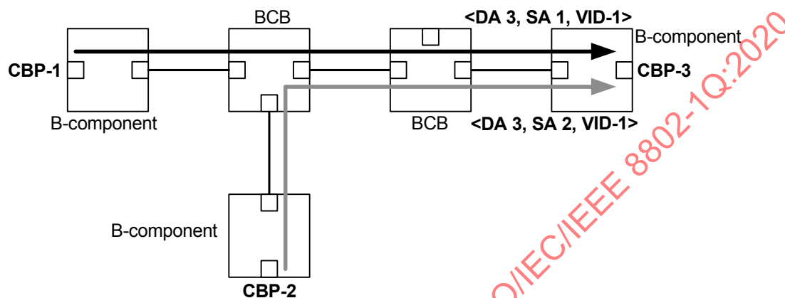
Figure 26-7—Independent ESPs using the same ESP-DAs and ESP-VIDs
