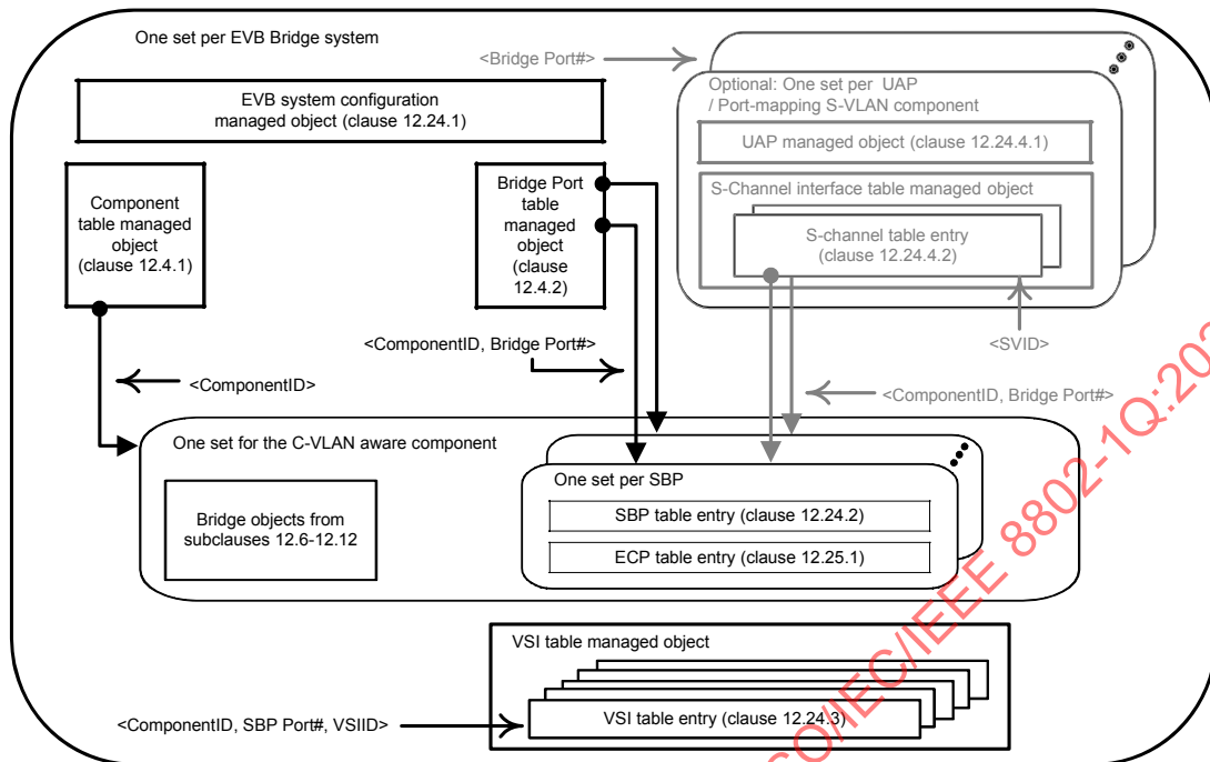
Figure 12-4—Relationships among EVB Bridge managed objects
