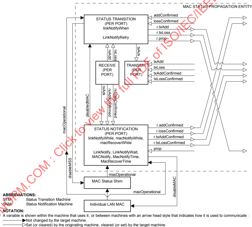
Figure 23-9—MSPE state machine overview
