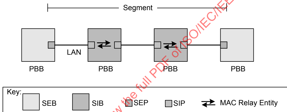
Figure 26-18—Segment terminology and properties
