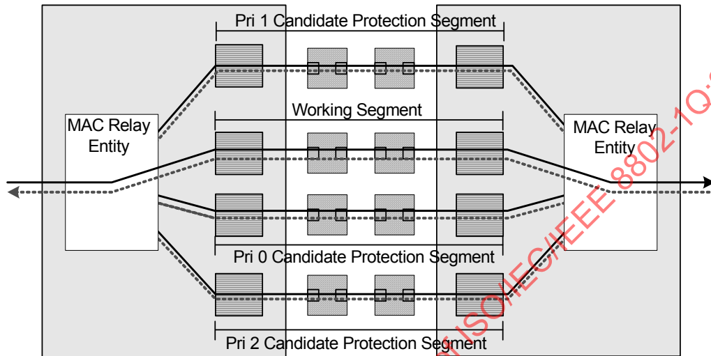
Figure 26-23—M:1 IPS
