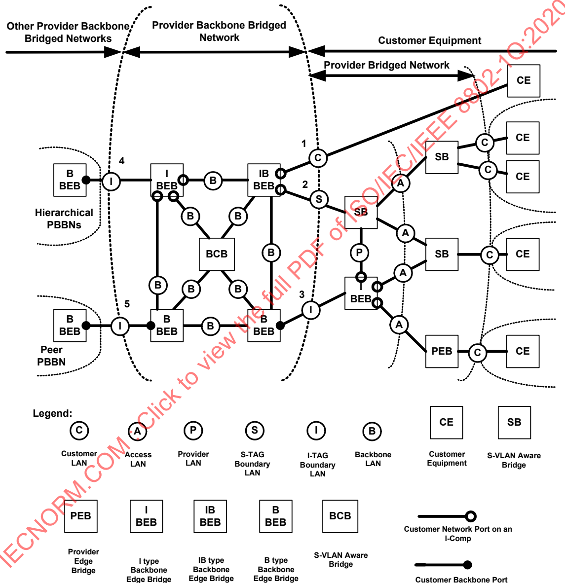
Figure 26-1—PBBN example
