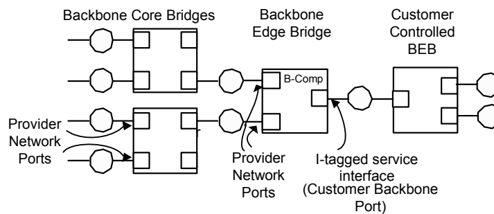
Figure 25-10—I-tagged service interface equipment
