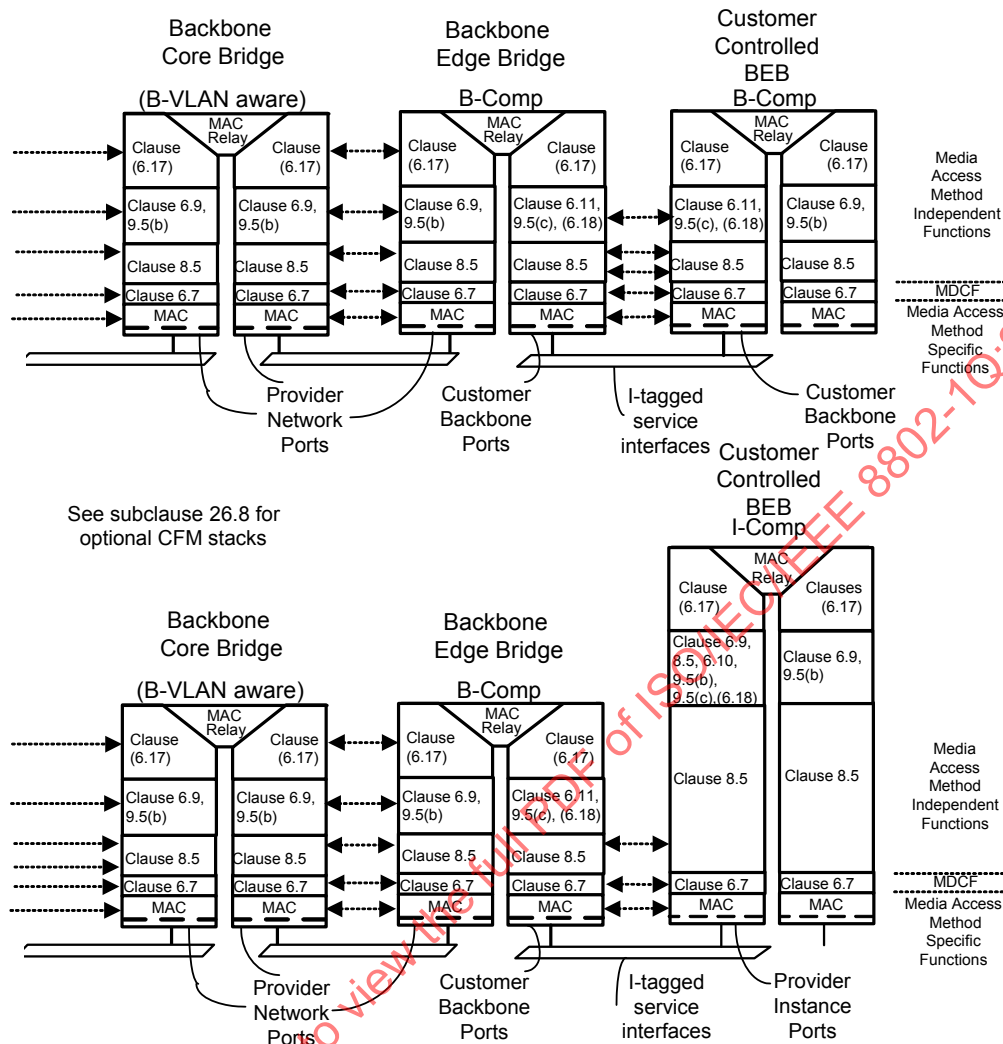
Figure 25-9—I-tagged service interface
