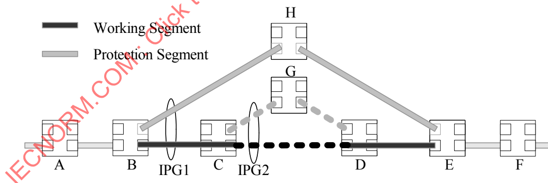
Figure 26-21—Nested IPGs
