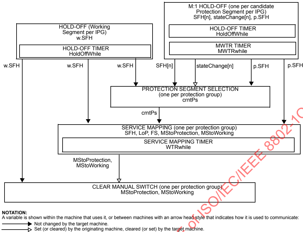
Figure 26-24—M:1 IPS state machines
