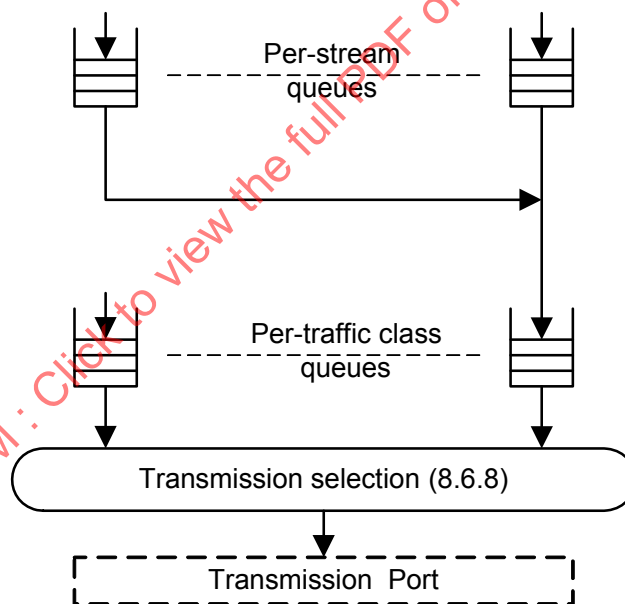
Figure 34-1—Queuing model for a Talker station
