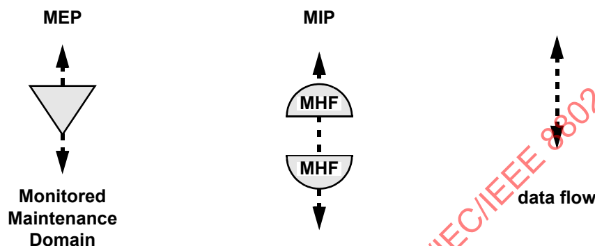
Figure 18-4—MEP and MIP Symbols
