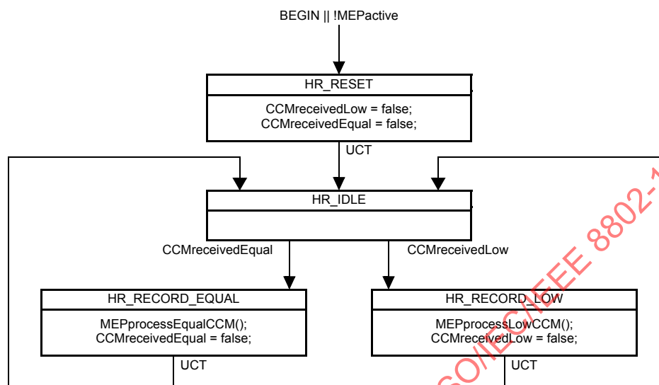
Figure 20-4—MEP Continuity Check Receiver state machine
