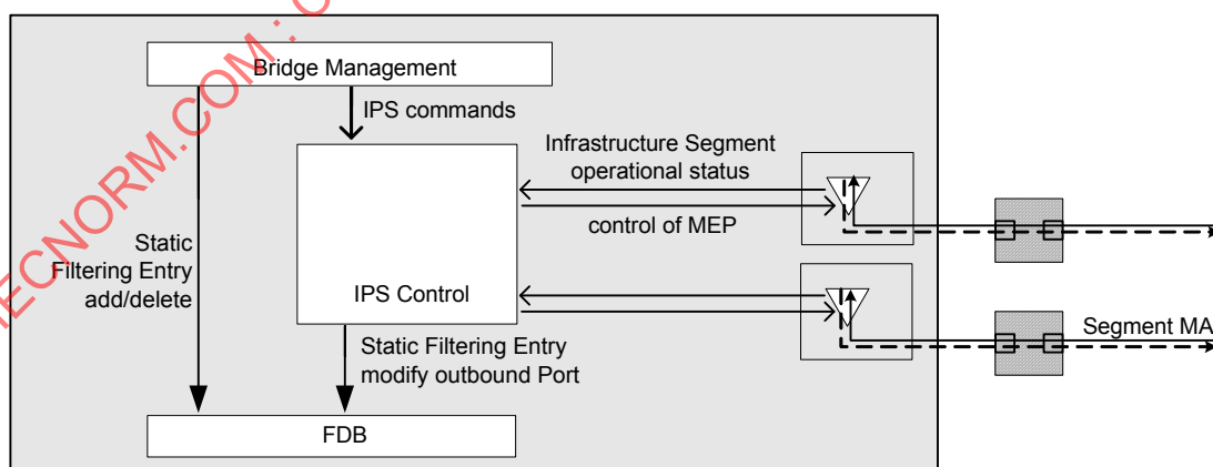
Figure 26-22—IPS Control entity
