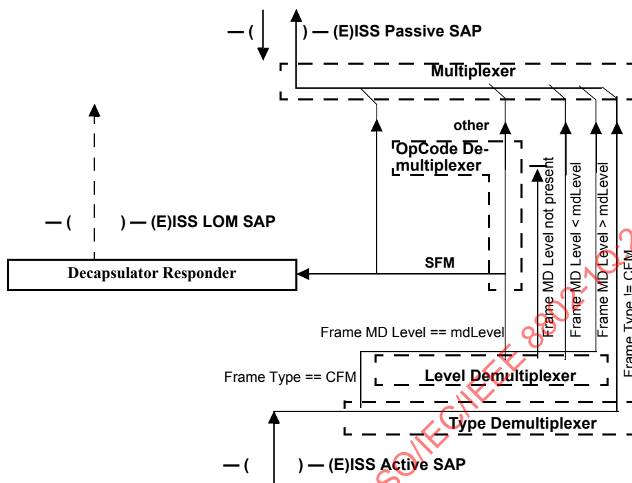
Figure 29-6—Return Path DR
