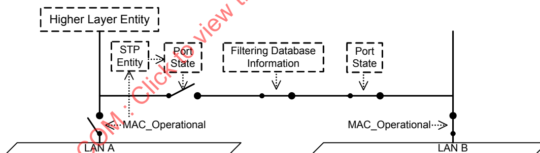
Figure 8-24—Effect of Port State
