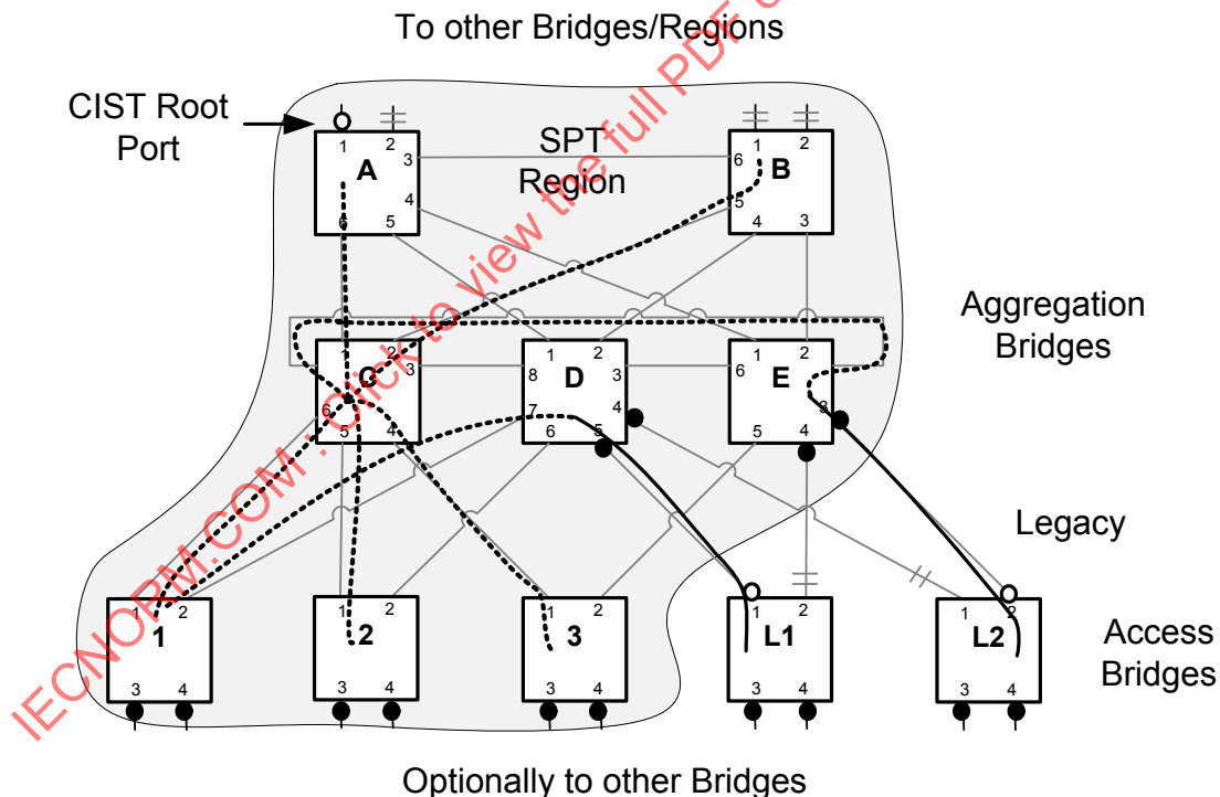
Figure 27-6—SPBV campus network example
