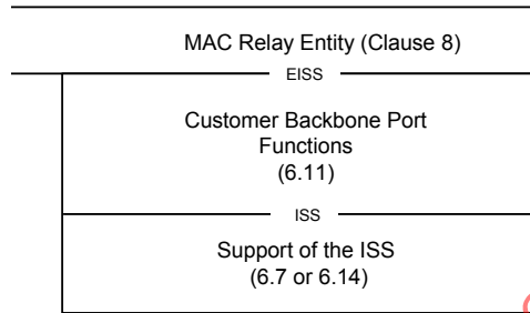
Figure 6-3—B-Component CBP
