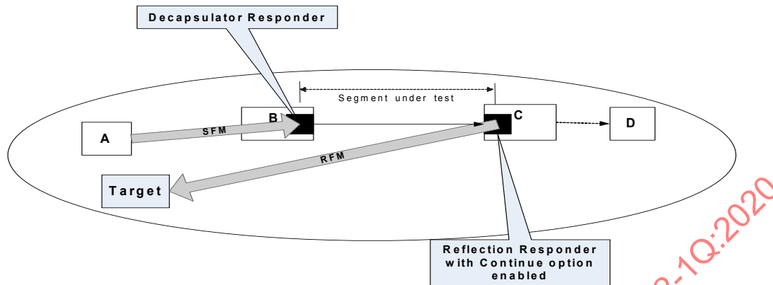
Figure 29-3—Combination of FPT and RPT
