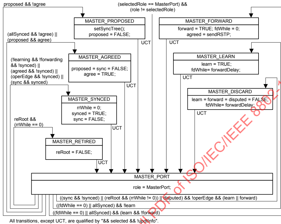
Figure 13-23—Port Role Transitions state machine—MasterPort
