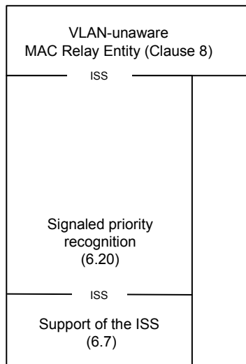
Figure 6-10—Supporting the ISS with signaled priority
