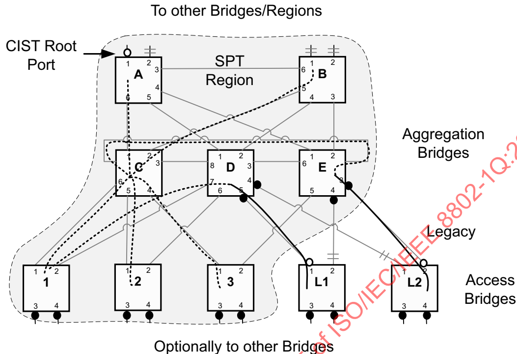
Figure 27-6—SPBV campus network example
