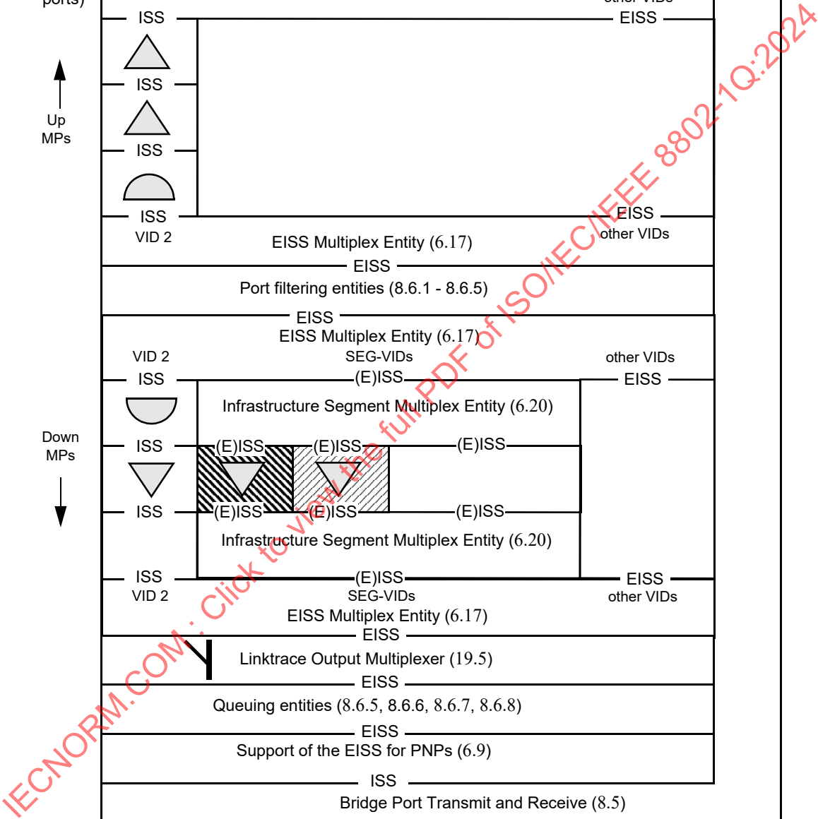
Figure 26-10—Infrastructure Segment MEP placement in a PNP
