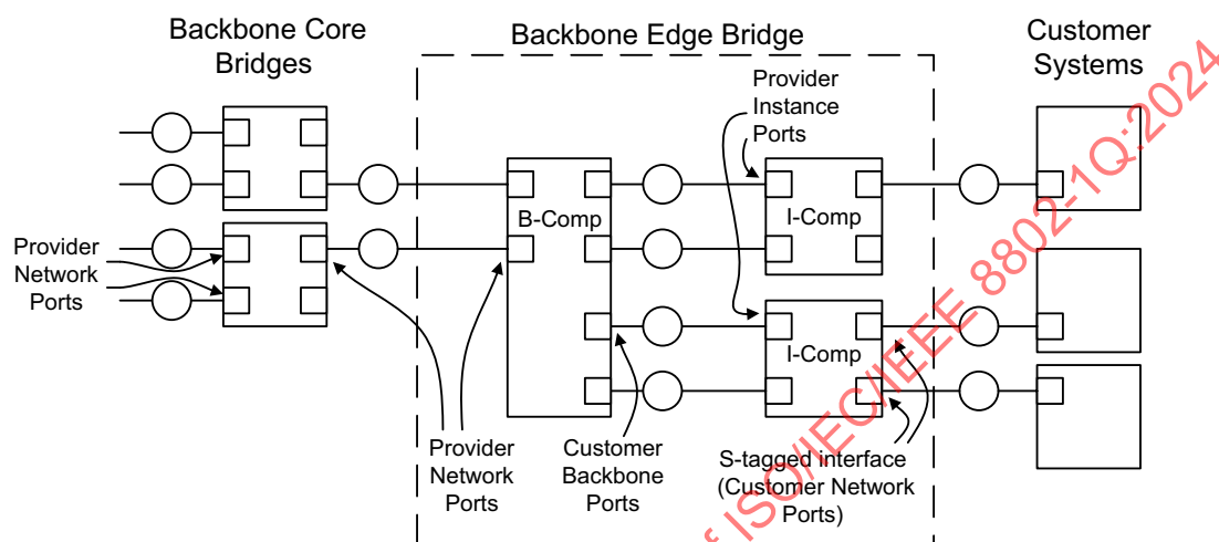
Figure 25-8—S-tagged service interface equipment
