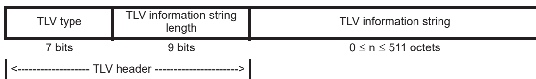
Figure 11-19—EAPOL-Announcement TLV format
