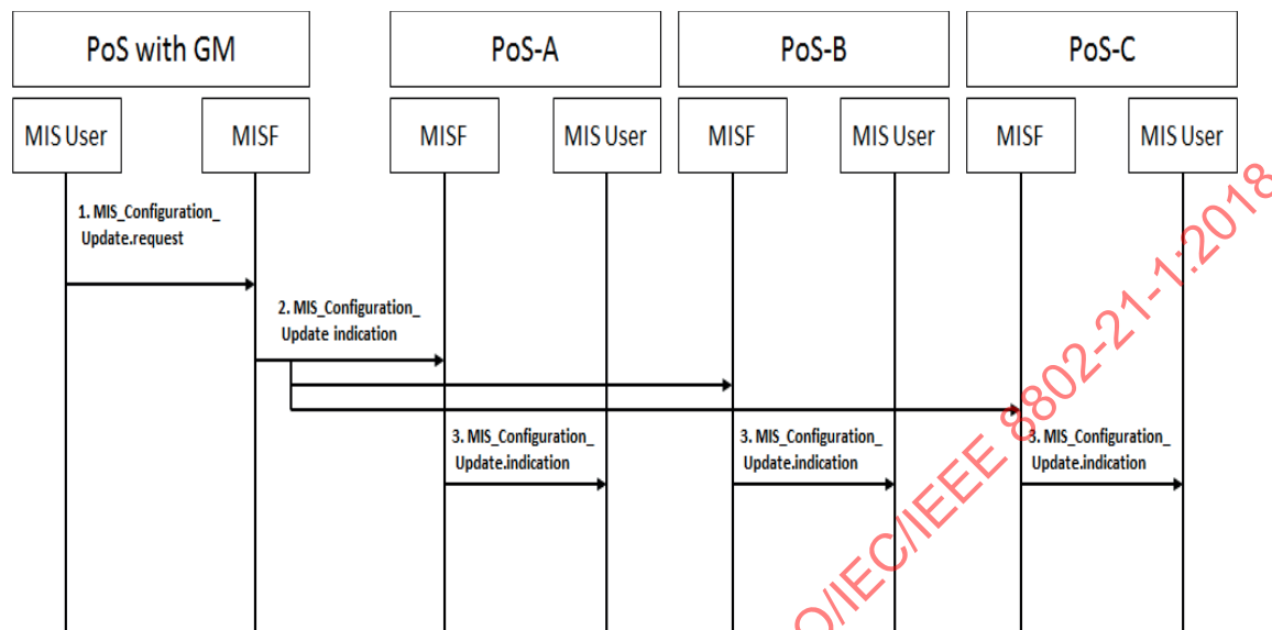
Figure 19—Transmission of the control command
