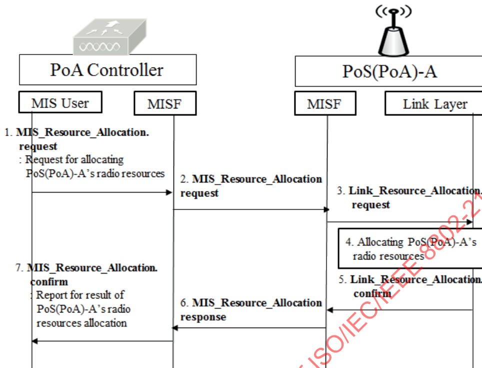
Figure 39—PoA controller allocates radio resources for PoS(PoA)
