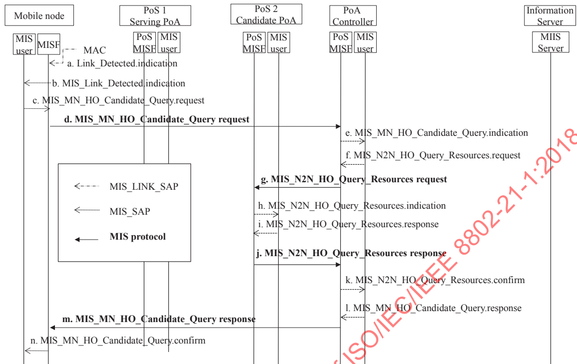
Figure 14—Signaling flows for handover preparation procedure
