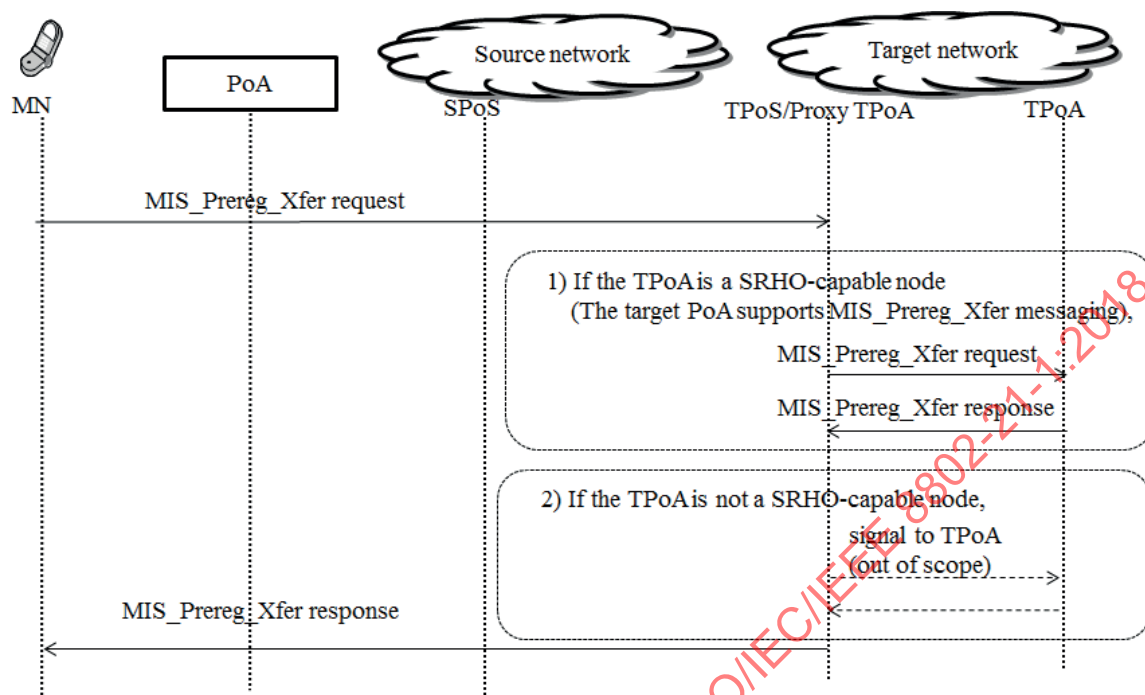
Figure 7—Communication between the MN and the TPoA
