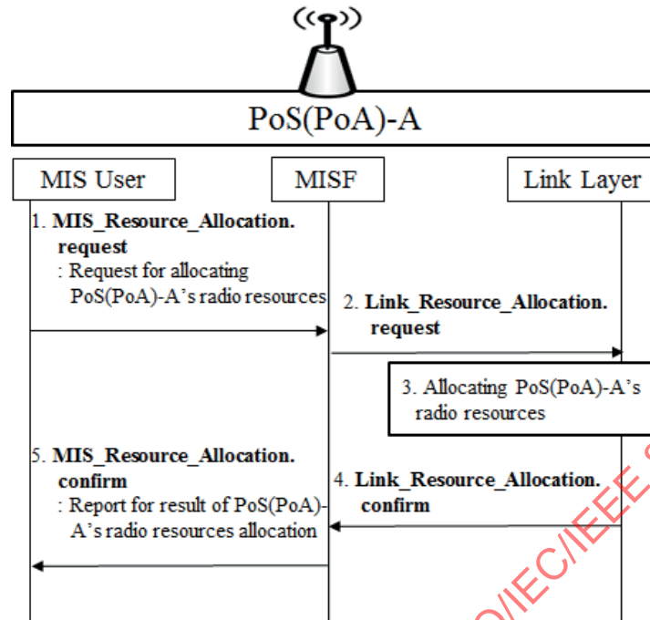
Figure 38 —PoS(PoA) allocates its own radio resources
