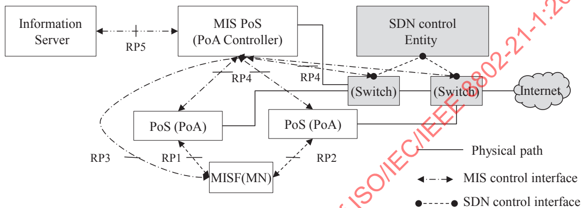
Figure 10—MIS communication model for SDRAN
