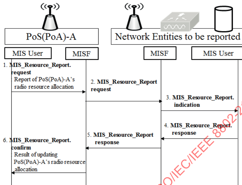
Figure 40—PoS(PoA) reports its updated radio resources to other network entities
