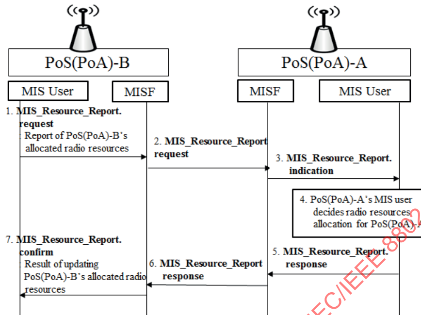
Figure 31—PoS(PoA)-A decides its radio resource allocation based on radio resource allocation reports of PoS(PoA)-B
