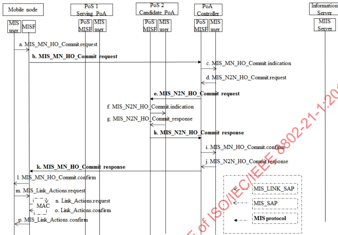
Figure 15—Signaling flows for handover decision procedure
