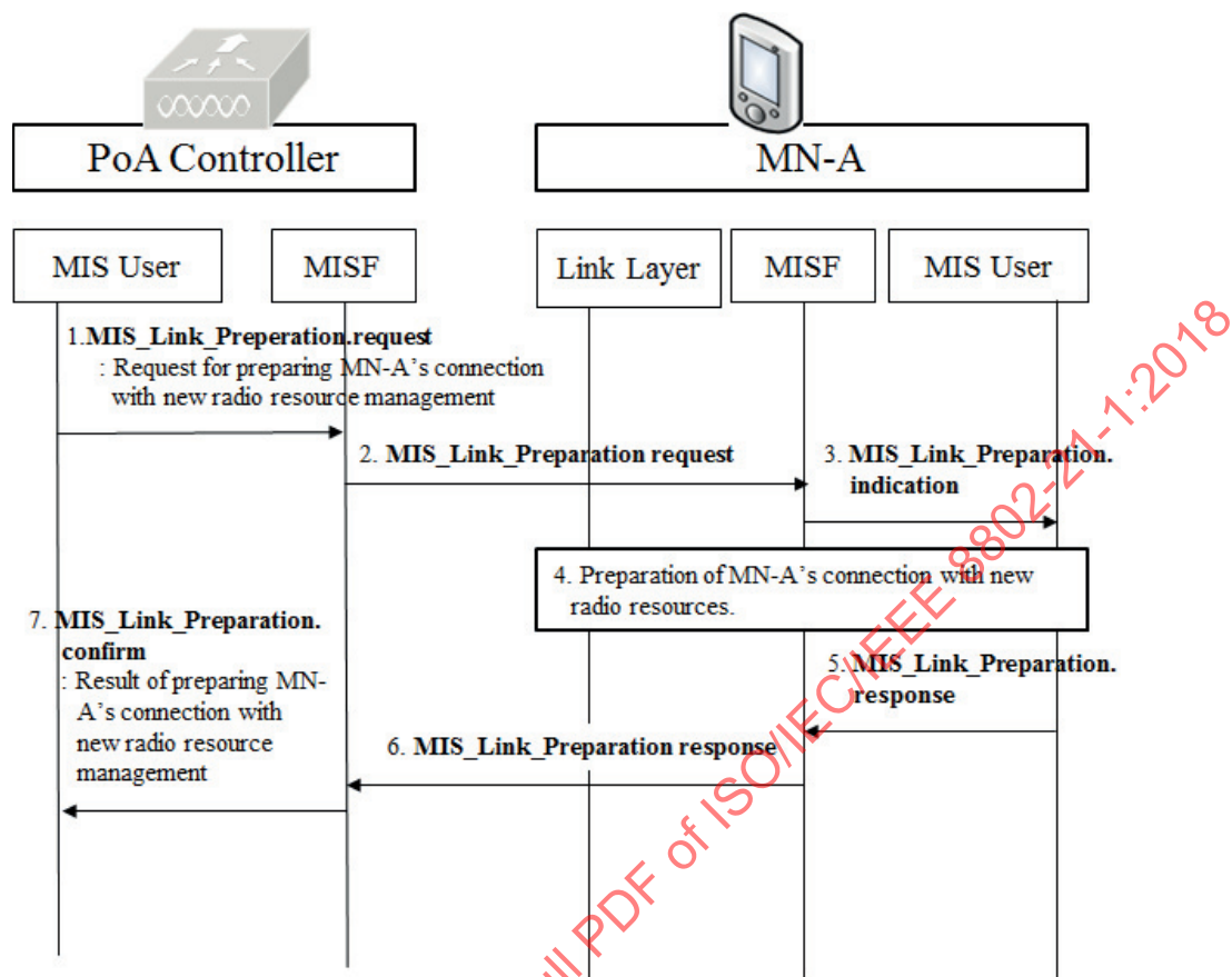
Figure 37—PoA controller requests MN-A to prepare connection with newly allocated radio resources
