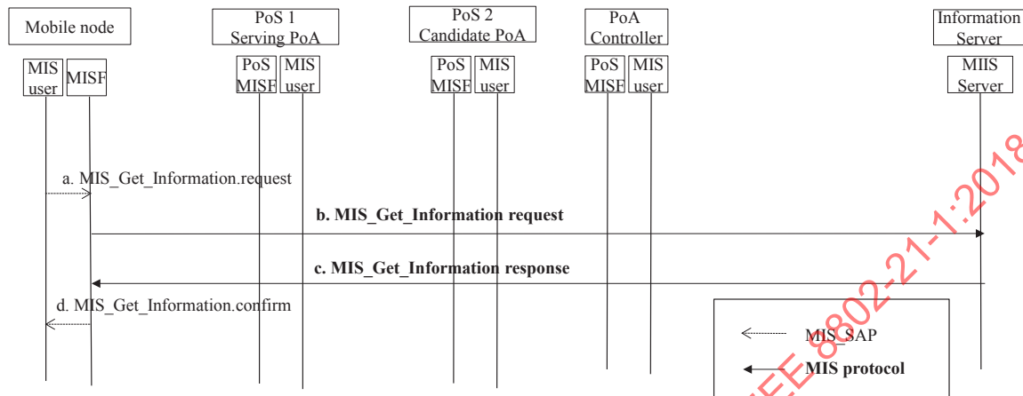
Figure 13—Signaling flows for handover initiation procedure
