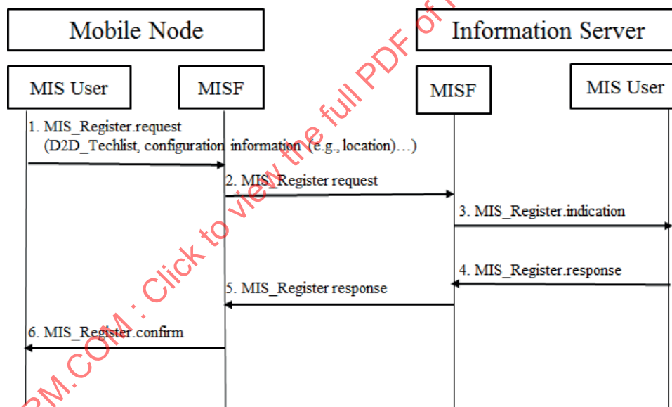
Figure 43—Registration of D2D devices with list of D2D technologies
