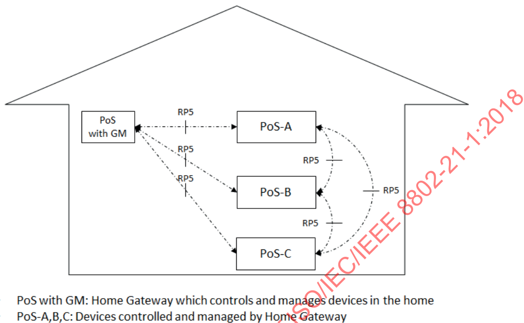
Figure 18—MIS reference model for HEMS use case
