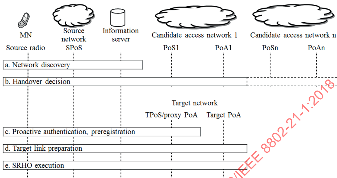
Figure 3—Single-radio handover procedures
