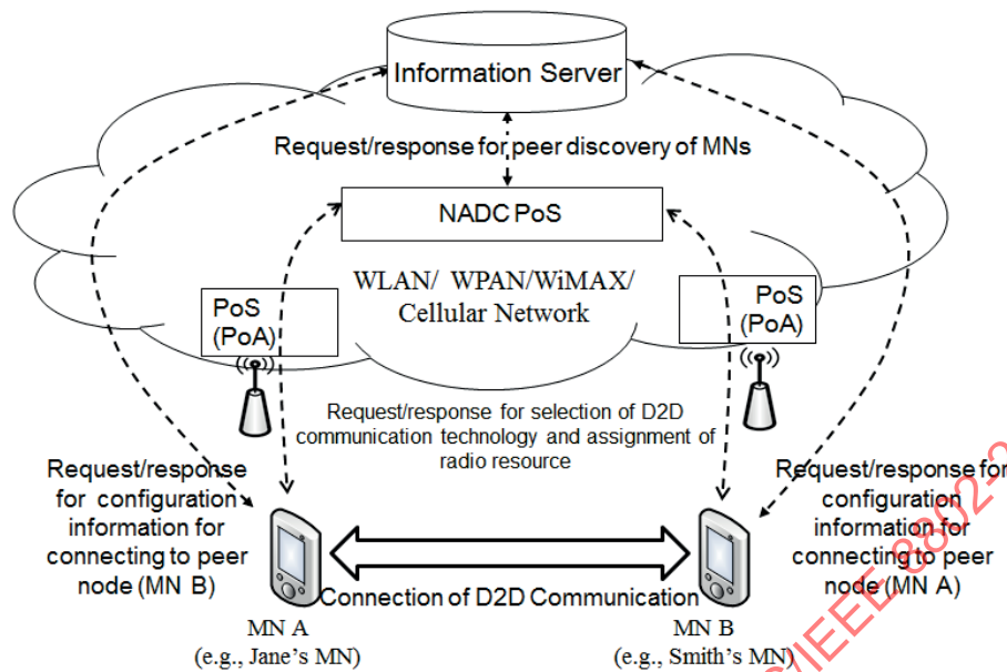
Figure 41—Control signaling of NADC
