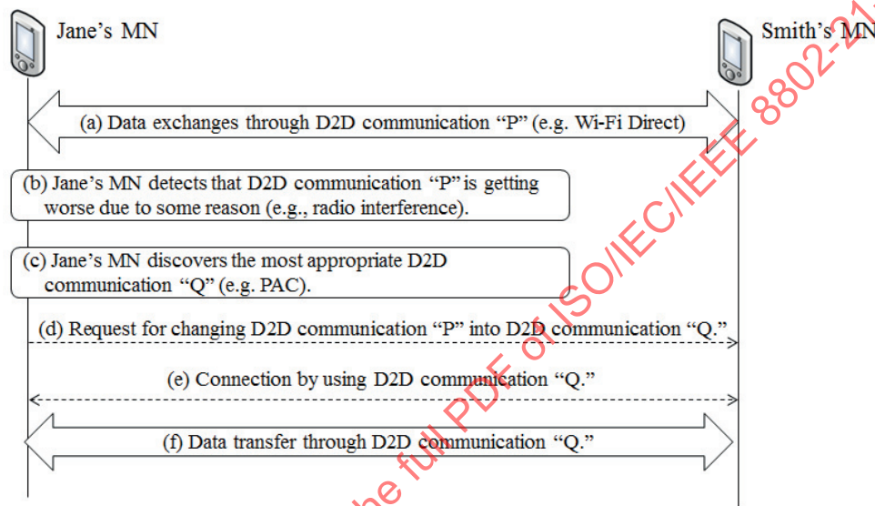
Figure 46—Control signaling of D2D communication without network assistance
