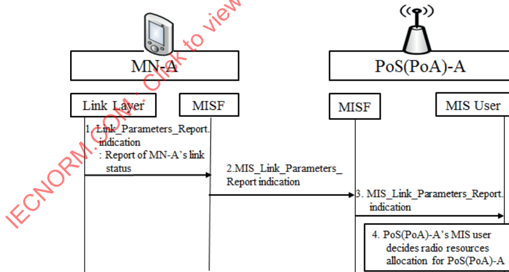
Figure 29—PoS(PoA)-A decides its radio resource allocation based on link status of MN
