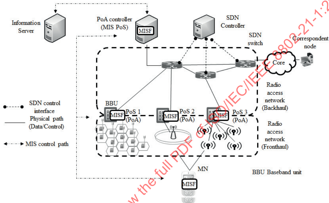
Figure 9—MIS framework architecture for SDRANs
