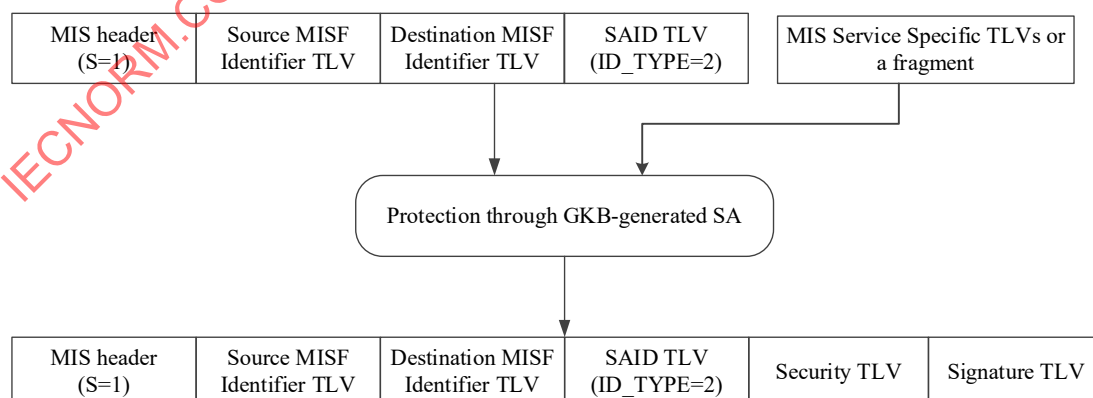
Figure 34—MIS PDU protected by a GKB-generated MIS SA with a signature TLV
