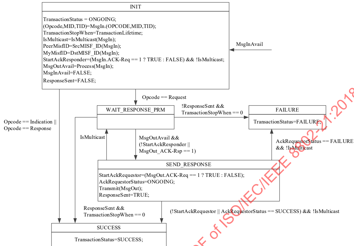
Figure 24—Transaction destination state machine
