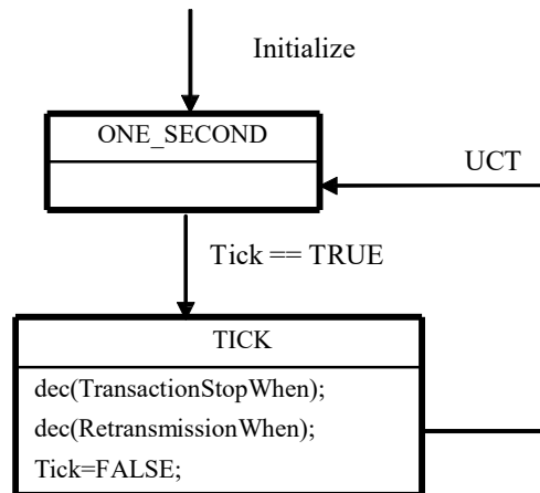
Figure 22—Transaction timers state machine
