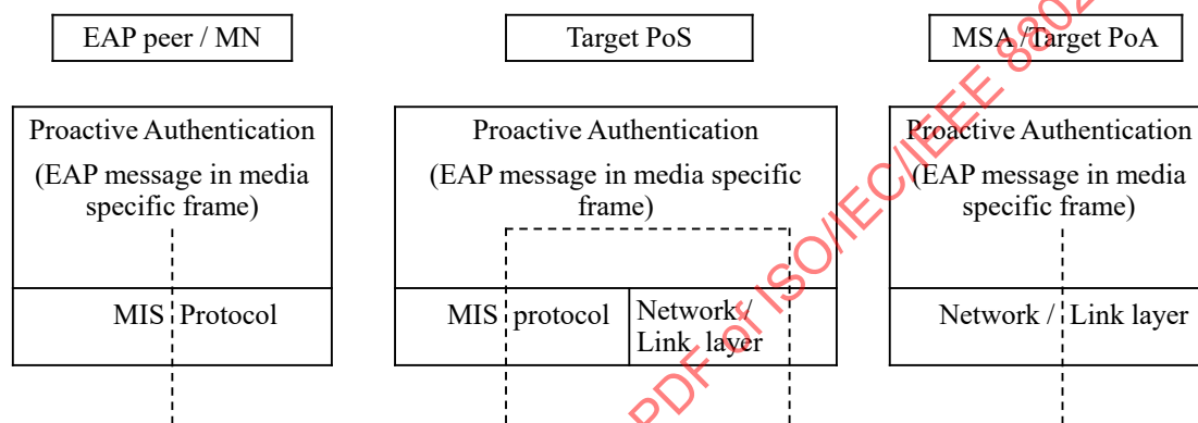
Figure 80—Protocol stack for MIS supported proactive authentication
