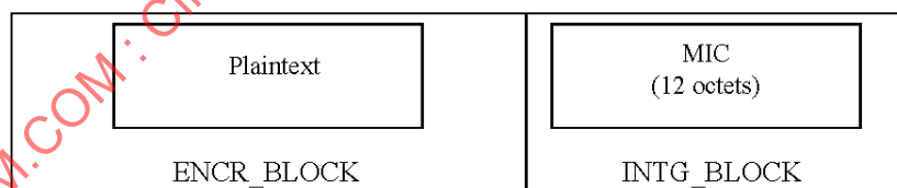
Figure 54—Security TLV for AES-CMAC
