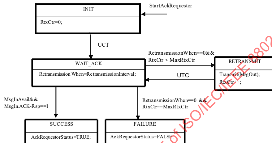
Figure 25—ACK requestor state machine
