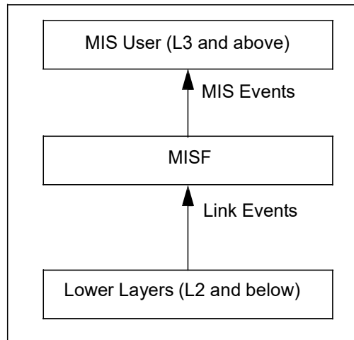
Figure 12—Link events and MIS events
