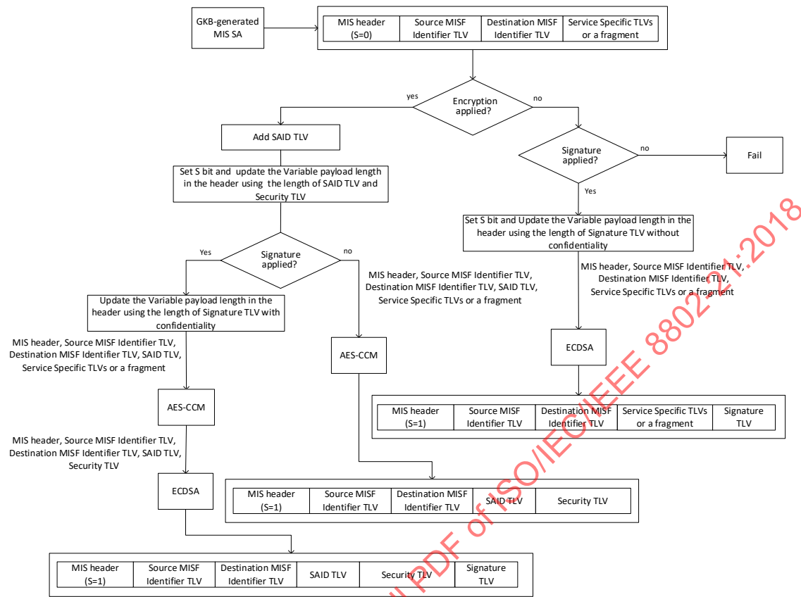
Figure 74—MIS PDU protection procedure with the GKB-generated MIS SA
