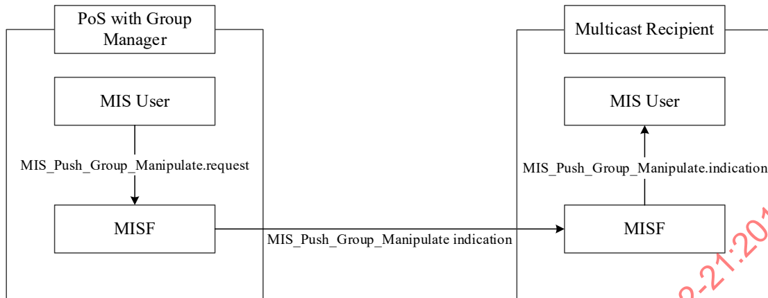
Figure 67—Example of group manipulation distribution using multicast mechanisms
