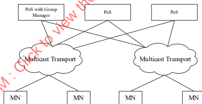
Figure 2—Group communication functional entities
