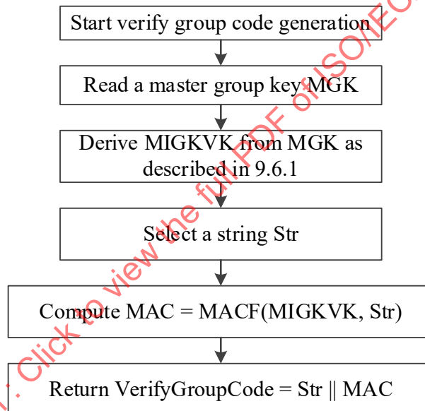
Figure 59—Flow diagram of the verify group code generation
