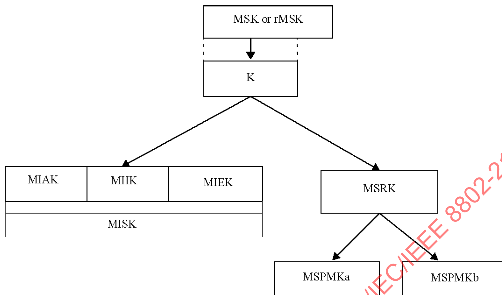
Figure 82—Key hierarchy for bundle case
