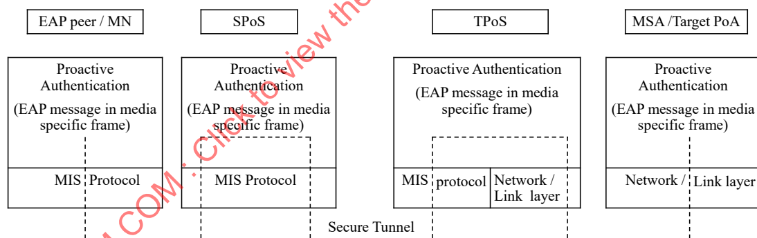
Figure 81—Protocol stack for MIS supported optimized pull key distribution with two points of service
