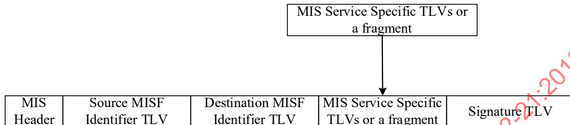
Figure 35—MIS PDU protected by digital signature only
