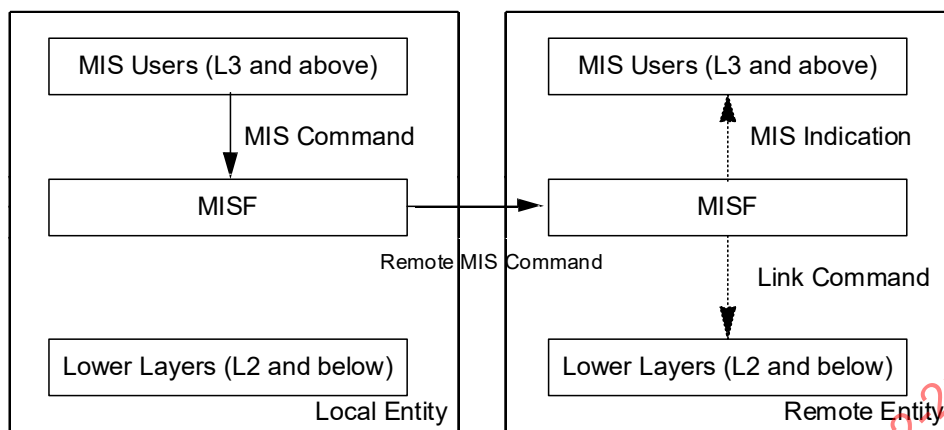
Figure 16—Remote MIS command
