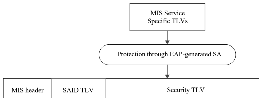
Figure 32—MIS PDU protected by an EAP-generated MIS SA
