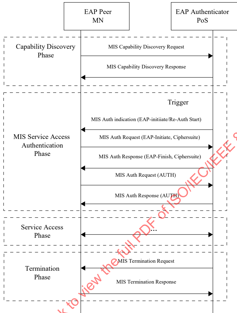
Figure 44—Main stages with PoS initiated ERP execution (1)
