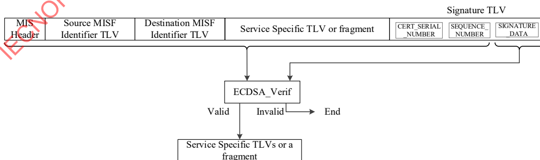
Figure 79—Signature verification without confidentiality
