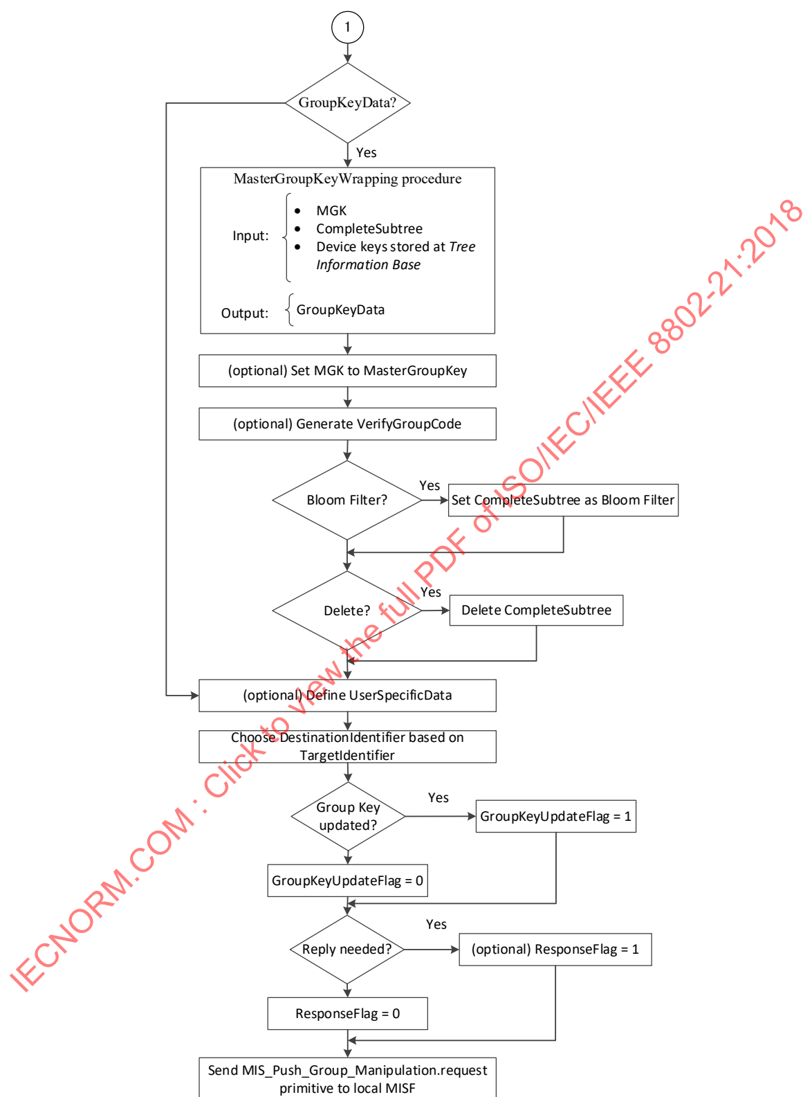
Figure 69—Summary of steps performed by MIS user of PoS with group manager (continued from Figure 68)
