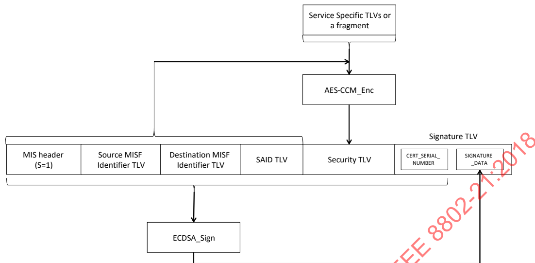
Figure 76—Signing with confidentiality
