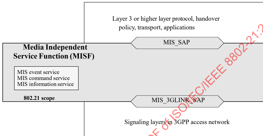
Figure 9—MIS reference model for 3GPP systems
