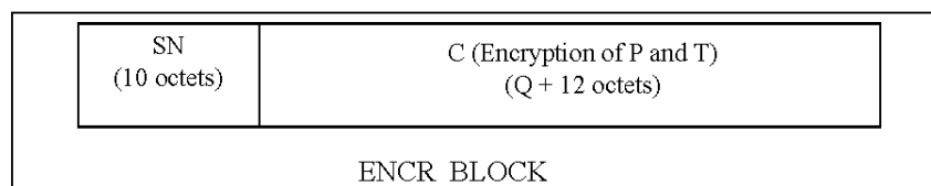
Figure 51—Security TLV for AES-CCM
