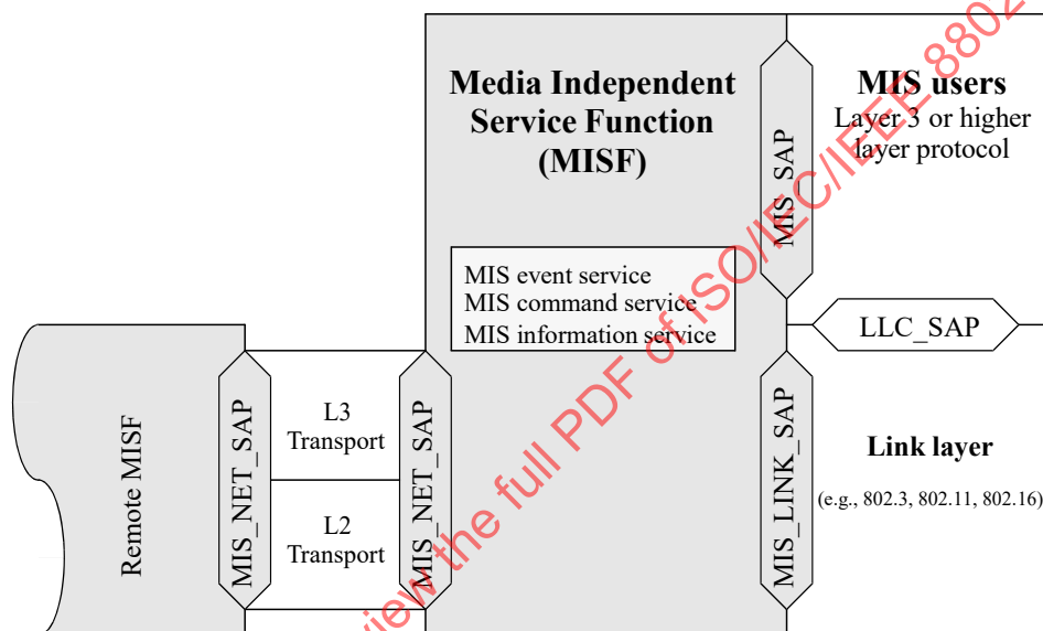
Figure 4—General MISF reference model and SAPs
