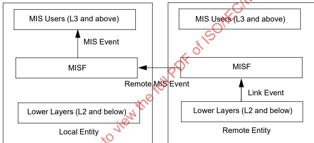
Figure 13—Remote MIS events
