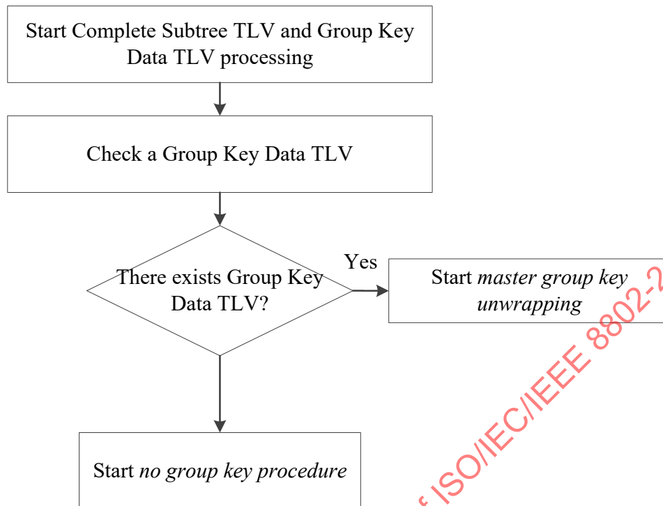
Figure 61—Selection of master group key unwrapping or no group key procedures
