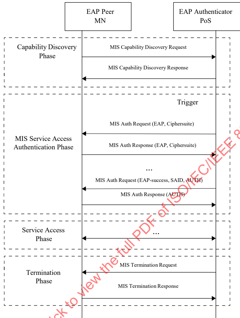
Figure 42—Main stages with PoS initiated EAP execution
