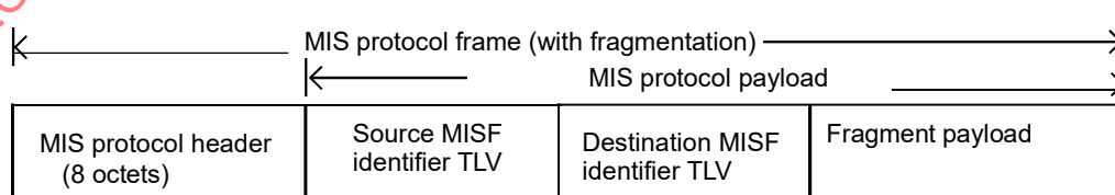
Figure 36—Fragmented MIS protocol frame format
