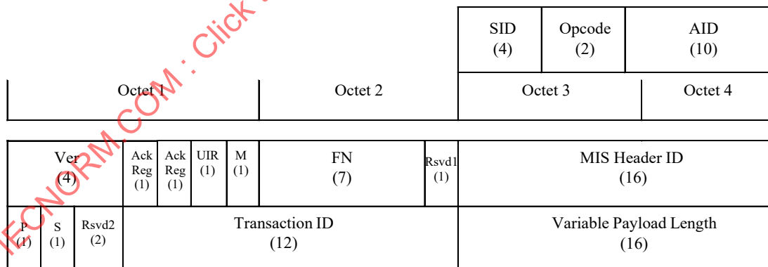
Figure 28—MIS protocol header format
