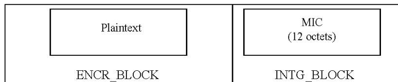
Figure 53—Security TLV for HMAC-SHA1-96
