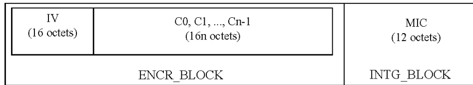
Figure 52—Security TLV for AES CBC and HMAC-SHA1-96
