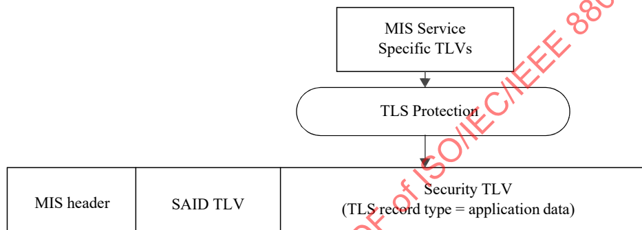
Figure 31—MIS PDU in existence of MIS SA by TLS
