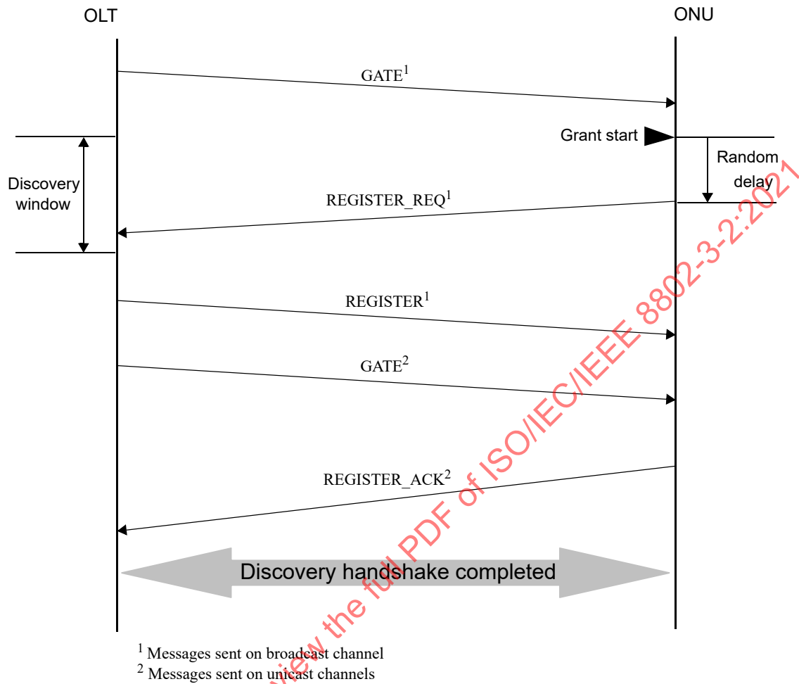
Figure 7-3—Discovery handshake message exchange
