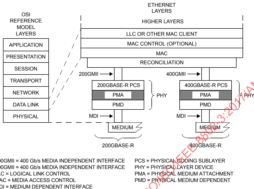
Figure 120-1—200GBASE-R and 400GBASE-R PMA relationship to the ISO/IEC Open Systems Interconnection (OSI) reference model and IEEE 802.3 Ethernet model
