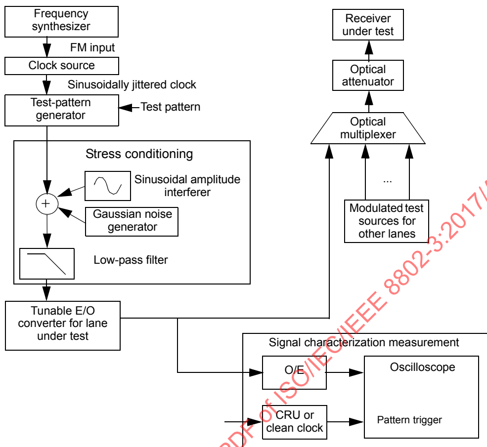
Figure 122-5—Stressed receiver conformance test block diagram
