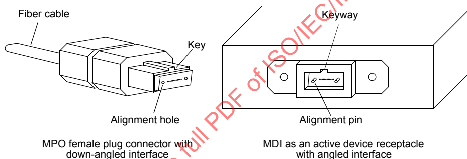
Figure 124-6—MPO female plug with down-angled interface and MDI active device receptacle with angled interface
