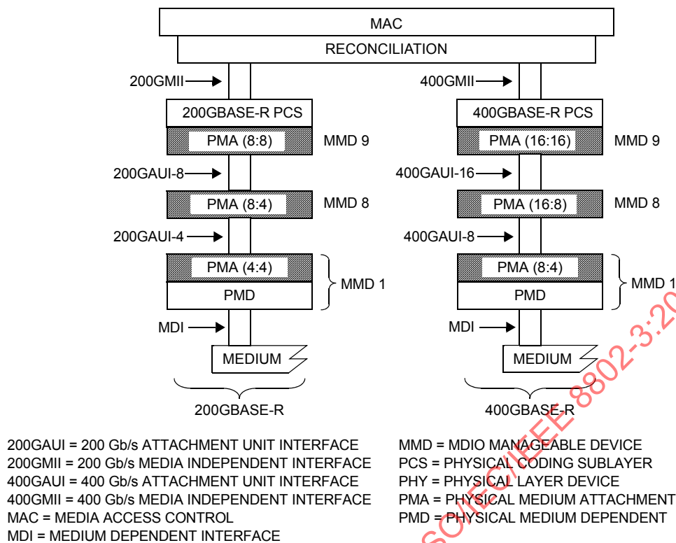
Figure 120-2—Example 200GBASE-R and 400GBASE-R PMA layering
