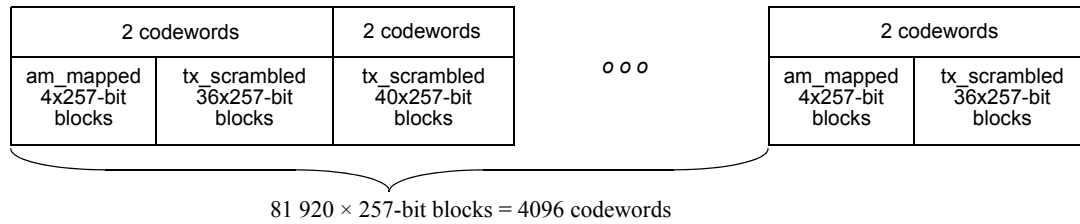
Figure 119–6—200GBASE-R alignment marker insertion period
