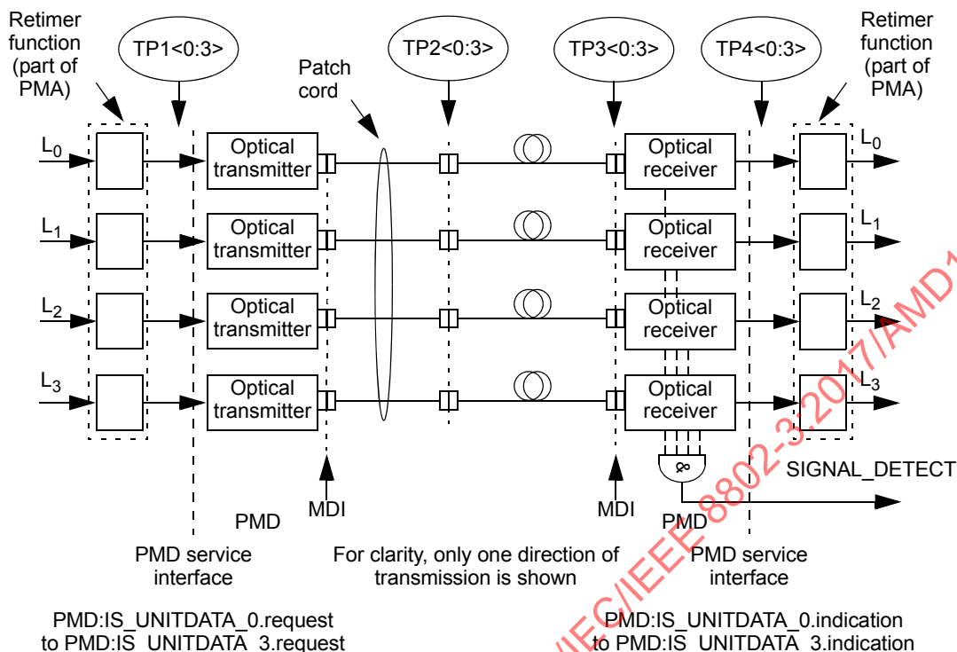
Figure 121-2—Block diagram for 200GBASE-DR4 transmit/receive paths
