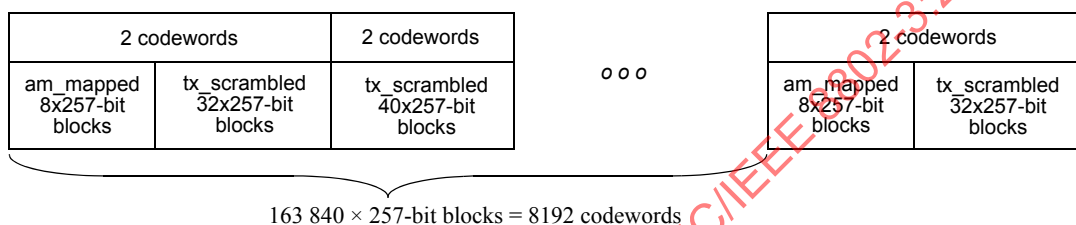
Figure 119–8—400GBASE-R alignment marker insertion period
