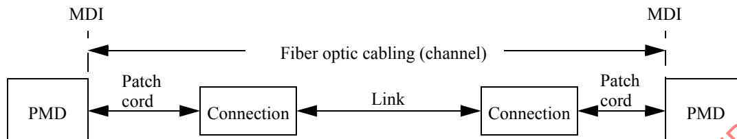
Figure 121–8—Fiber optic cabling model
