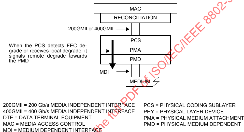
Figure 116–6—Remote Degrade signaling without Extender Sublayer
