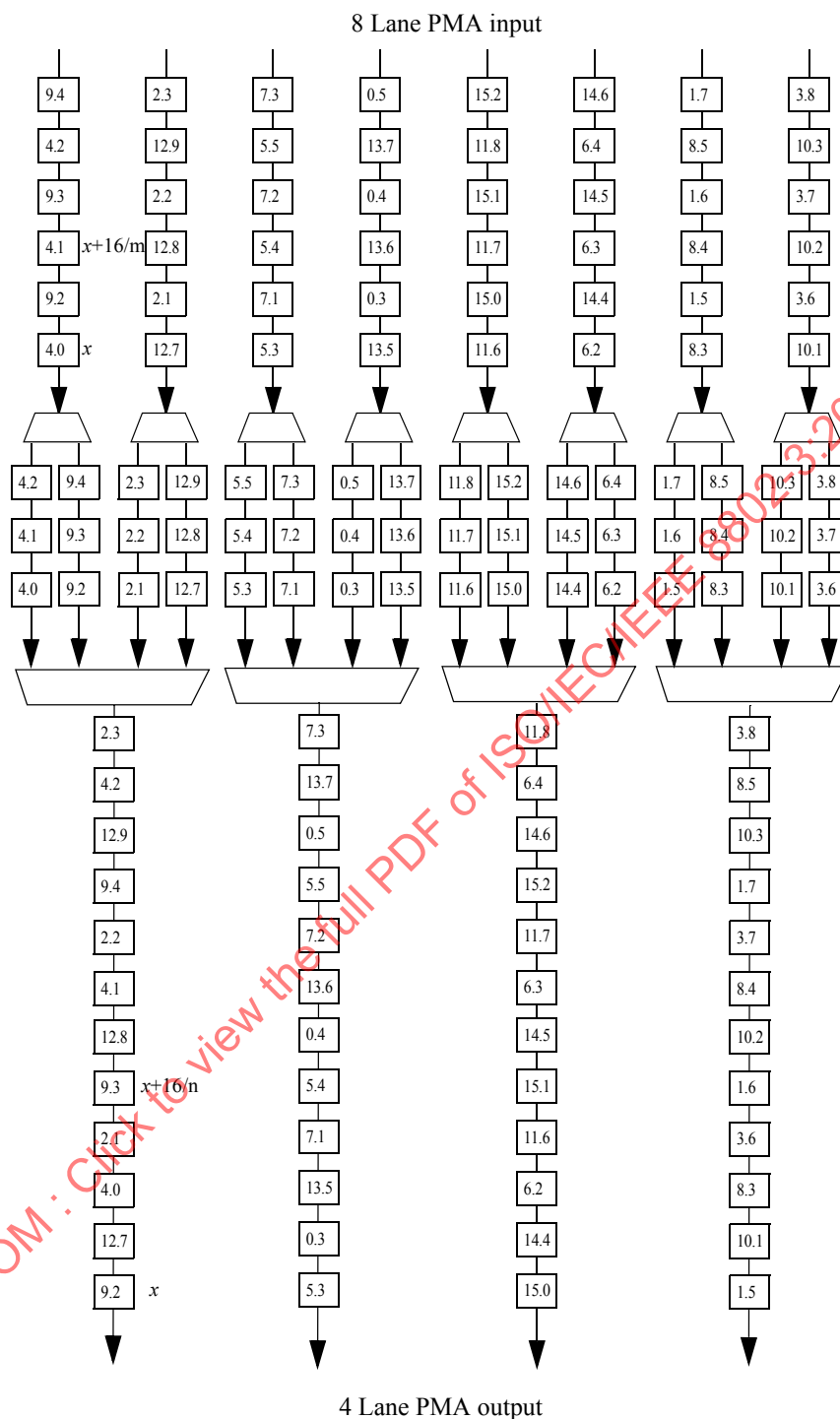
Figure 120–6—Example 8:4 400GBASE-R PMA bit mux
