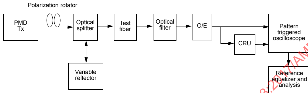
Figure 122–4—TDECQ conformance test block diagram
