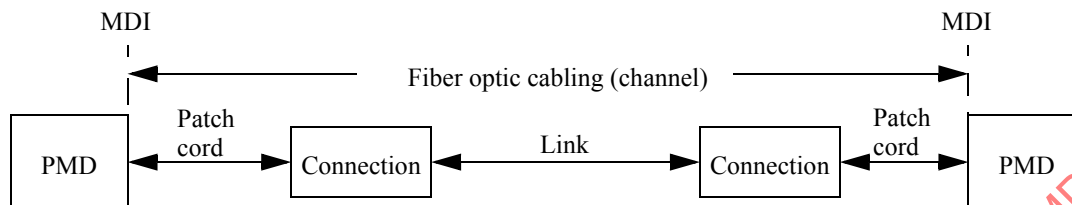
Figure 122–6—Fiber optic cabling model
