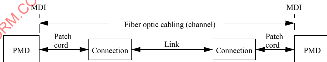
Figure 124-4—Fiber optic cabling model
