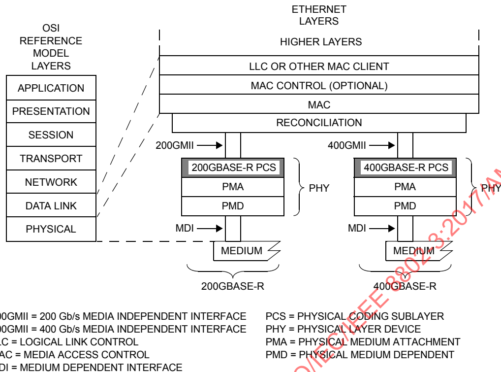
Figure 119-1—200GBASE-R and 400GBASE-R PCS relationship to the ISO/IEC Open Systems Interconnection (OSI) reference model and IEEE 802.3 Ethernet model
