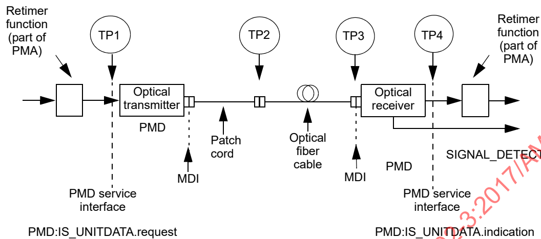
Figure 114-2—Block diagram for 25GBASE-LR and 25GBASE-ER transmit/receive paths
