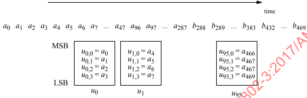
Figure 102–8—Downstream PHY Link mapping of FEC output to stream nibbles
