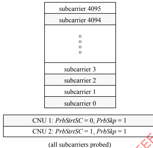
Figure 102–26—Scheduling two CNU in the same probing symbol
