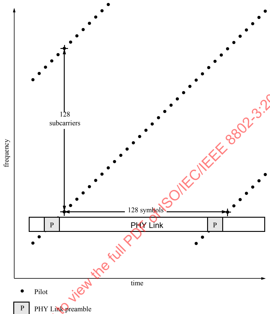
Figure 101-20—Downstream scattered pilot pattern
