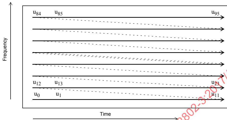
Figure 102-9—Downstream PHY Link subcarrier block interleaving
