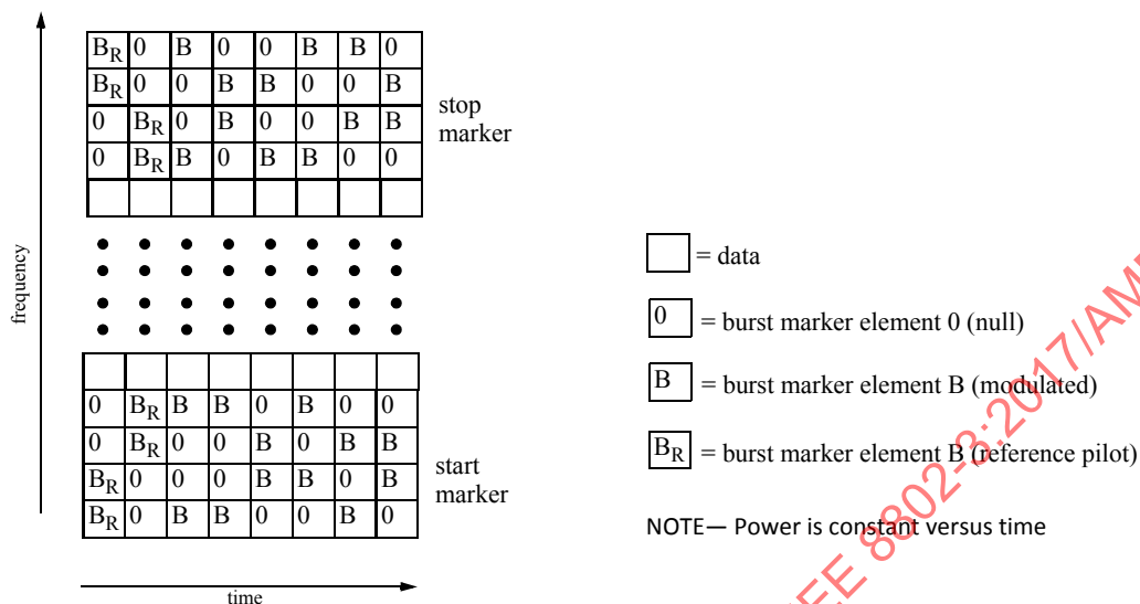
Figure 101-35—Burst marker in 8 symbol Resource Block
