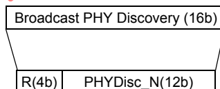
Figure 102–13—Broadcast PHY Discovery type Probe Control field
