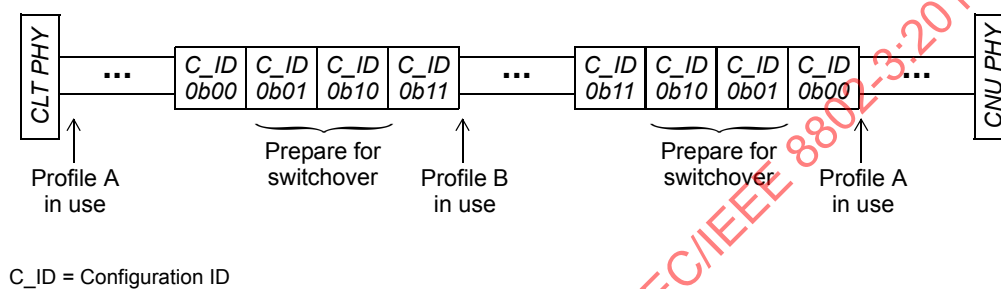
Figure 102–10—Configuration ID bit usage
