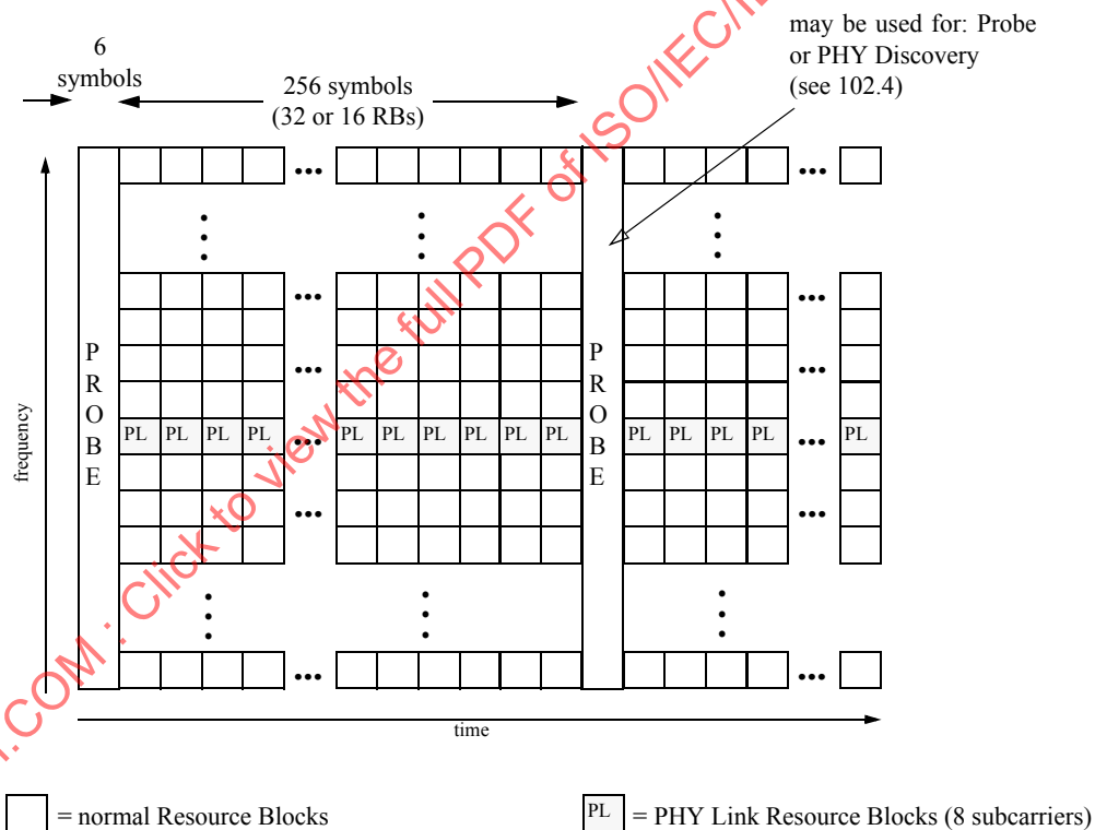
Figure 101–30—Upstream superframe structure
