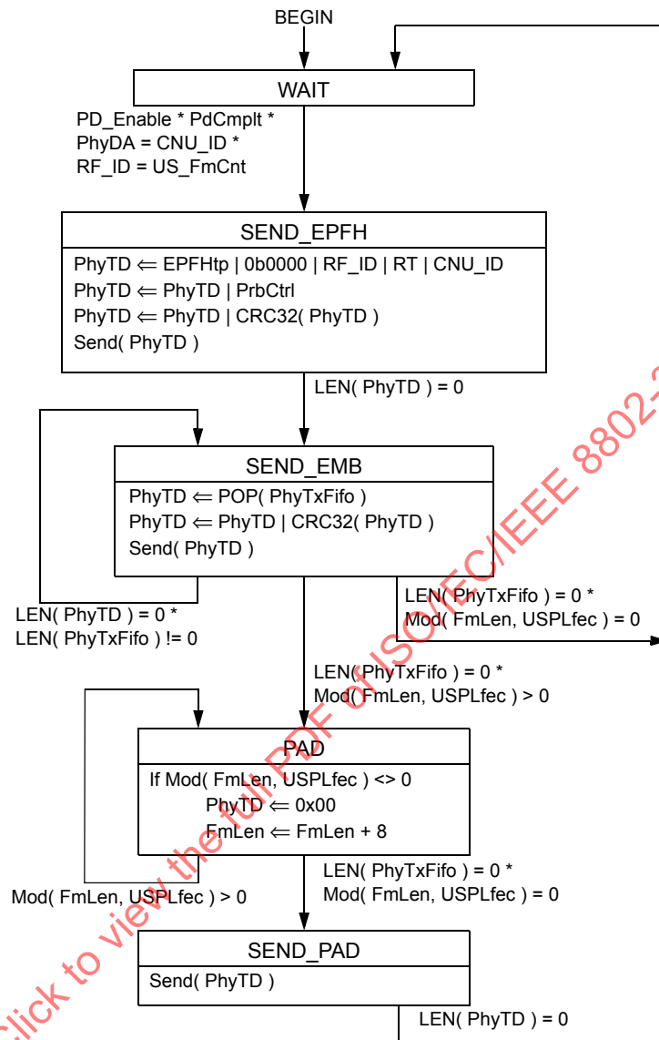
Figure 102-17—CNU PHY Link transmission control state diagram
