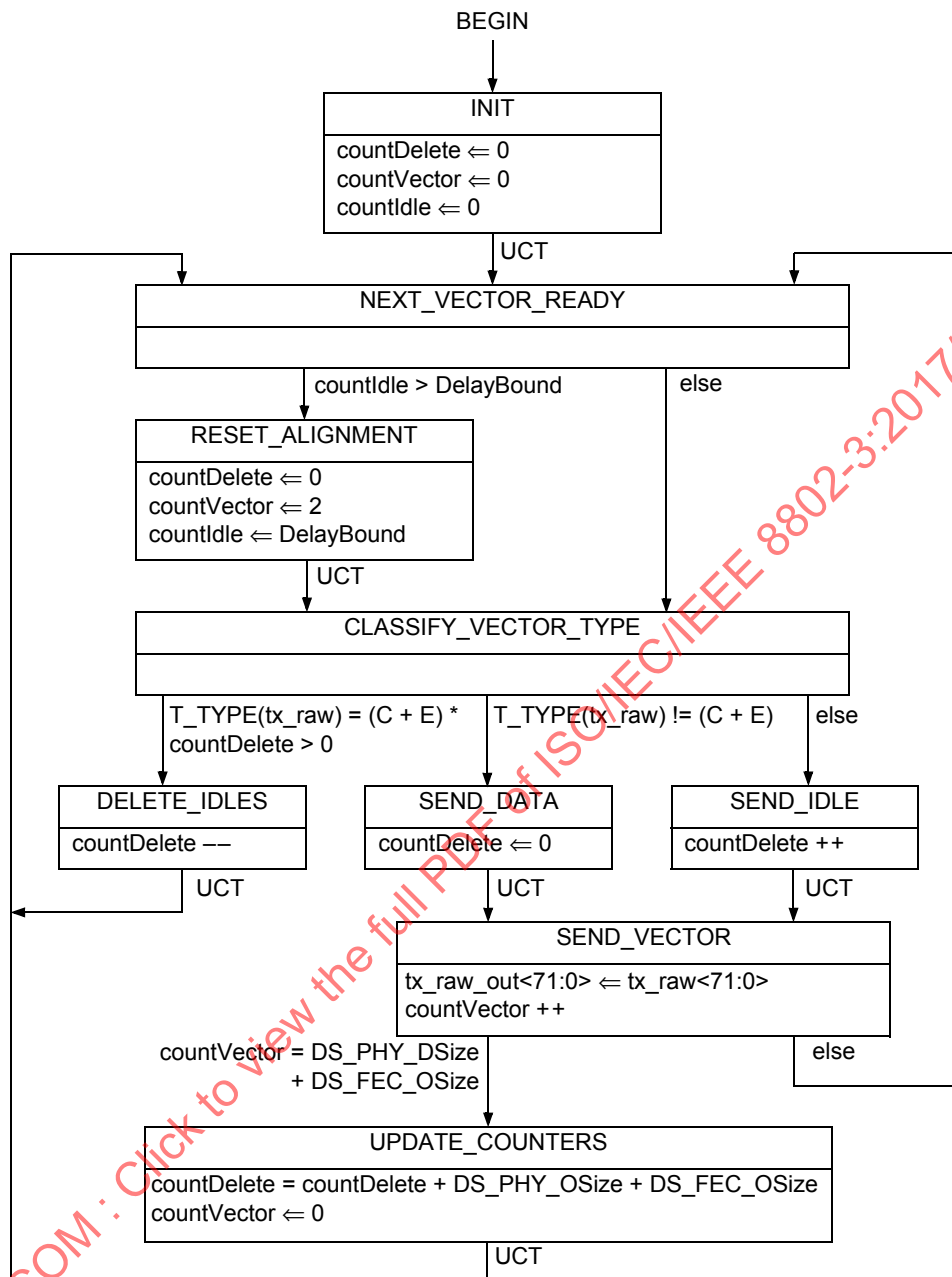
Figure 101-7—CNU Idle deletion process state diagram
