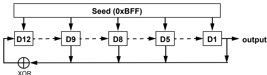
Figure 102-27—Probe sequence generator
