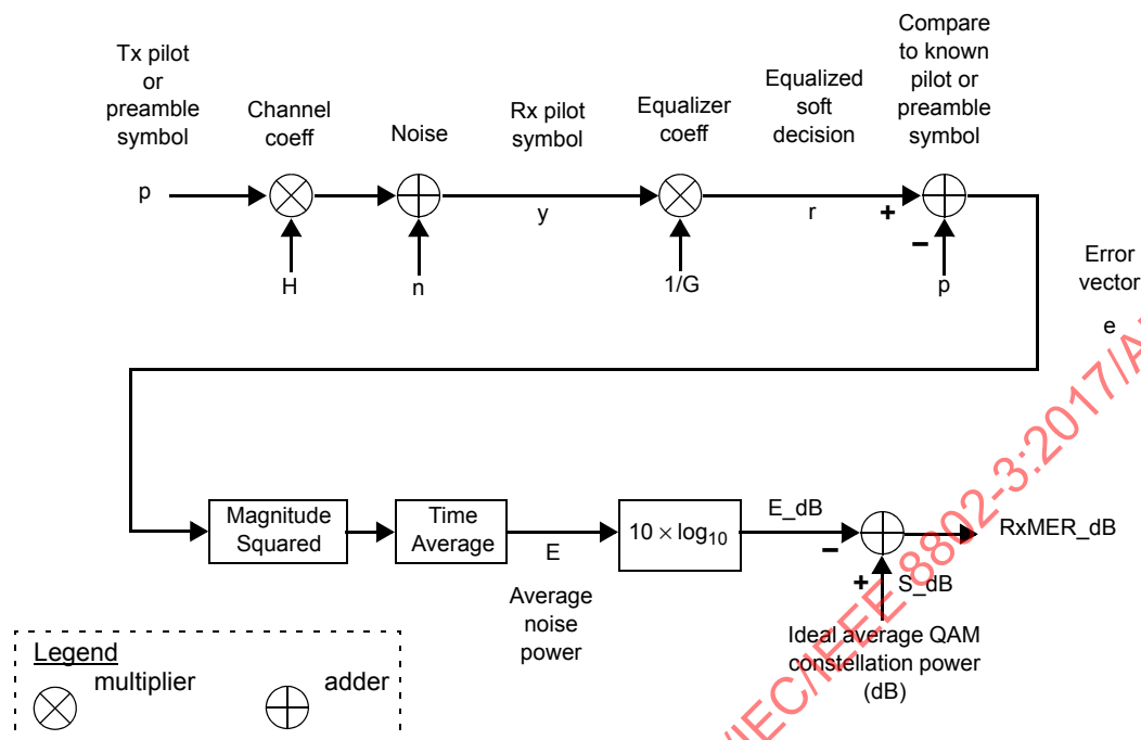
Figure 100-4—Computation of received modulation error ratio (RxMER) for a given subcarrier
