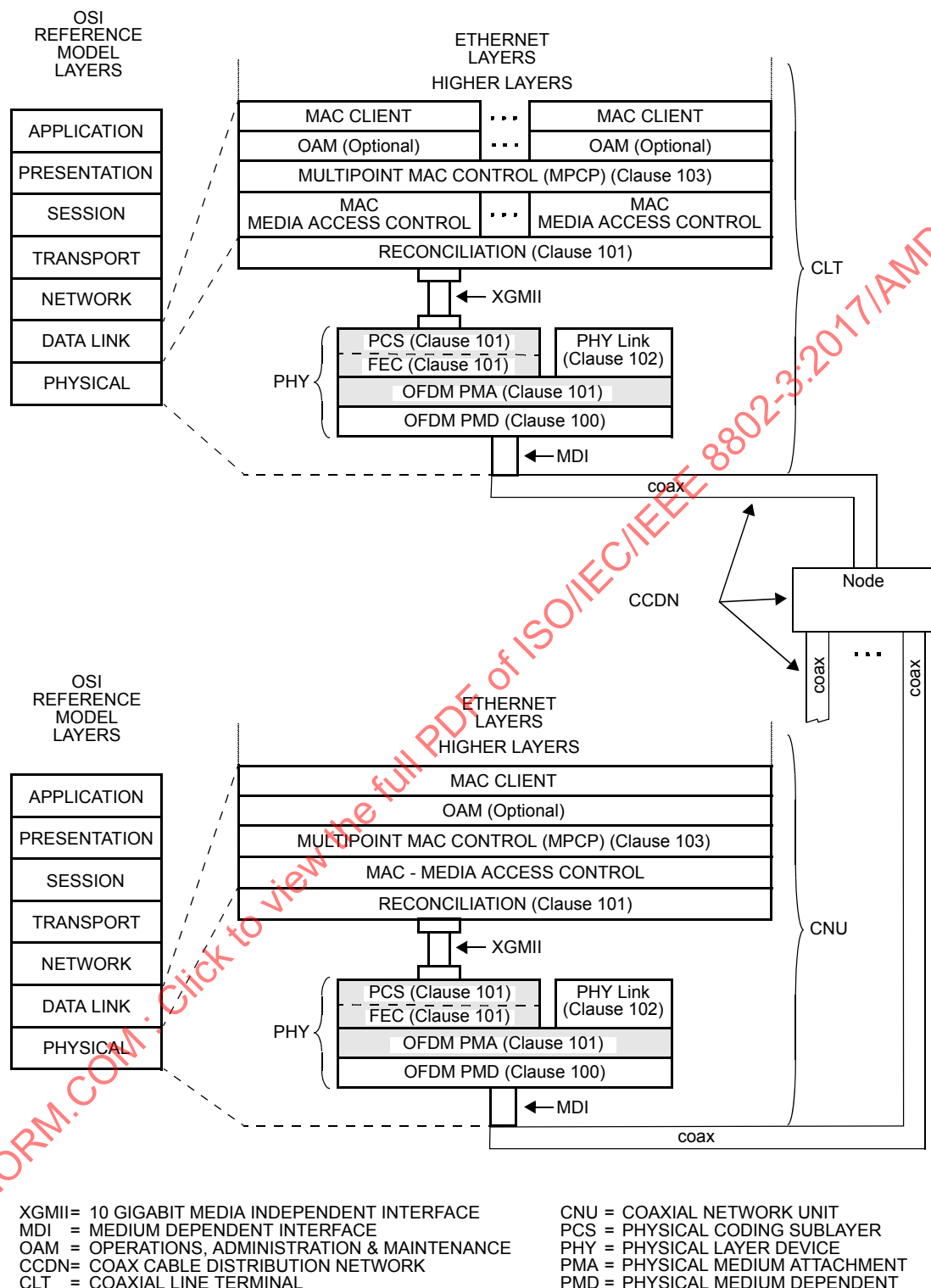
Figure 101-5—Relationship of EPoC PCS and PMA to the ISO/IEC OSI reference model and the IEEE 802.3 Ethernet LAN model
