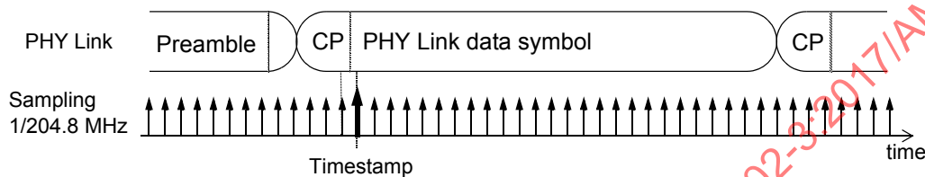
Figure 102–11—PHY Link Timestamp reference point
