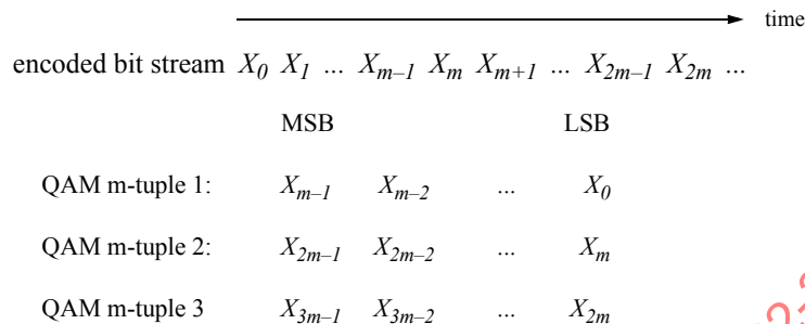
Figure 101–39—Bitstream to QAM m-tuple mapping
