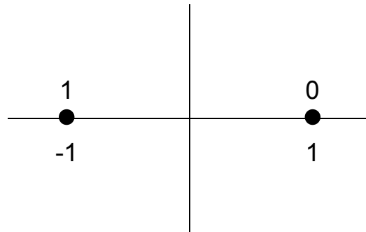
Figure 101-40—BPSK
