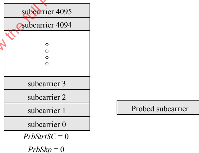
Figure 102–24—Example, all subcarriers used for probing, no skipping
