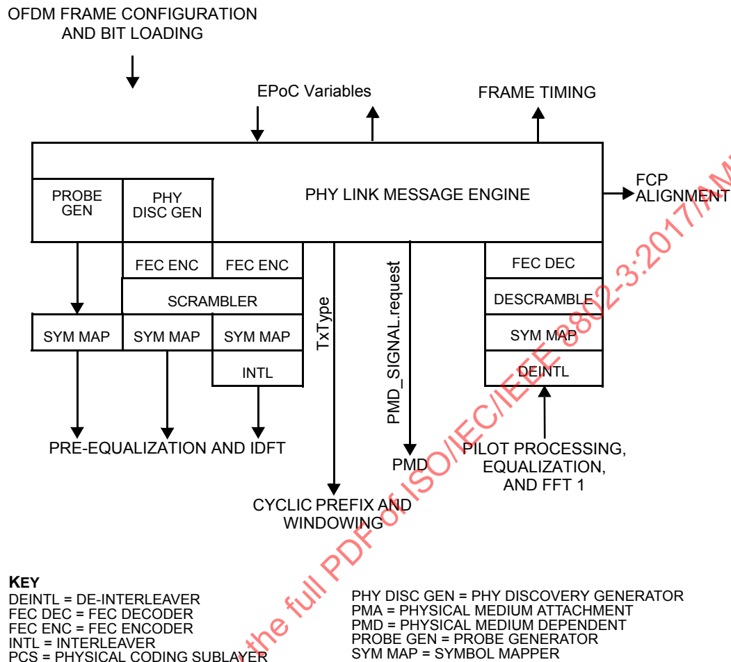
Figure 102-4—PHY Link CNU architecture
