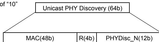
Figure 102–14—Unicast PHY Discovery type Probe Control field
