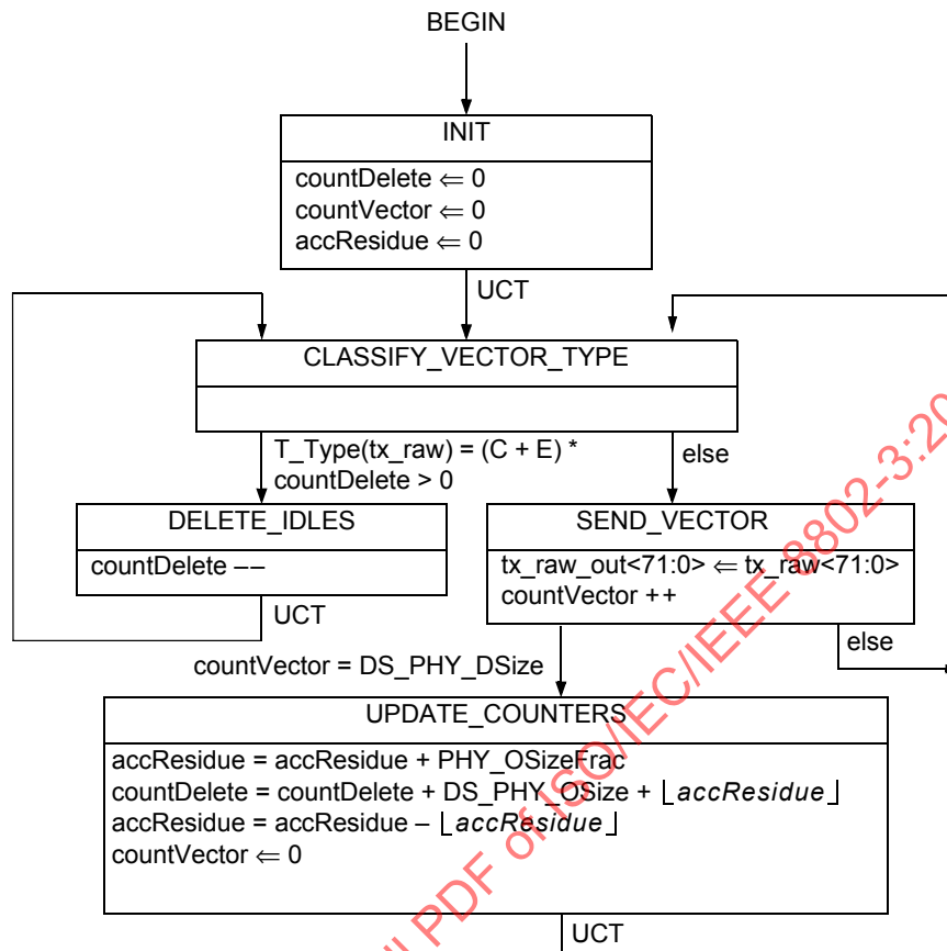
Figure 101-6—CLT Idle deletion process state diagram
