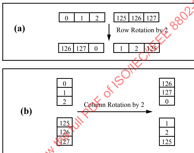
Figure 101–23—Rotation of subcarriers: a) Horizontal rows, b) Vertical columns
