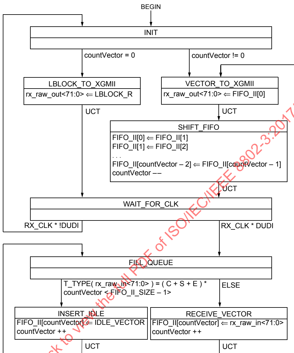
Figure 101-18—Idle control character insertion process state diagram
