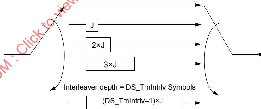
Figure 101–22—Time interleaver structure
