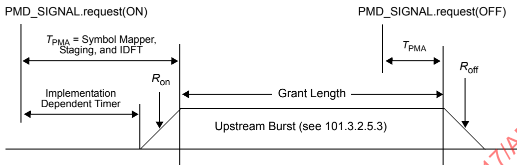
Figure 100-3—Details of RF power amplifier turn on and turn off timing
