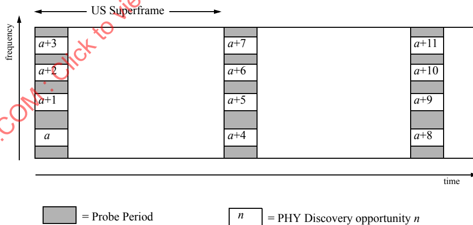
Figure 102–20—PHY Discovery opportunity numbering
