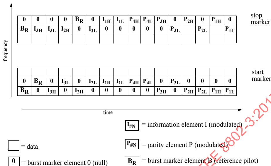
Figure 101-38—Burst marker encoding in 16 symbol Resource Block
