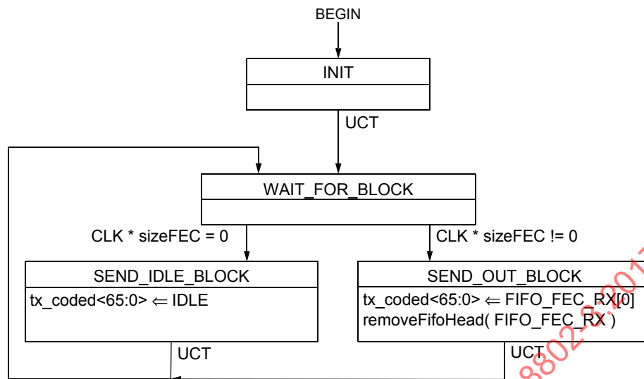
Figure 101-17—FEC Decoder, output process state diagram (CNU)
