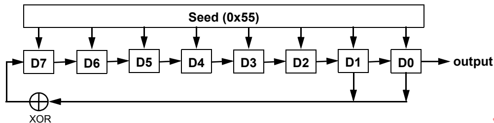
Figure 102-22—PHY Discovery Preamble generator
