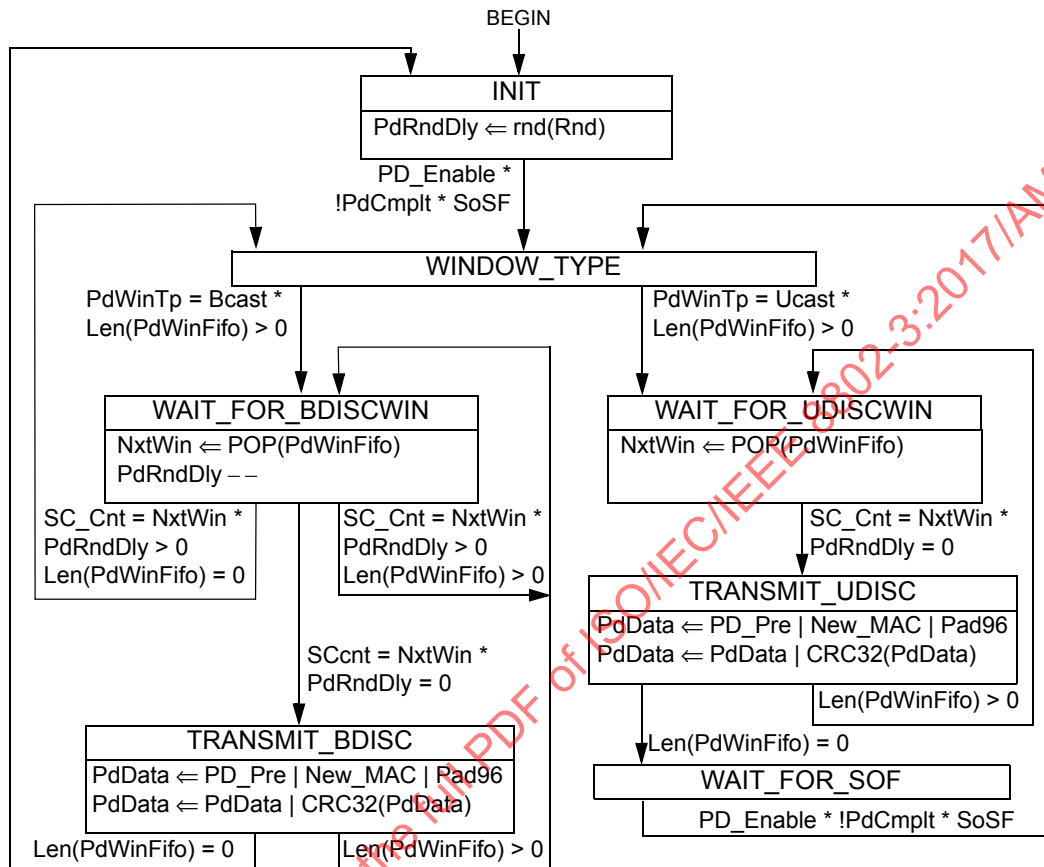
Figure 102–23—CNU PHY Discovery Response transmission control state diagram
