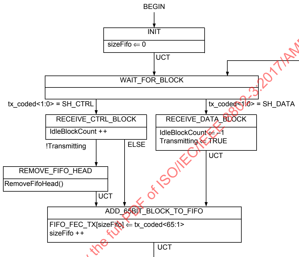
Figure 101–11— FEC Encoder and Data Detector input process state diagram
