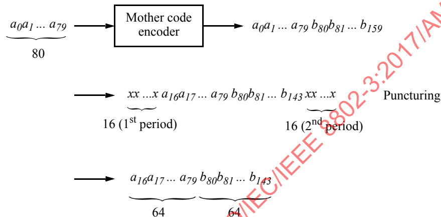
Figure 102–6—Puncturing encoder for the LDPC (128, 80) FEC
