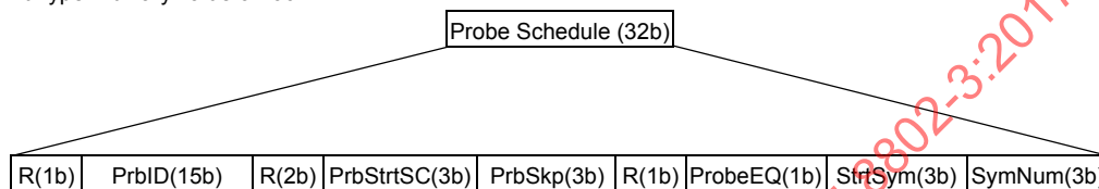
Figure 102–12—Probe Scheduling type Probe Control field
