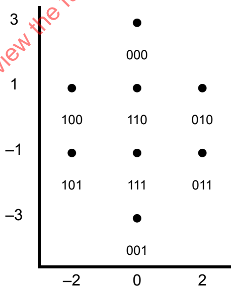
Figure 101-42—8-QAM
