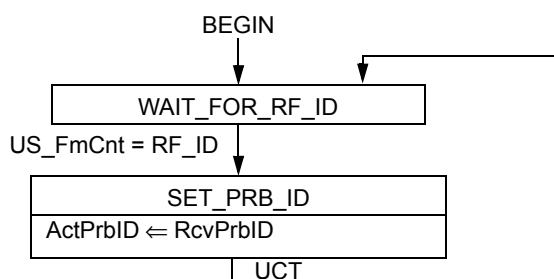
Figure 102–29—PrbID update state diagram
