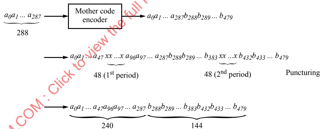
Figure 102–5—Puncturing encoder for LDPC (384,288) FEC
