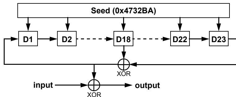
Figure 101-21—Scrambler
