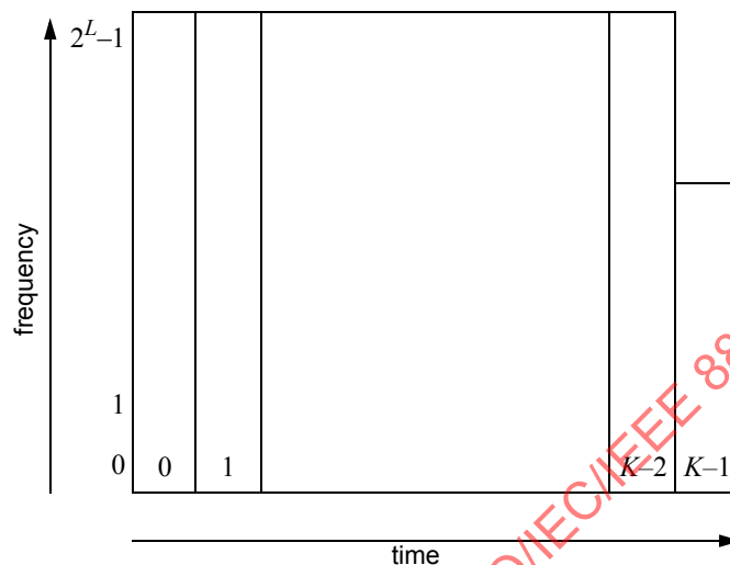
Figure 101–24—Two-dimensional store block structure
