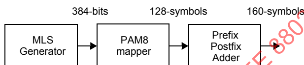
Figure 115-8—Pilot S 2 sub-block generator
