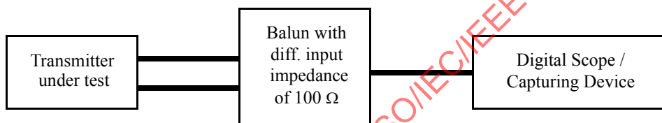
Figure 97-32—Transmitter test fixture 4 for MDI jitter measurement
