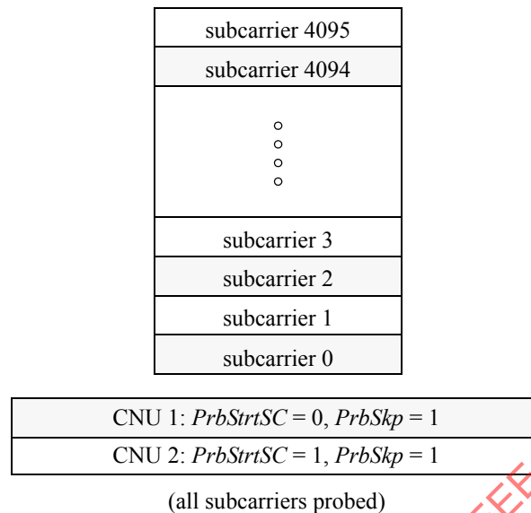
Figure 102–26—Scheduling two CNUs in the same probing symbol
