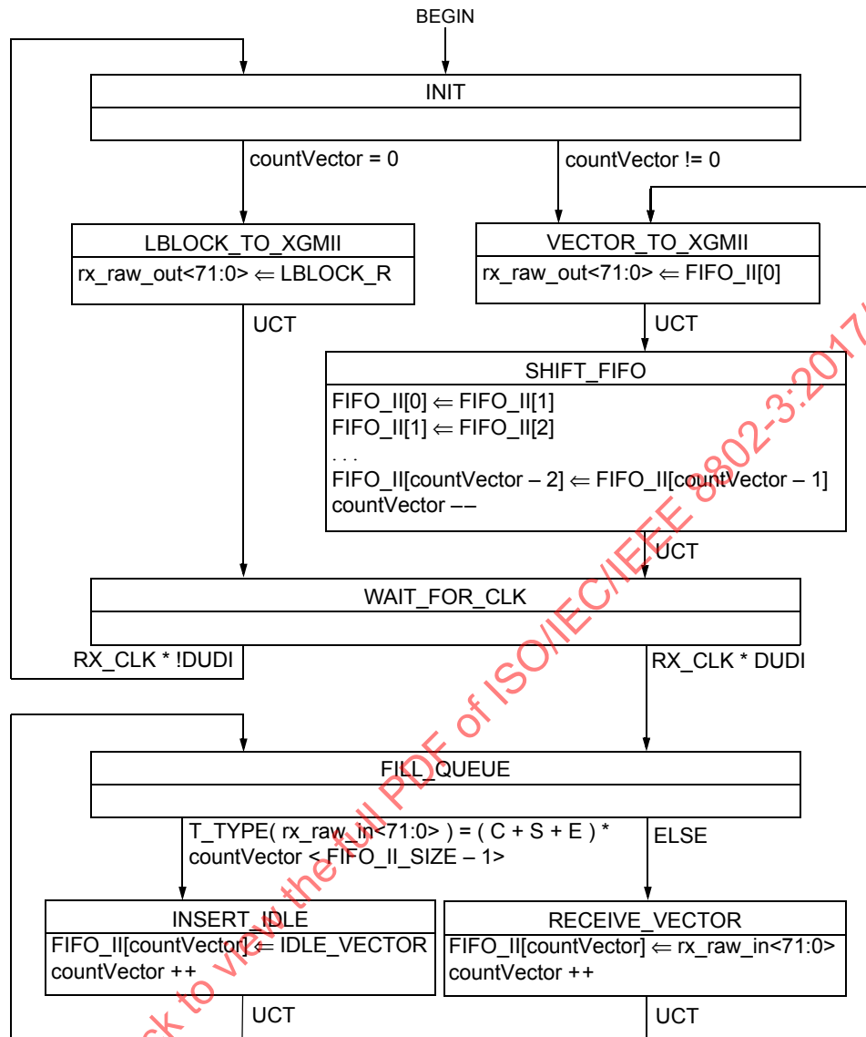
Figure 101-18—Idle control character insertion process state diagram
