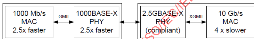
Figure 127A–1—2.5X speed 1000BASE-X to 2.5GBASE-X Link
