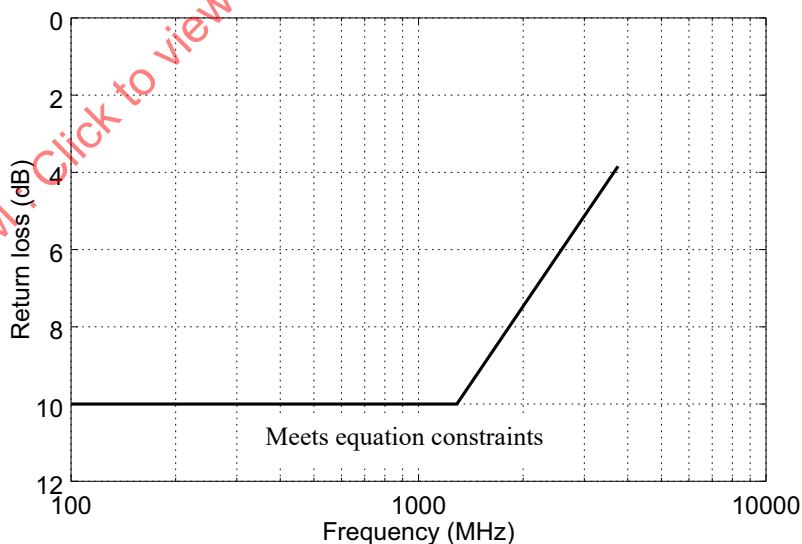
Figure 130-4—Transmit output differential-mode return loss limit
