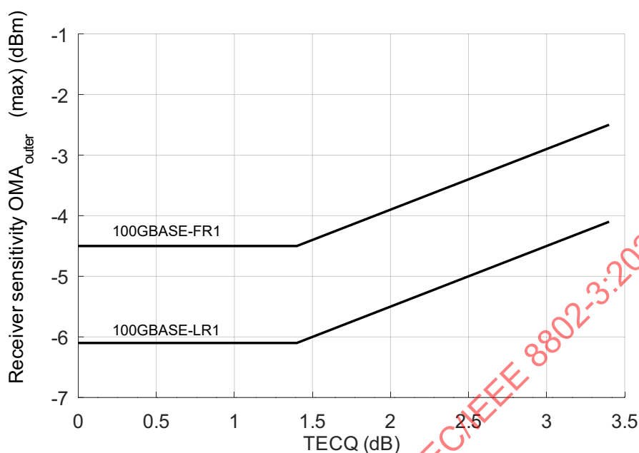
Figure 140-2b—Receiver sensitivity ( OMA_{outer} ) (max) for 100GBASE-FR1 and 100GBASE-LR1
