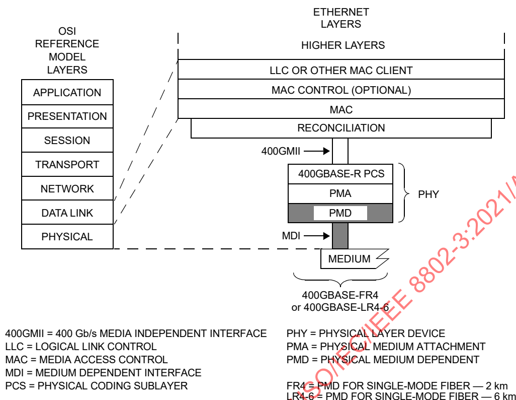
Figure 151–1—400GBASE-FR4 and 400GBASE-LR4-6 PMDs relationship to the ISO/IEC Open Systems Interconnection (OSI) reference model and IEEE 802.3 Ethernet model
