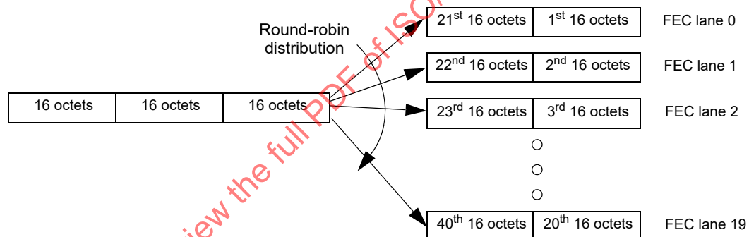
Figure 153-6—Lane distribution
