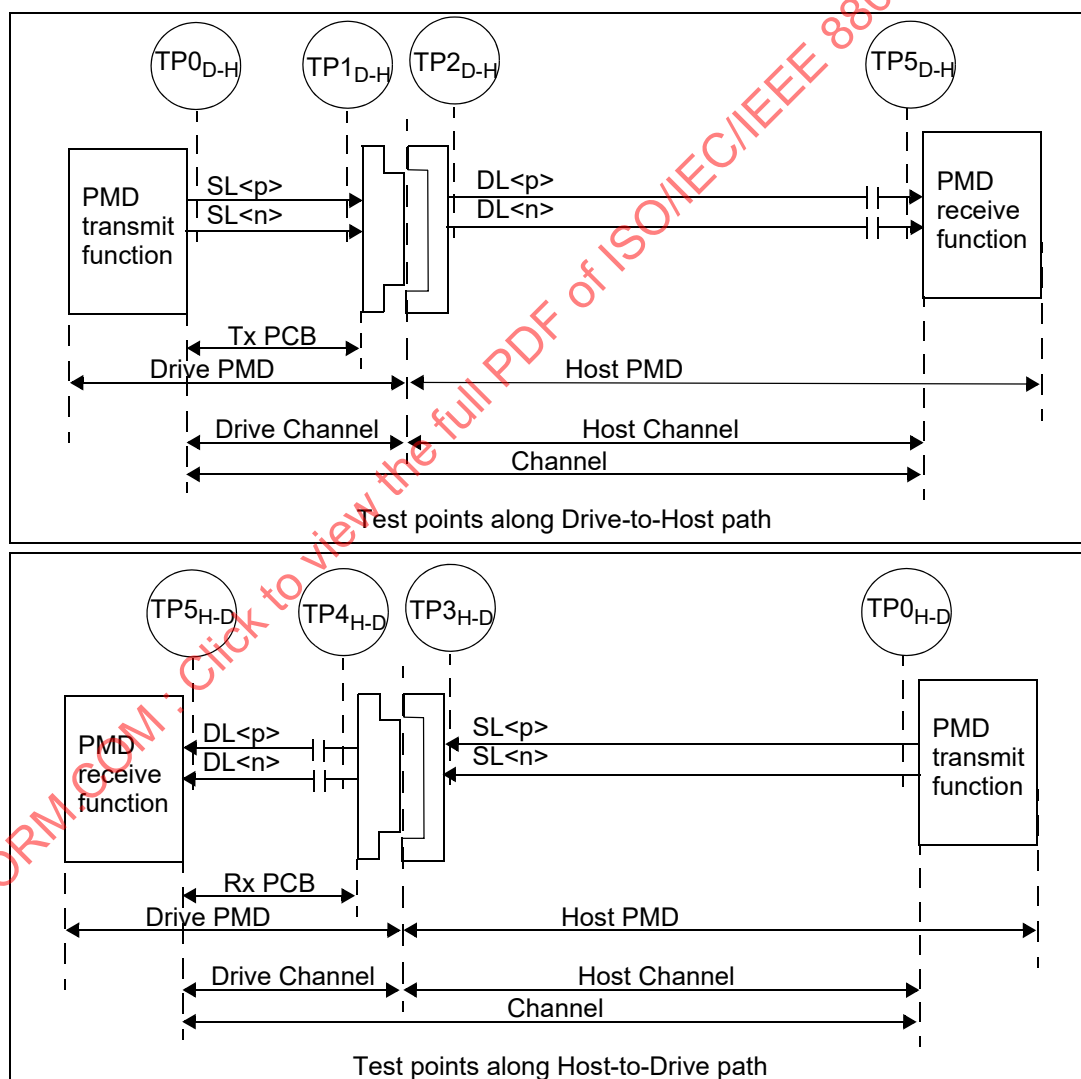
Figure 128A-1—Test points
