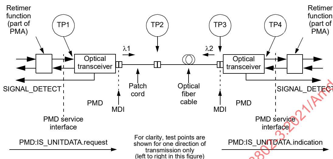
Figure 158-2—Block diagram for 10GBASE-BRx transmit/receive paths
