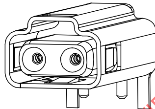
Figure 146-33—IEC 63171-6 jack
