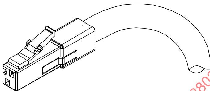
Figure 146–29—IEC 63171-1 plug
