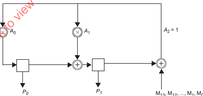
Figure 149–23—OAM FEC parity vector model
