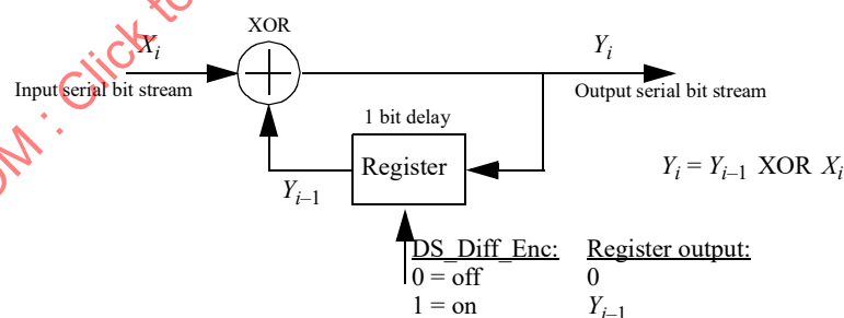
Figure 142–18—Differential encoding
