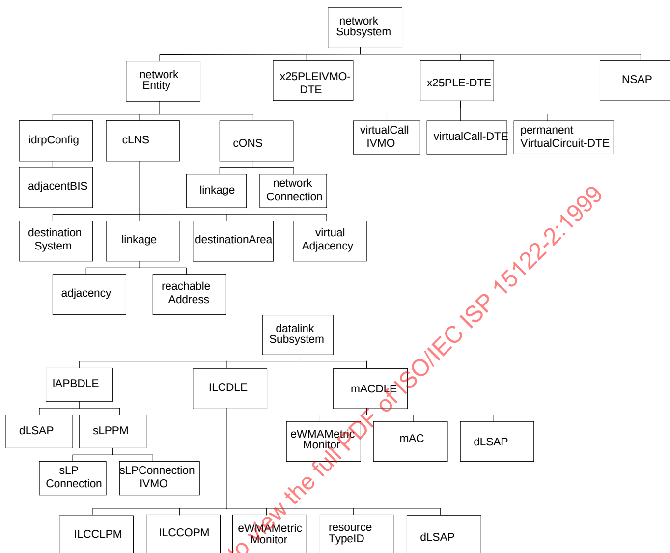
Figure 4 — Management Information Model for RB51.11x1 and RC51.11x1 Profiles
