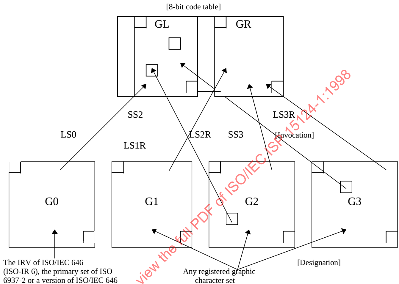
Figure 4 - Code extension features (all possible cases)
