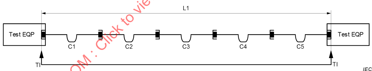
Figure 9 – Five-segments, six-connections, E2E link
